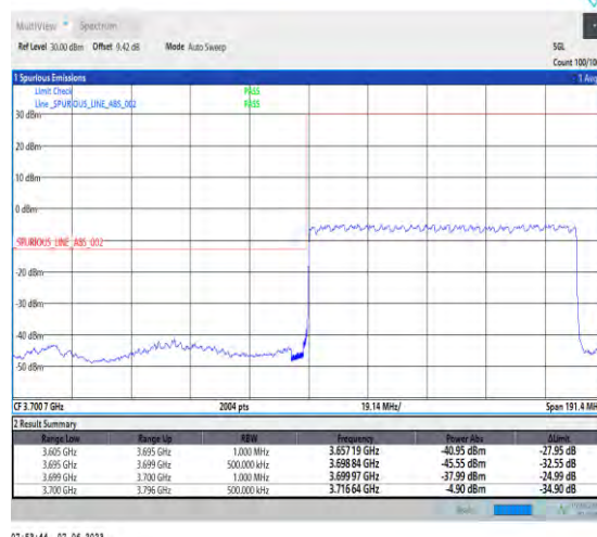
1-N78-3700-3800-PC3-30-90-L-3-DFT-PI2BPSK-Outer_Full-240@0-Ant1-1--PASS-see graph
