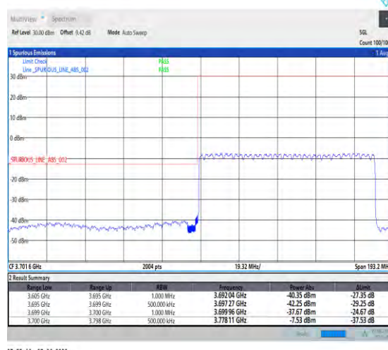
1-N78-3700-3800-PC3-30-90-L-6-CP-QPSK-Outer_Full-245@0-Ant1-1--PASS-see graph
