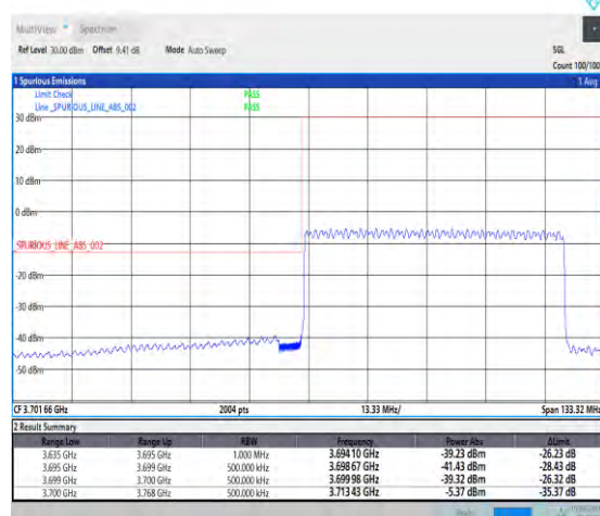
1-N78-3700-3800-PC3-30-60-L-6-CP-QPSK-Outer_Full-162@0-Ant1-1--PASS-see graph
