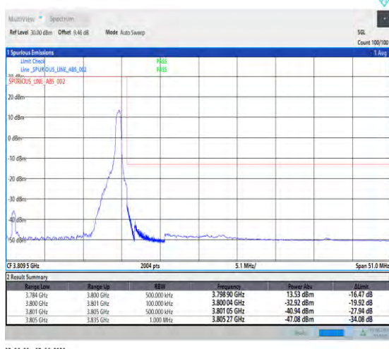
1-N78-3700-3800-PC3-30-30-H-5-CP-QPSK-Edge_1RB_Right-1@77-Ant1-1--PASS-see graph
