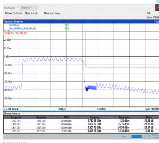
1-N78-3700-3800-PC3-30-30-H-6-CP-QPSK-Outer_Full-78@0-Ant1-1--PASS-see graph
