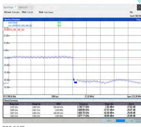
1-N78-3700-3800-PC3-30-100-H-6-CP-QPSK-Outer_Full-273@0-Ant1-1--PASS-see graph
