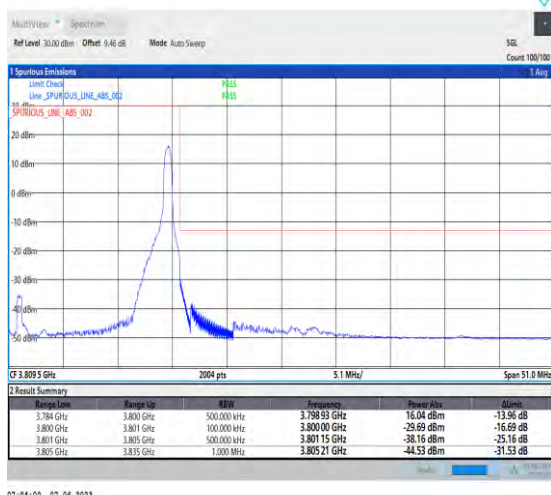
1-N78-3700-3800-PC3-30-30-H-2-DFT-PI2BPSK-Edge_1RB_Right-1@77-Ant1-1--PASS-see graph
