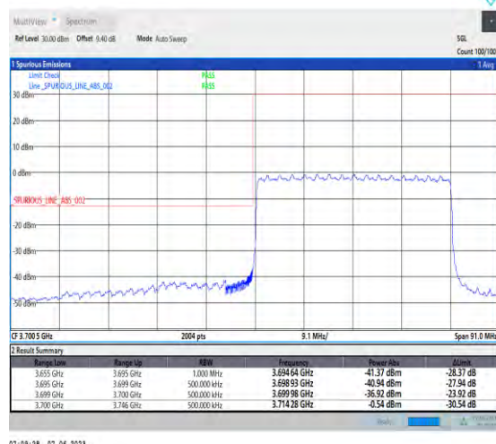
1-N78-3700-3800-PC3-30-40-L-3-DFT-PI2BPSK-Outer_Full-100@0-Ant1-1--PASS-see graph
