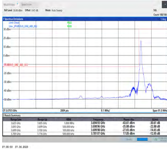
1-N78-3700-3800-PC3-30-70-L-1-DFT-PI2BPSK-Edge_1RB_Left-1@0-Ant1-1--PASS-see graph
