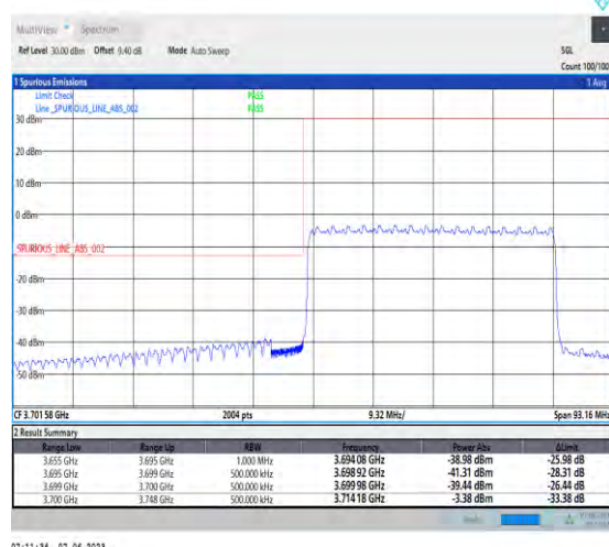
1-N78-3700-3800-PC3-30-40-L-6-CP-QPSK-Outer_Full-106@0-Ant1-1--PASS-see graph
