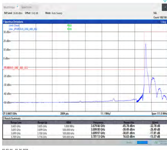
1-N78-3700-3800-PC3-30-90-L-1-DFT-PI2BPSK-Edge_1RB_Left-1@0-Ant1-1--PASS-see graph
