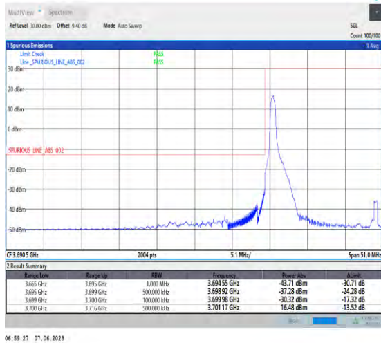
1-N78-3700-3800-PC3-30-30-L-1-DFT-PI2BPSK-Edge_1RB_Left-1@0-Ant1-1--PASS-see graph
