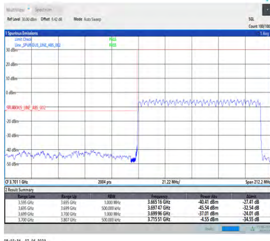
1-N78-3700-3800-PC3-30-100-L-3-DFT-PI2BPSK-Outer_Full-270@0-Ant1-1--PASS-see graph
