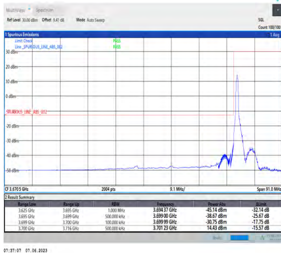
1-N78-3700-3800-PC3-30-70-L-4-CP-QPSK-Edge_1RB_Left-1@0-Ant1-1--PASS-see graph
