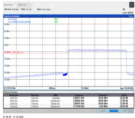
1-N78-3700-3800-PC3-30-70-L-6-CP-QPSK-Outer_Full-189@0-Ant1-1--PASS-see graph
