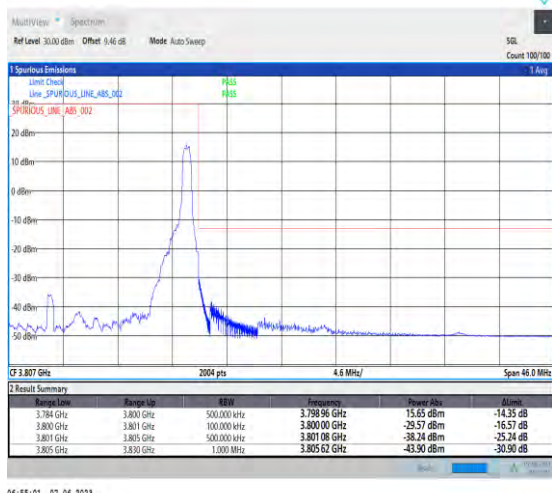
1-N78-3700-3800-PC3-30-25-H-2-DFT-PI2BPSK-Edge_1RB_Right-1@64-Ant1-1--PASS-see graph
