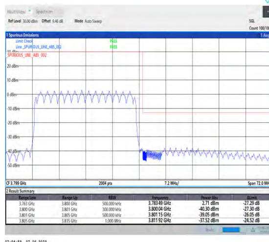
1-N78-3700-3800-PC3-30-30-H-3-DFT-PI2BPSK-Outer_Full-75@0-Ant1-1--PASS-see graph
