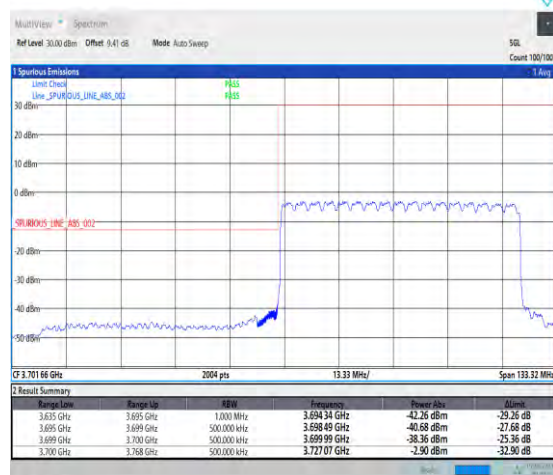
1-N78-3700-3800-PC3-30-60-L-3-DFT-PI2BPSK-Outer_Full-162@0-Ant1-1--PASS-see graph
