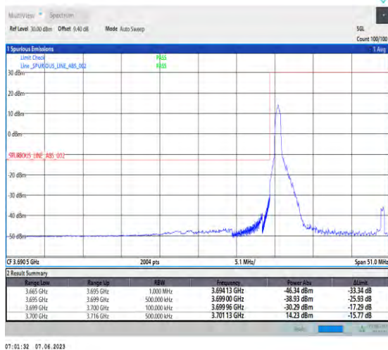
1-N78-3700-3800-PC3-30-30-L-4-CP-QPSK-Edge_1RB_Left-1@0-Ant1-1--PASS-see graph
