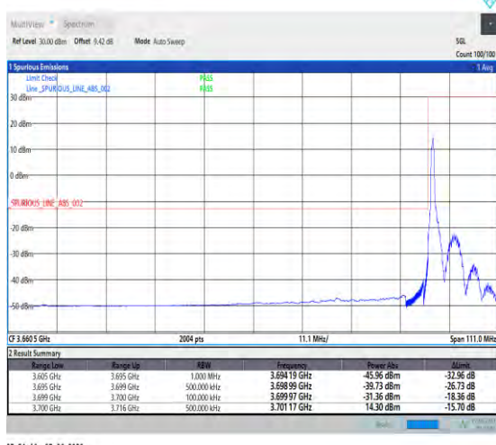
1-N78-3700-3800-PC3-30-90-L-4-CP-QPSK-Edge_1RB_Left-1@0-Ant1-1--PASS-see graph
