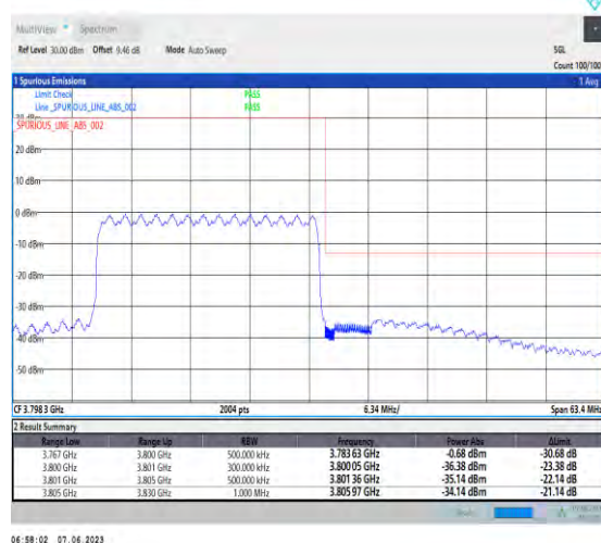
1-N78-3700-3800-PC3-30-25-H-6-CP-QPSK-Outer_Full-65@0-Ant1-1--PASS-see graph
