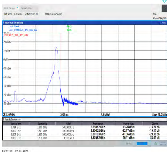
1-N78-3700-3800-PC3-30-25-H-5-CP-QPSK-Edge_1RB_Right-1@64-Ant1-1--PASS-see graph
