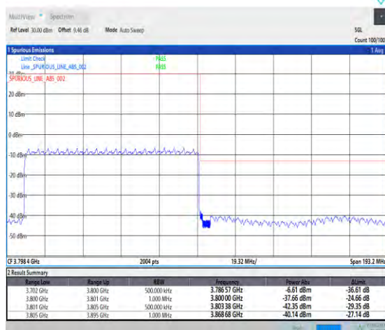
1-N78-3700-3800-PC3-30-90-H-6-CP-QPSK-Outer_Full-245@0-Ant1-1--PASS-see graph
