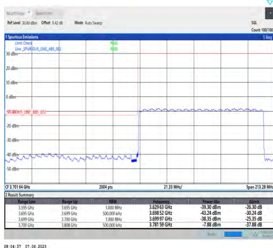
1-N78-3700-3800-PC3-30-100-L-6-CP-QPSK-Outer_Full-273@0-Ant1-1--PASS-see graph
