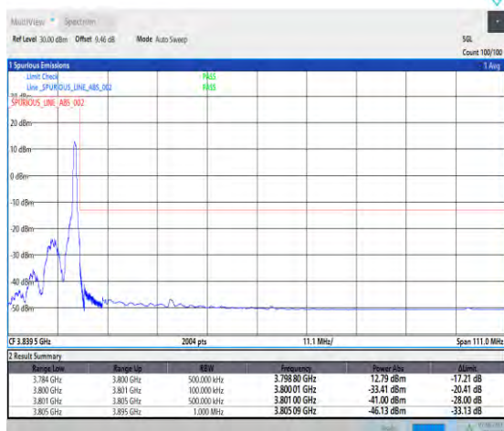
1-N78-3700-3800-PC3-30-90-H-5-CP-QPSK-Edge_1RB_Right-1@244-Ant1-1--PASS-see graph
