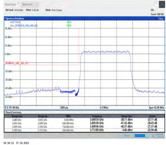
1-N78-3700-3800-PC3-30-15-L-3-DFT-PI2BPSK-Outer_Full-36@0-Ant1-1--PASS-see graph
