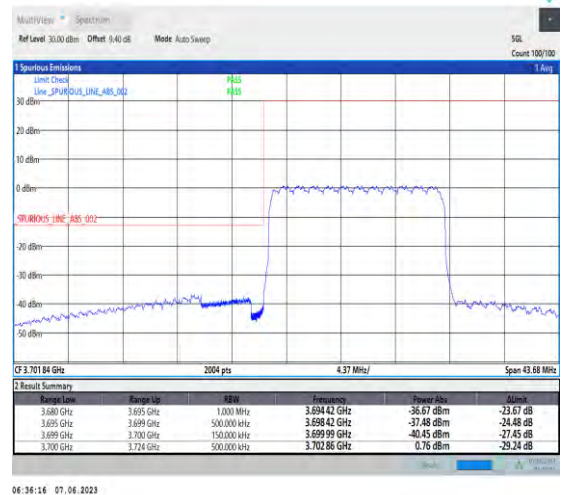
1-N78-3700-3800-PC3-30-15-L-6-CP-QPSK-Outer_Full-38@0-Ant1-1--PASS-see graph
