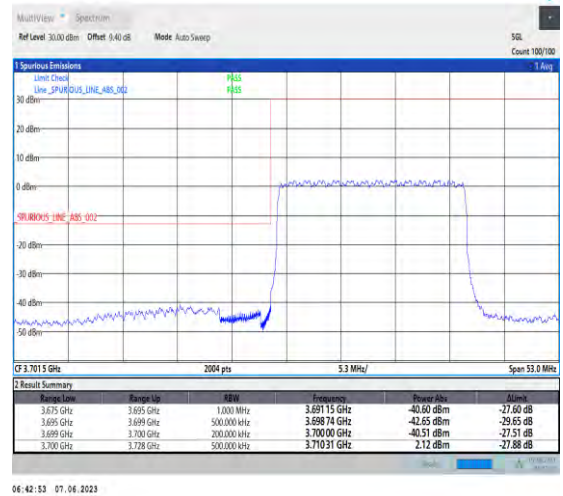
1-N78-3700-3800-PC3-30-20-L-3-DFT-PI2BPSK-Outer_Full-50@0-Ant1-1--PASS-see graph
