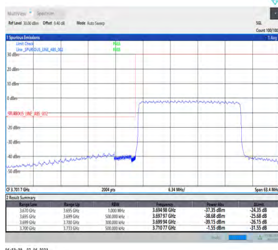
1-N78-3700-3800-PC3-30-25-L-6-CP-QPSK-Outer_Full-65@0-Ant1-1--PASS-see graph
