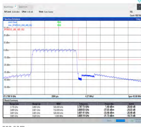
1-N78-3700-3800-PC3-30-15-H-6-CP-QPSK-Outer_Full-38@0-Ant1-1--PASS-see graph
