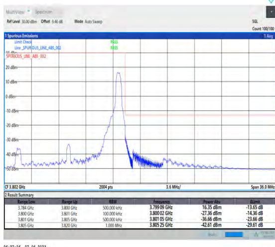
1-N78-3700-3800-PC3-30-15-H-2-DFT-PI2BPSK-Edge_1RB_Right-1@37-Ant1-1--PASS-see graph
