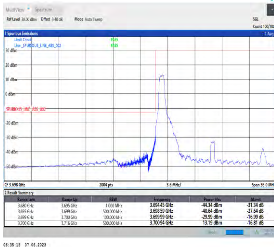
1-N78-3700-3800-PC3-30-15-L-4-CP-QPSK-Edge_1RB_Left-1@0-Ant1-1--PASS-see graph
