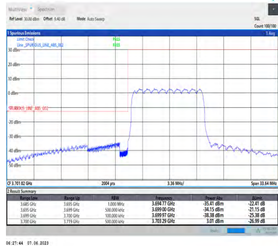
1-N78-3700-3800-PC3-30-10-L-6-CP-QPSK-Outer_Full-24@0-Ant1-1--PASS-see graph
