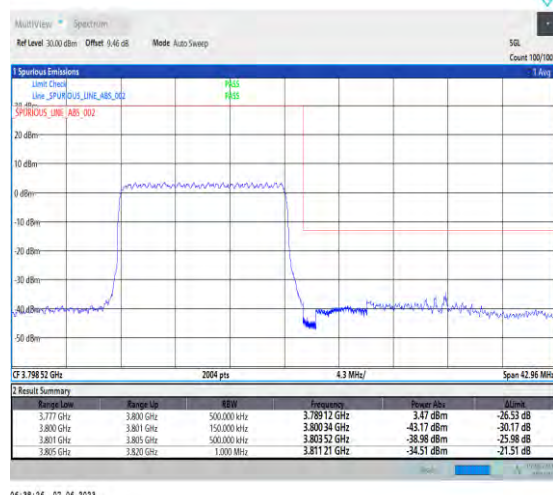
1-N78-3700-3800-PC3-30-15-H-3-DFT-PI2BPSK-Outer_Full-36@0-Ant1-1--PASS-see graph
