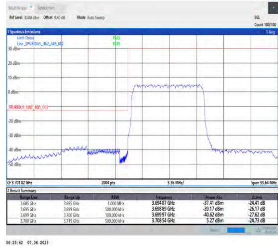
1-N78-3700-3800-PC3-30-10-L-3-DFT-PI2BPSK-Outer_Full-24@0-Ant1-1--PASS-see graph
