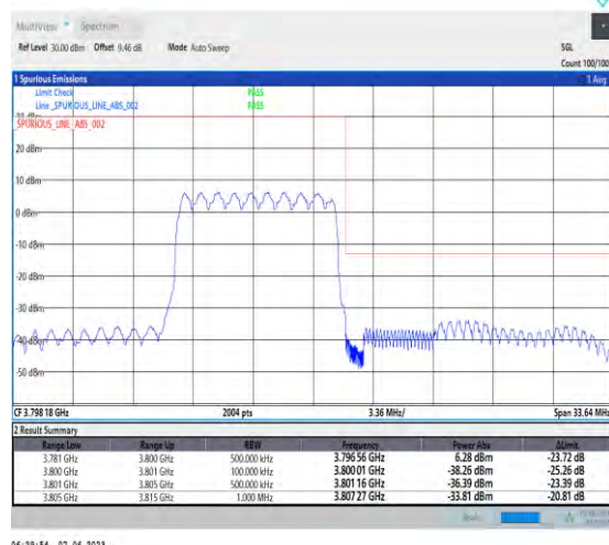
1-N78-3700-3800-PC3-30-10-H-3-DFT-PI2BPSK-Outer_Full-24@0-Ant1-1--PASS-see graph
