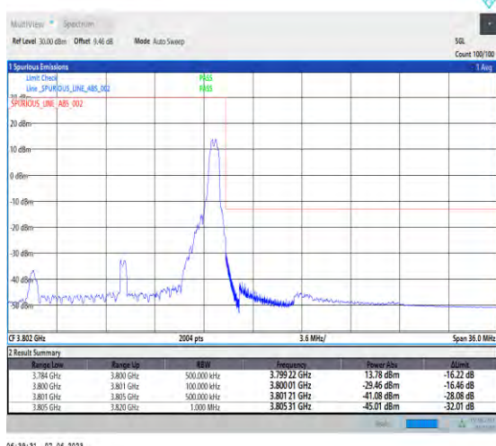
1-N78-3700-3800-PC3-30-15-H-5-CP-QPSK-Edge_1RB_Right-1@37-Ant1-1--PASS-see graph
