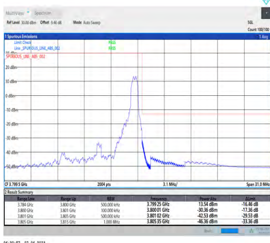
1-N78-3700-3800-PC3-30-10-H-5-CP-QPSK-Edge_1RB_Right-1@23-Ant1-1--PASS-see graph
