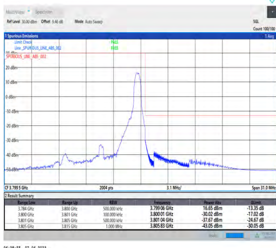
1-N78-3700-3800-PC3-30-10-H-2-DFT-PI2BPSK-Edge_1RB_Right-1@23-Ant1-1--PASS-see graph
