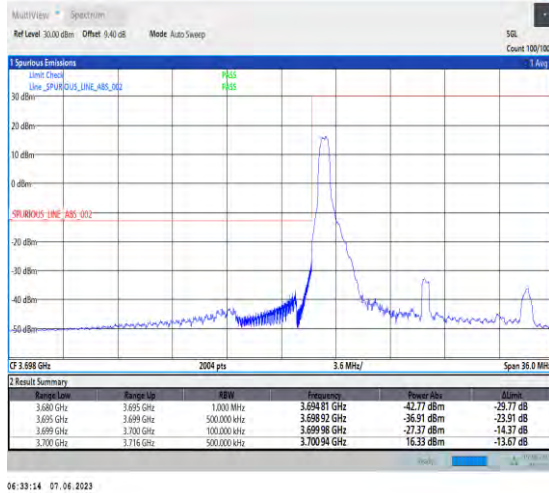
1-N78-3700-3800-PC3-30-15-L-1-DFT-PI2BPSK-Edge_1RB_Left-1@0-Ant1-1--PASS-see graph
