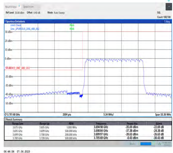
1-N78-3700-3800-PC3-30-20-L-6-CP-QPSK-Outer_Full-51@0-Ant1-1--PASS-see graph
