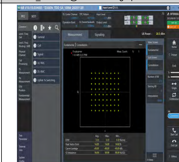
1-N78-3700-3800-PC3-30-100-M-8-CP-64QAM-Outer_Full-273@0-Ant1-see graph-PASS
