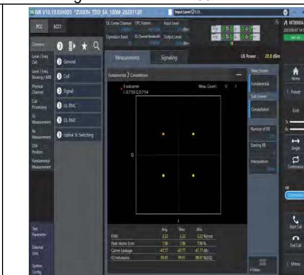
1-N78-3700-3800-PC3-30-100-M-6-CP-QPSK-Outer_Full-273@0-Ant1-see graph-PASS
