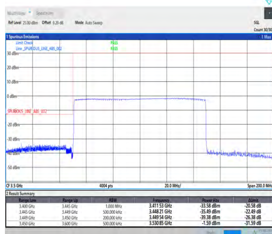
1-N78-3450-3550-PC3-30-100-L-6-CP-QPSK-Outer_Full-273@0-Ant1-1--PASS-see graph
