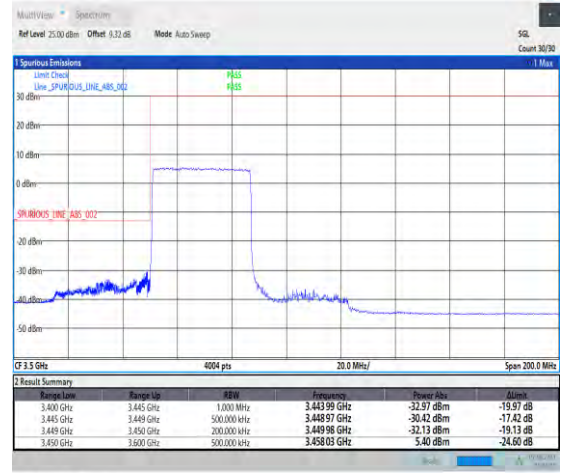
1-N78-3450-3550-PC3-30-40-L-3-DFT-PI2BPSK-Outer_Full-100@0-Ant1-1--PASS-see graph
