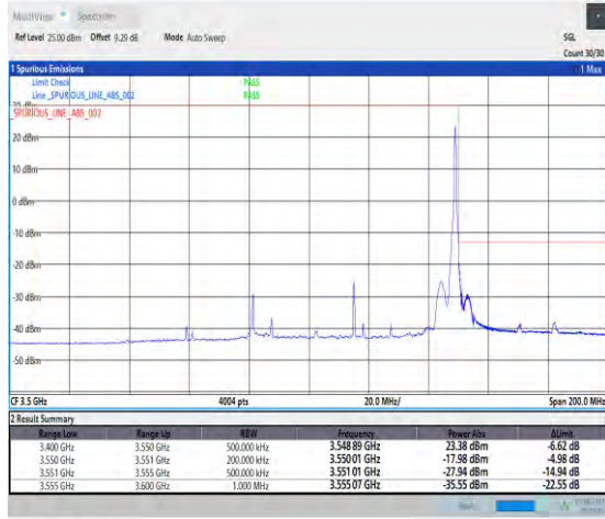
1-N78-3450-3550-PC3-30-70-H-2-DFT-PI2BPSK-Edge_1RB_Right-1@188-Ant1-1--PASS-see graph
