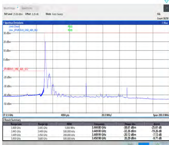
1-N78-3450-3550-PC3-30-100-L-4-CP-QPSK-Edge_1RB_Left-1@0-Ant1-1--PASS-see graph
