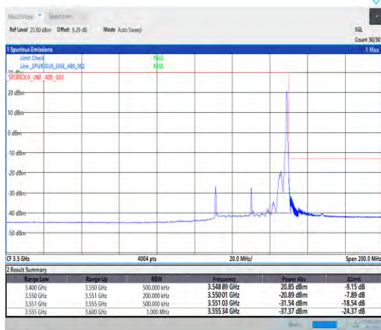
1-N78-3450-3550-PC3-30-40-H-5-CP-QPSK-Edge_1RB_Right-1@105-Ant1-1--PASS-see graph
