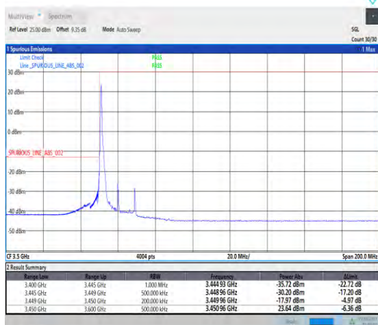
1-N78-3450-3550-PC3-30-20-L-1-DFT-PI2BPSK-Edge_1RB_Left-1@0-Ant1-1--PASS-see graph
