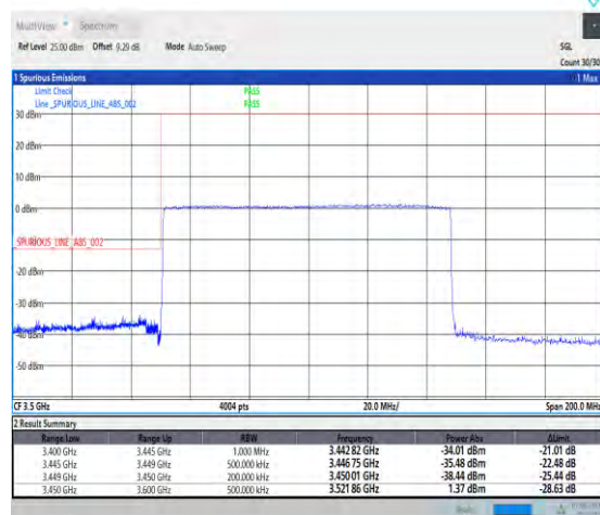
1-N78-3450-3550-PC3-30-100-L-3-DFT-PI2BPSK-Outer_Full-270@0-Ant1-1--PASS-see graph
