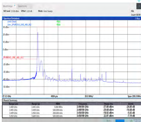
1-N78-3450-3550-PC3-30-100-L-1-DFT-PI2BPSK-Edge_1RB_Left-1@0-Ant1-1--PASS-see graph
