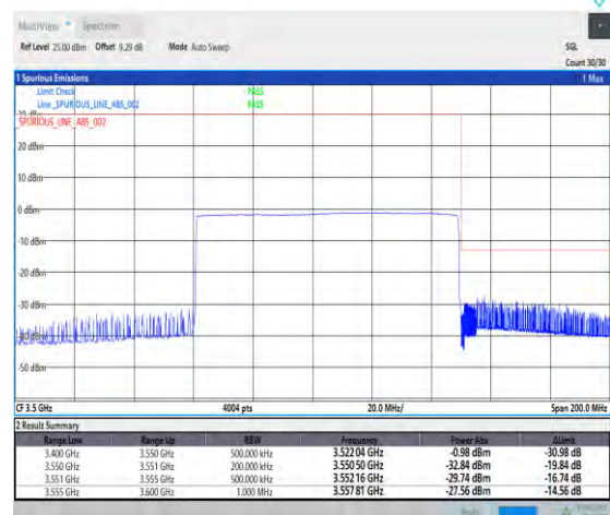
1-N78-3450-3550-PC3-30-90-H-6-CP-QPSK-Outer_Full-245@0-Ant1-1--PASS-see graph
