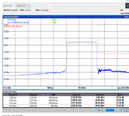
1-N78-3450-3550-PC3-30-50-H-3-DFT-PI2BPSK-Outer_Full-128@0-Ant1-1--PASS-see graph
