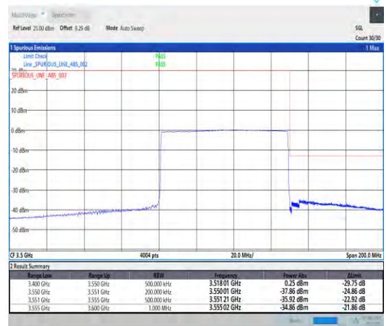
1-N78-3450-3550-PC3-30-70-H-6-CP-QPSK-Outer_Full-189@0-Ant1-1--PASS-see graph
