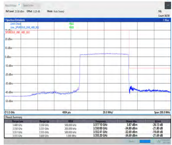
1-N78-3450-3550-PC3-30-60-H-3-DFT-PI2BPSK-Outer_Full-162@0-Ant1-1--PASS-see graph
