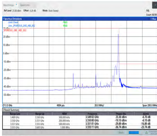
1-N78-3450-3550-PC3-30-60-H-2-DFT-PI2BPSK-Edge_1RB_Right-1@161-Ant1-1--PASS-see graph
