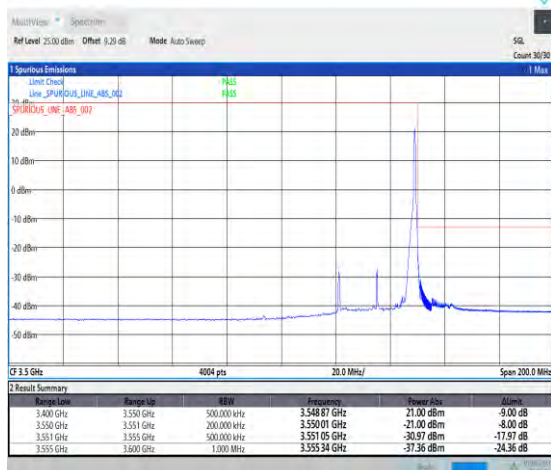
1-N78-3450-3550-PC3-30-30-H-5-CP-QPSK-Edge_1RB_Right-1@77-Ant1-1--PASS-see graph
