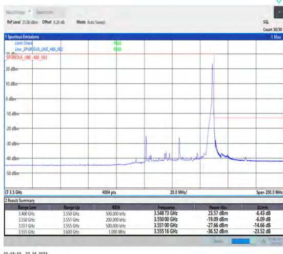
1-N78-3450-3550-PC3-30-50-H-2-DFT-PI2BPSK-Edge_1RB_Right-1@132-Ant1-1--PASS-see graph
