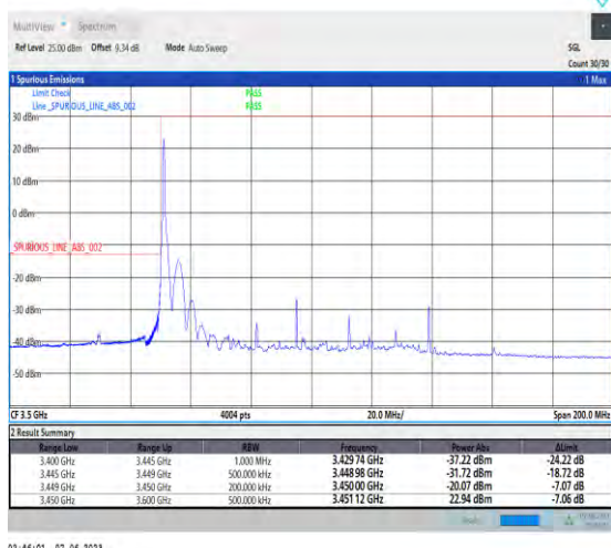
1-N78-3450-3550-PC3-30-90-L-1-DFT-PI2BPSK-Edge_1RB_Left-1@0-Ant1-1--PASS-see graph
