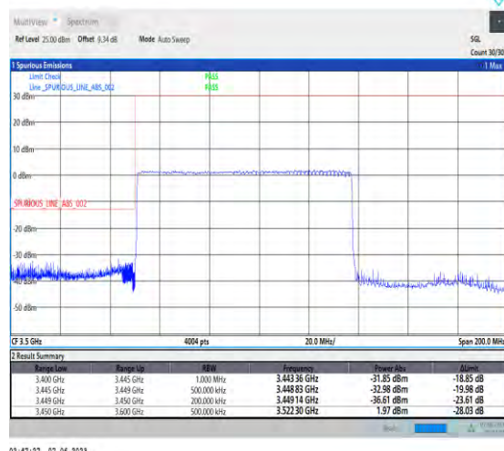
1-N78-3450-3550-PC3-30-90-L-3-DFT-PI2BPSK-Outer_Full-240@0-Ant1-1--PASS-see graph
