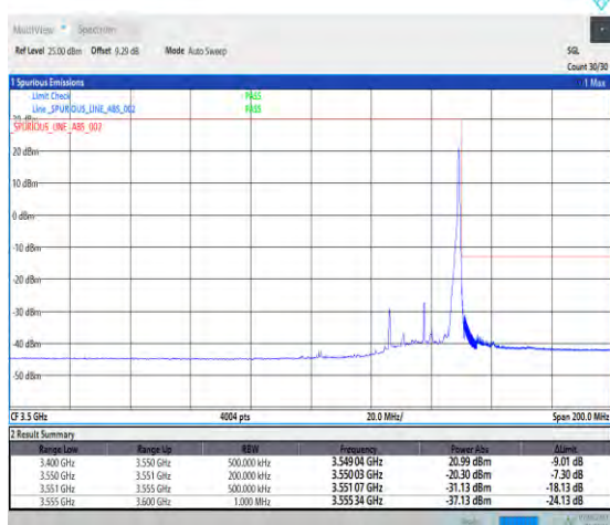
1-N78-3450-3550-PC3-30-25-H-5-CP-QPSK-Edge_1RB_Right-1@64-Ant1-1--PASS-see graph
