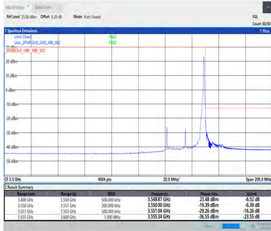
1-N78-3450-3550-PC3-30-30-H-2-DFT-PI2BPSK-Edge_1RB_Right-1@77-Ant1-1--PASS-see graph
