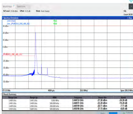
1-N78-3450-3550-PC3-30-20-L-4-CP-QPSK-Edge_1RB_Left-1@0-Ant1-1--PASS-see graph
