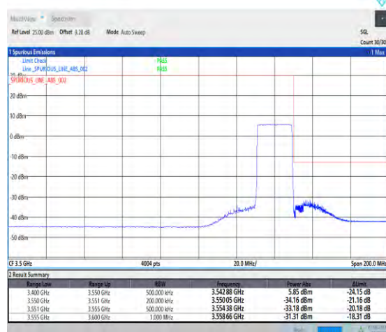
1-N78-3450-3550-PC3-30-20-H-6-CP-QPSK-Outer_Full-51@0-Ant1-1--PASS-see graph
