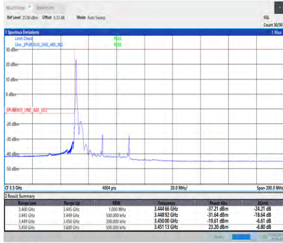
1-N78-3450-3550-PC3-30-40-L-1-DFT-PI2BPSK-Edge_1RB_Left-1@0-Ant1-1--PASS-see graph
