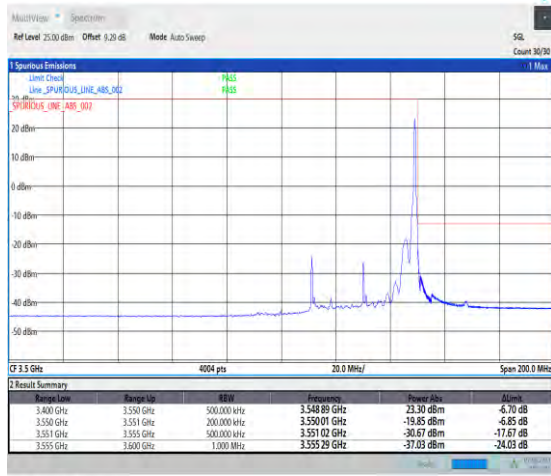
1-N78-3450-3550-PC3-30-40-H-2-DFT-PI2BPSK-Edge_1RB_Right-1@105-Ant1-1--PASS-see graph
