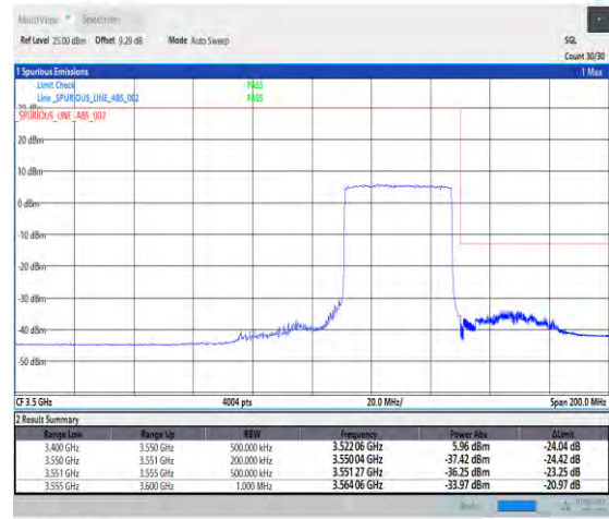
1-N78-3450-3550-PC3-30-40-H-3-DFT-PI2BPSK-Outer_Full-100@0-Ant1-1--PASS-see graph
