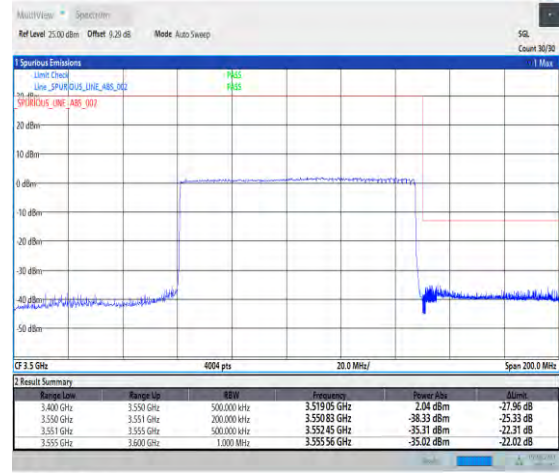
1-N78-3450-3550-PC3-30-90-H-3-DFT-PI2BPSK-Outer_Full-240@0-Ant1-1--PASS-see graph
