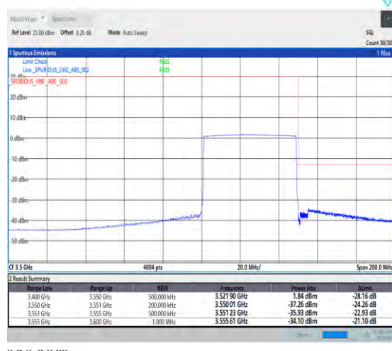
1-N78-3450-3550-PC3-30-50-H-6-CP-QPSK-Outer_Full-133@0-Ant1-1--PASS-see graph
