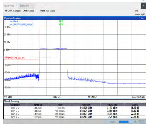
1-N78-3450-3550-PC3-30-40-L-6-CP-QPSK-Outer_Full-106@0-Ant1-1--PASS-see graph
