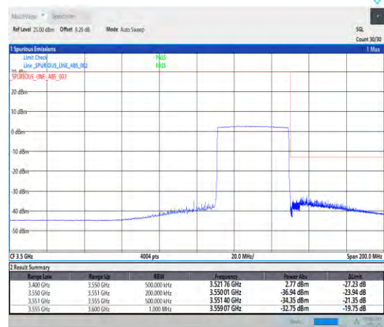
1-N78-3450-3550-PC3-30-40-H-6-CP-QPSK-Outer_Full-106@0-Ant1-1--PASS-see graph
