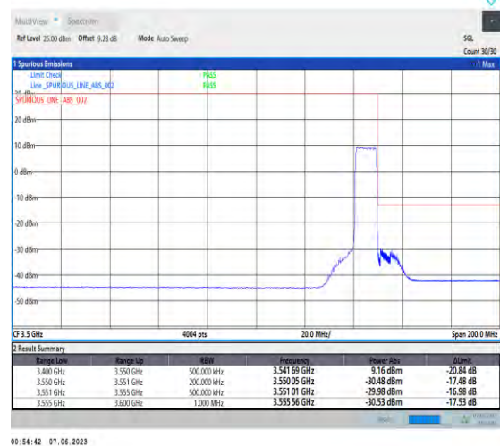
1-N78-3450-3550-PC3-30-10-H-6-CP-QPSK-Outer_Full-24@0-Ant1-1--PASS-see graph
