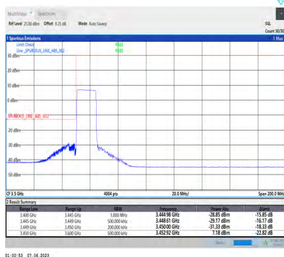
1-N78-3450-3550-PC3-30-15-L-6-CP-QPSK-Outer_Full-38@0-Ant1-1--PASS-see graph
