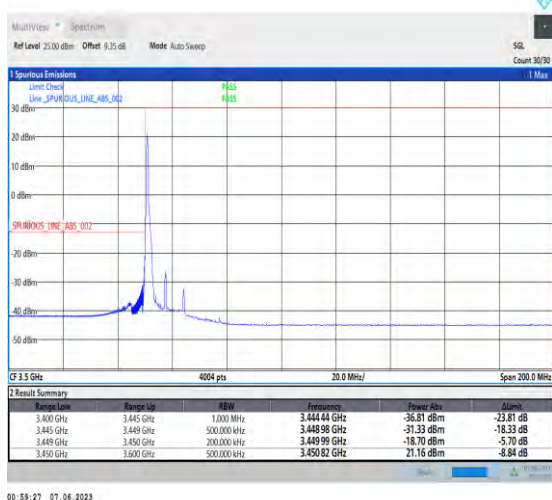
1-N78-3450-3550-PC3-30-15-L-4-CP-QPSK-Edge_1RB_Left-1@0-Ant1-1--PASS-see graph
