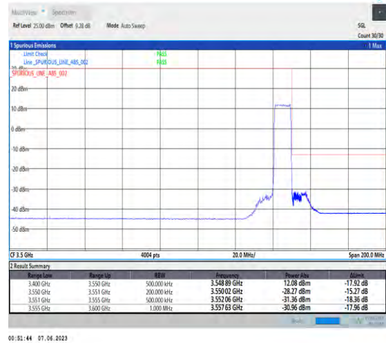
1-N78-3450-3550-PC3-30-10-H-3-DFT-PI2BPSK-Outer_Full-24@0-Ant1-1--PASS-see graph
