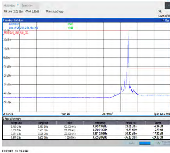
1-N78-3450-3550-PC3-30-10-H-2-DFT-PI2BPSK-Edge_1RB_Right-1@23-Ant1-1--PASS-see graph
