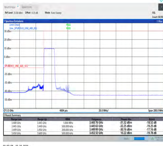
1-N78-3450-3550-PC3-30-15-L-3-DFT-PI2BPSK-Outer_Full-36@0-Ant1-1--PASS-see graph
