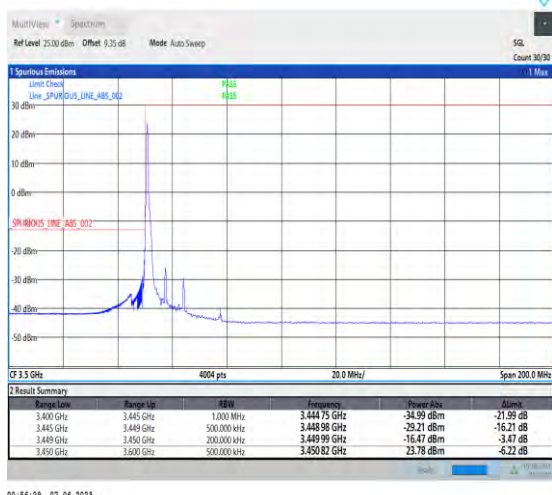
1-N78-3450-3550-PC3-30-15-L-1-DFT-PI2BPSK-Edge_1RB_Left-1@0-Ant1-1--PASS-see graph
