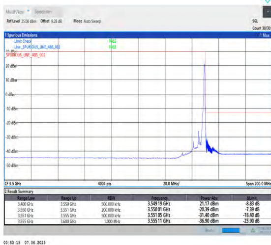
1-N78-3450-3550-PC3-30-10-H-5-CP-QPSK-Edge_1RB_Right-1@23-Ant1-1--PASS-see graph
