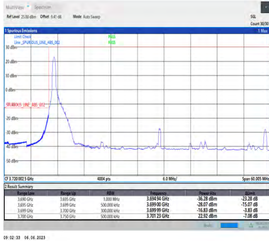
1-N77-3700-3980-PC3-30-50-L-1-DFT-PI2BPSK-Edge_1RB_Left-1@0-Ant1-1--PASS-see graph
