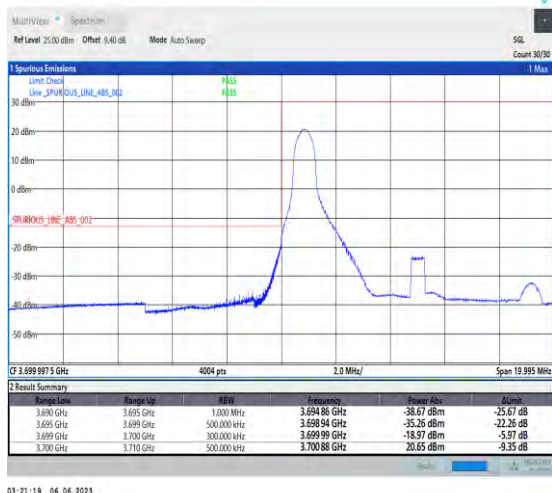
1-N77-3700-3980-PC3-30-10-L-4-CP-QPSK-Edge_1RB_Left-1@0-Ant1-1--PASS-see graph
