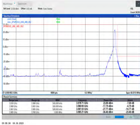
1-N77-3700-3980-PC3-30-50-H-2-DFT-PI2BPSK-Edge_1RB_Right-1@132-Ant1-1--PASS-see graph
