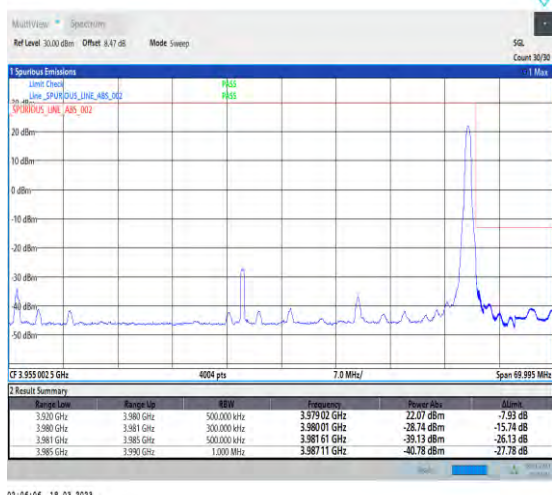
1-N77-3700-3980-PC3-30-60-H-2-DFT-PI2BPSK-Edge_1RB_Right-1@161-Ant1-1--PASS-see graph
