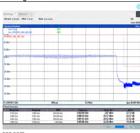
1-N77-3700-3980-PC3-30-70-H-3-DFT-PI2BPSK-Outer_Full-180@0-Ant1-1--PASS-see graph
