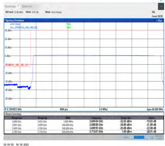
1-N77-3700-3980-PC3-30-50-L-6-CP-QPSK-Outer_Full-133@0-Ant1-1--PASS-see graph
