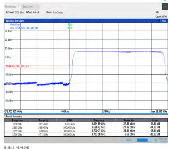
1-N77-3700-3980-PC3-30-15-L-6-CP-QPSK-Outer_Full-38@0-Ant1-1--PASS-see graph
