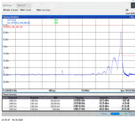
1-N77-3700-3980-PC3-30-90-H-5-CP-QPSK-Edge_1RB_Right-1@244-Ant1-1--PASS-see graph
