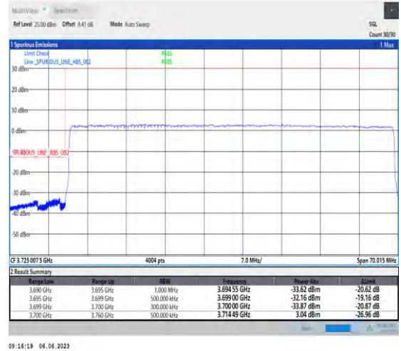
1-N77-3700-3980-PC3-30-60-L-3-DFT-PI2BPSK-Outer_Full-162@0-Ant1-1--PASS-see graph
