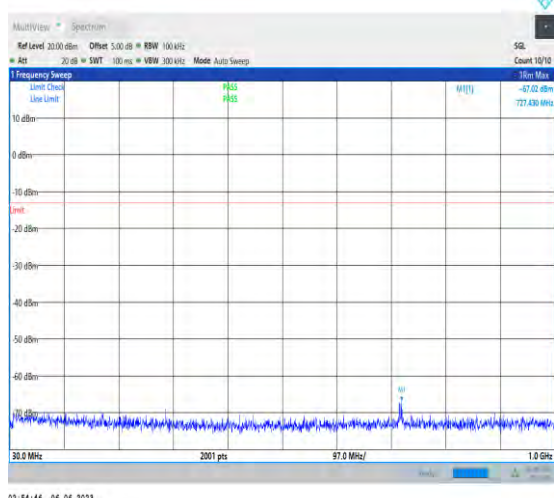
1-N77-3700-3980-PC3-30-100-M-1-N/A-DFT-PI2BP SK-Inner_1RB_Left-1@1-30-1000-Ant1-727.43--67. 02--13-PASS
