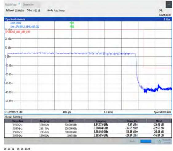
1-N77-3700-3980-PC3-30-50-H-3-DFT-PI2BPSK-Outer_Full-128@0-Ant1-1--PASS-see graph
