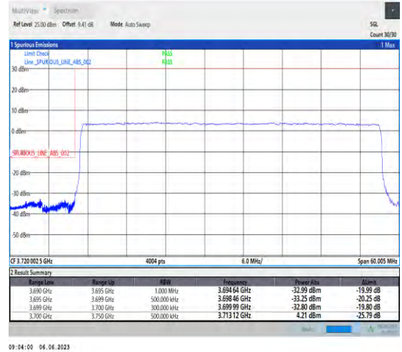
1-N77-3700-3980-PC3-30-50-L-3-DFT-PI2BPSK-Outer_Full-128@0-Ant1-1--PASS-see graph
