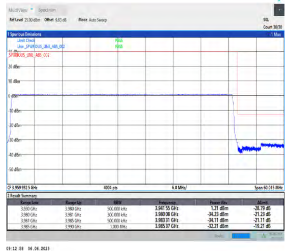
1-N77-3700-3980-PC3-30-50-H-6-CP-QPSK-Outer_Full-133@0-Ant1-1--PASS-see graph
