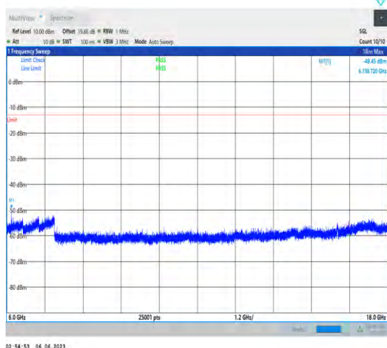
1-N77-3700-3980-PC3-30-100-M-1-N/A-DFT-PI2BP SK-Inner_1RB_Left-1@1-6000-18000-Ant1-6138.72 --49.45--13-PASS
