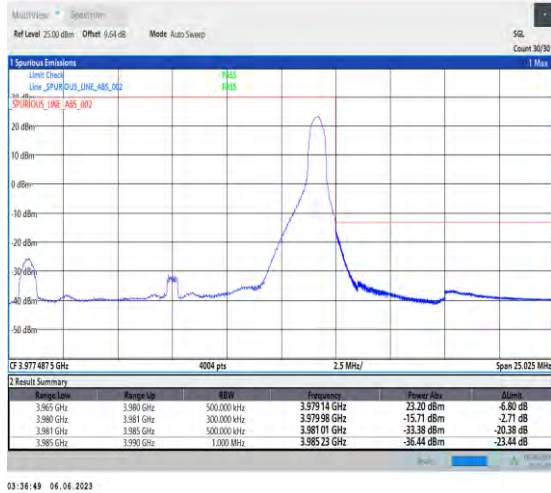
1-N77-3700-3980-PC3-30-15-H-2-DFT-PI2BPSK-Edge_1RB_Right-1@37-Ant1-1--PASS-see graph
