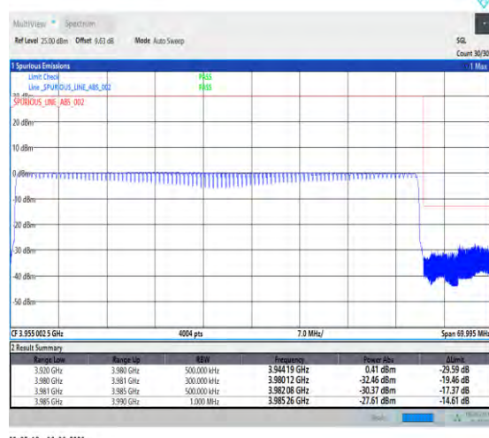
1-N77-3700-3980-PC3-30-60-H-6-CP-QPSK-Outer_Full-162@0-Ant1-1--PASS-see graph
