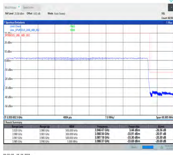
1-N77-3700-3980-PC3-30-60-H-3-DFT-PI2BPSK-Outer_Full-162@0-Ant1-1--PASS-see graph
