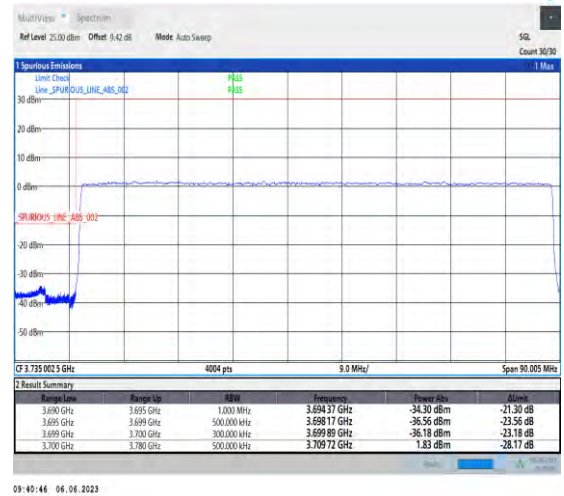
1-N77-3700-3980-PC3-30-80-L-3-DFT-PI2BPSK-Outer_Full-216@0-Ant1-1--PASS-see graph
