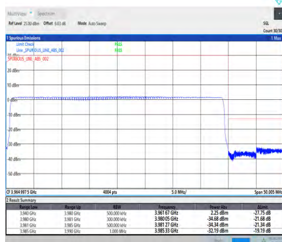
1-N77-3700-3980-PC3-30-40-H-6-CP-QPSK-Outer_Full-106@0-Ant1-1--PASS-see graph
