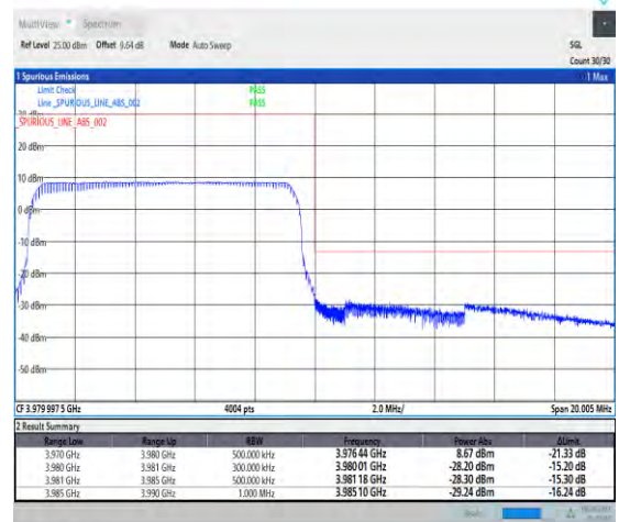
1-N77-3700-3980-PC3-30-10-H-6-CP-QPSK-Outer_Full-24@0-Ant1-1--PASS-see graph
