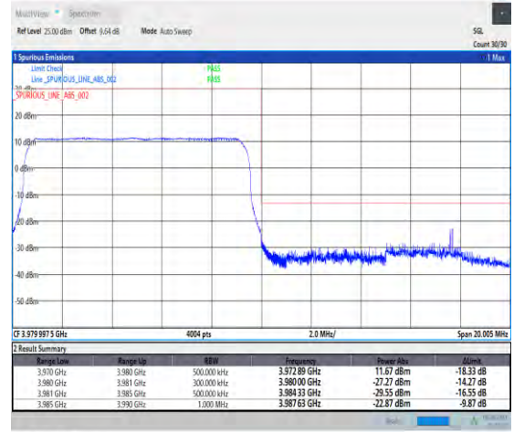
1-N77-3700-3980-PC3-30-10-H-3-DFT-PI2BPSK-Outer_Full-24@0-Ant1-1--PASS-see graph
