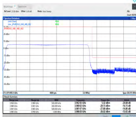
1-N77-3700-3980-PC3-30-20-H-6-CP-QPSK-Outer_Full-51@0-Ant1-1--PASS-see graph
