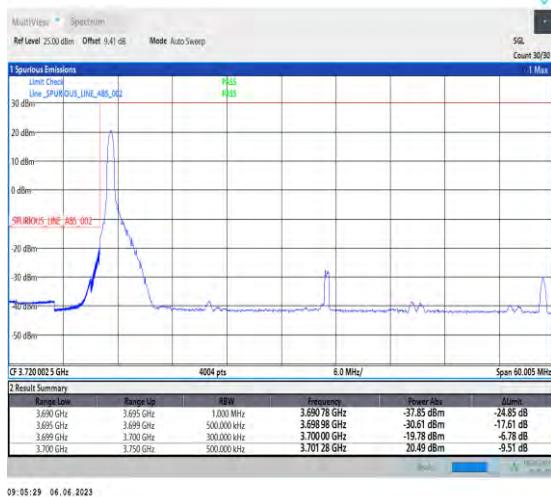
1-N77-3700-3980-PC3-30-50-L-4-CP-QPSK-Edge_1RB_Left-1@0-Ant1-1--PASS-see graph
