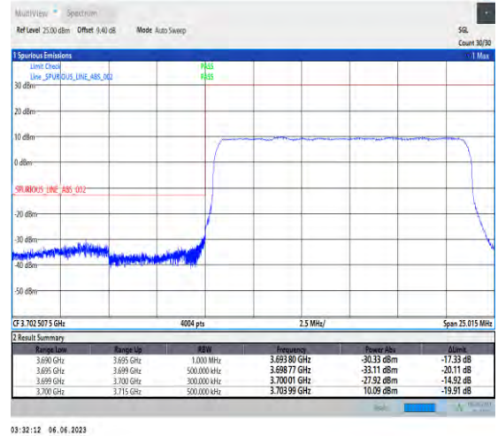
1-N77-3700-3980-PC3-30-15-L-3-DFT-PI2BPSK-Outer_Full-36@0-Ant1-1--PASS-see graph
