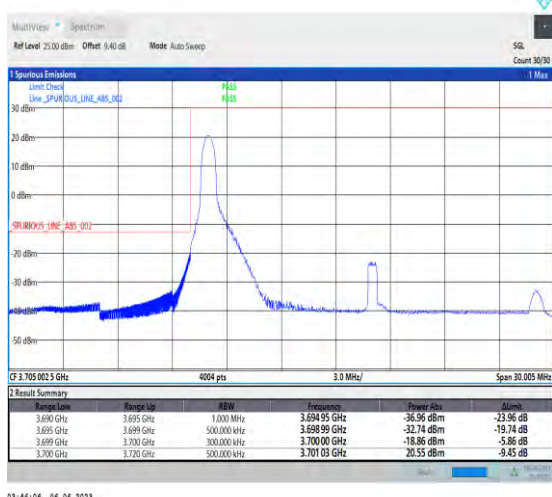
1-N77-3700-3980-PC3-30-20-L-4-CP-QPSK-Edge_1RB_Left-1@0-Ant1-1--PASS-see graph
