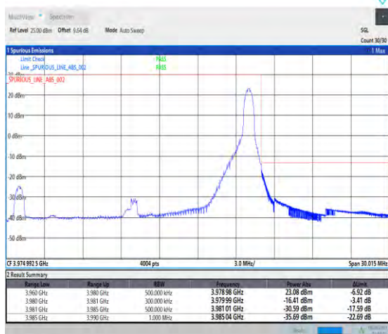
1-N77-3700-3980-PC3-30-20-H-2-DFT-PI2BPSK-Edge_1RB_Right-1@50-Ant1-1--PASS-see graph
