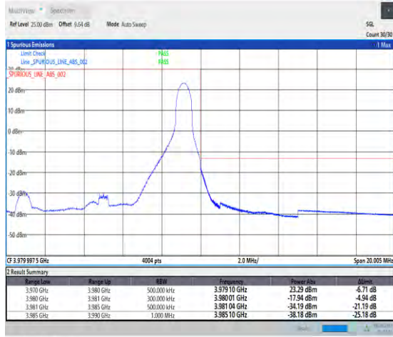
1-N77-3700-3980-PC3-30-10-H-2-DFT-PI2BPSK-Edge_1RB_Right-1@23-Ant1-1--PASS-see graph
