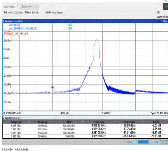
1-N77-3700-3980-PC3-30-15-H-5-CP-QPSK-Edge_1RB_Right-1@37-Ant1-1--PASS-see graph
