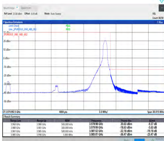
1-N77-3700-3980-PC3-30-20-H-5-CP-QPSK-Edge_1RB_Right-1@50-Ant1-1--PASS-see graph
