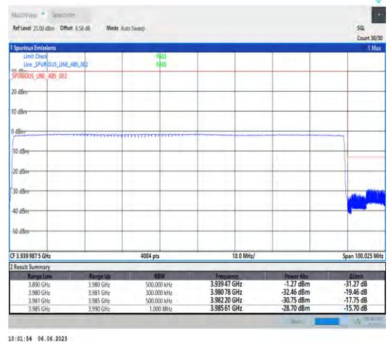
1-N77-3700-3980-PC3-30-90-H-6-CP-QPSK-Outer_Full-245@0-Ant1-1--PASS-see graph
