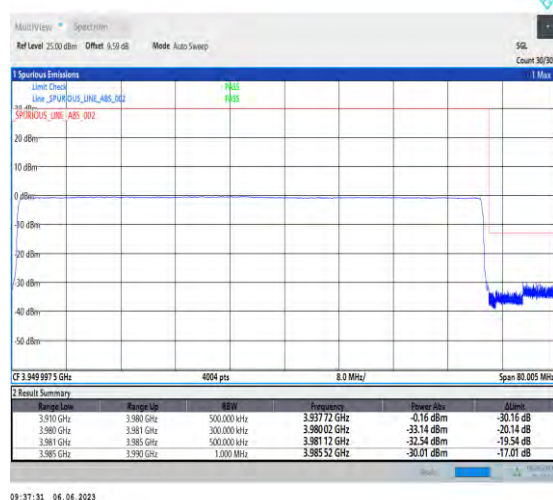
1-N77-3700-3980-PC3-30-70-H-6-CP-QPSK-Outer_Full-189@0-Ant1-1--PASS-see graph
