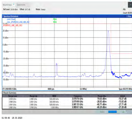
1-N77-3700-3980-PC3-30-50-H-5-CP-QPSK-Edge_1RB_Right-1@132-Ant1-1--PASS-see graph
