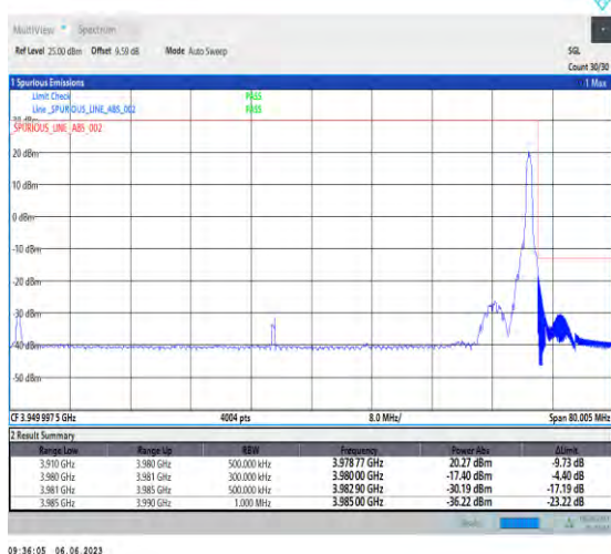
1-N77-3700-3980-PC3-30-70-H-5-CP-QPSK-Edge_1RB_Right-1@188-Ant1-1--PASS-see graph
