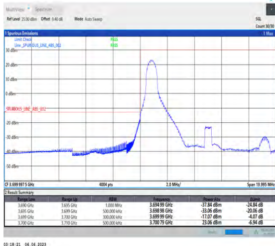
1-N77-3700-3980-PC3-30-10-L-1-DFT-PI2BPSK-Edge_1RB_Left-1@0-Ant1-1--PASS-see graph
