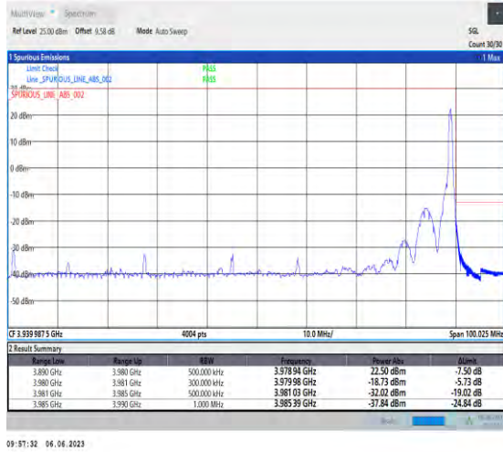
1-N77-3700-3980-PC3-30-90-H-2-DFT-PI2BPSK-Edge_1RB_Right-1@244-Ant1-1--PASS-see graph
