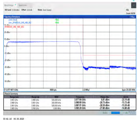
1-N77-3700-3980-PC3-30-15-H-6-CP-QPSK-Outer_Full-38@0-Ant1-1--PASS-see graph
