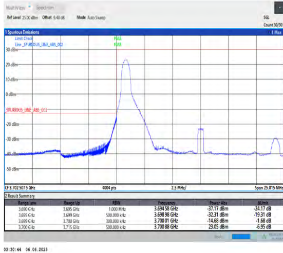
1-N77-3700-3980-PC3-30-15-L-1-DFT-PI2BPSK-Edge_1RB_Left-1@0-Ant1-1--PASS-see graph
