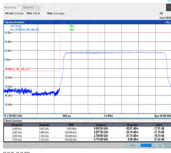
1-N77-3700-3980-PC3-30-20-L-3-DFT-PI2BPSK-Outer_Full-50@0-Ant1-1--PASS-see graph
