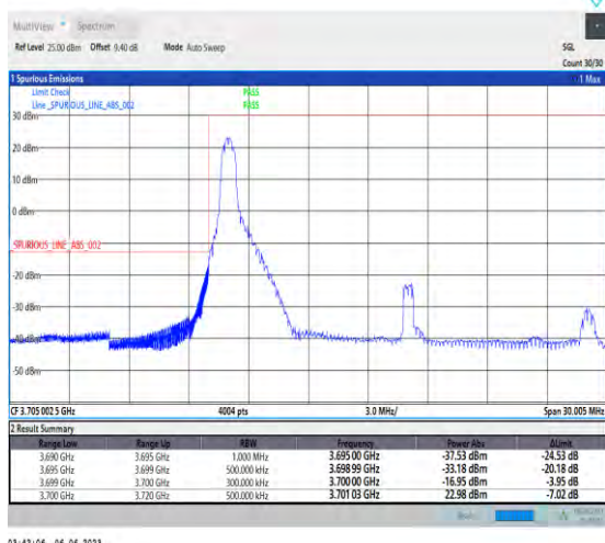
1-N77-3700-3980-PC3-30-20-L-1-DFT-PI2BPSK-Edge_1RB_Left-1@0-Ant1-1--PASS-see graph
