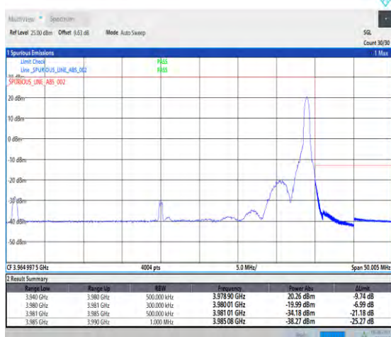
1-N77-3700-3980-PC3-30-40-H-5-CP-QPSK-Edge_1RB_Right-1@105-Ant1-1--PASS-see graph
