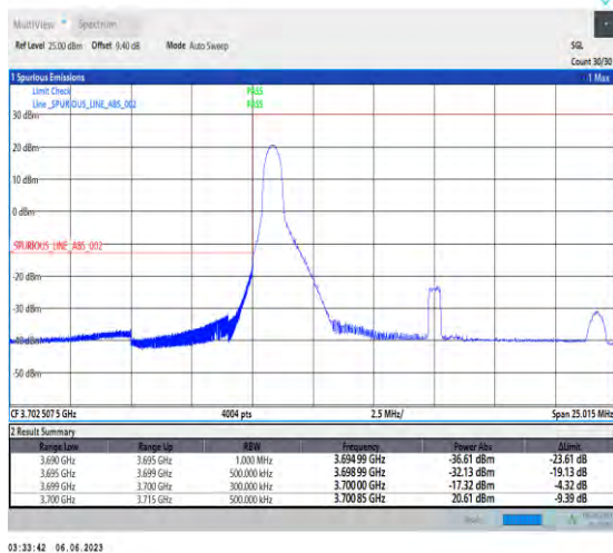
1-N77-3700-3980-PC3-30-15-L-4-CP-QPSK-Edge_1RB_Left-1@0-Ant1-1--PASS-see graph
