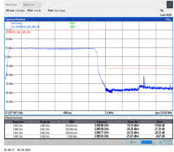
1-N77-3700-3980-PC3-30-15-H-3-DFT-PI2BPSK-Outer_Full-36@0-Ant1-1--PASS-see graph
