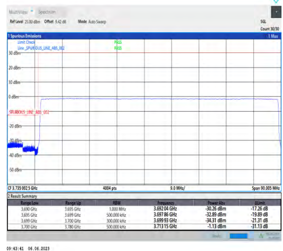
1-N77-3700-3980-PC3-30-80-L-6-CP-QPSK-Outer_Full-217@0-Ant1-1--PASS-see graph
