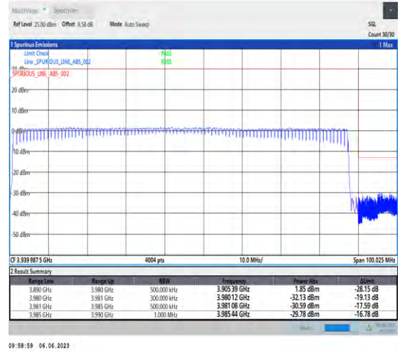
1-N77-3700-3980-PC3-30-90-H-3-DFT-PI2BPSK-Outer_Full-240@0-Ant1-1--PASS-see graph
