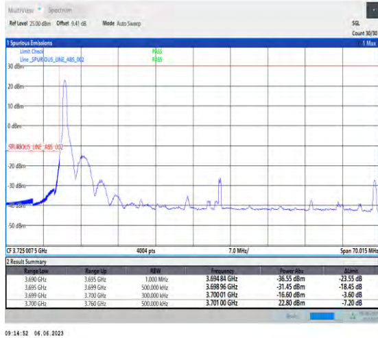
1-N77-3700-3980-PC3-30-60-L-1-DFT-PI2BPSK-Edge_1RB_Left-1@0-Ant1-1--PASS-see graph
