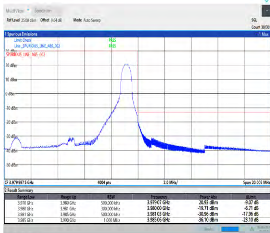
1-N77-3700-3980-PC3-30-10-H-5-CP-QPSK-Edge_1RB_Right-1@23-Ant1-1--PASS-see graph
