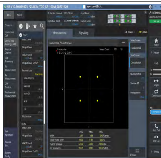
1-N77-3700-3980-PC3-30-100-M-6-CP-QPSK-Outer_Full-273@0-Ant1-see graph-PASS
