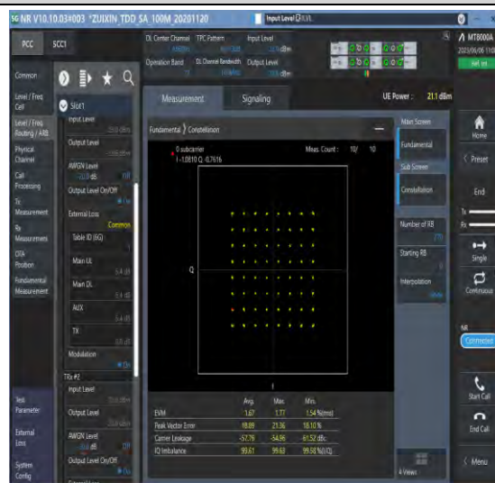
1-N77-3700-3980-30-100-M-4-DFT-64QAM-Outer_Full-270@0-Ant1-see graph-PASS
