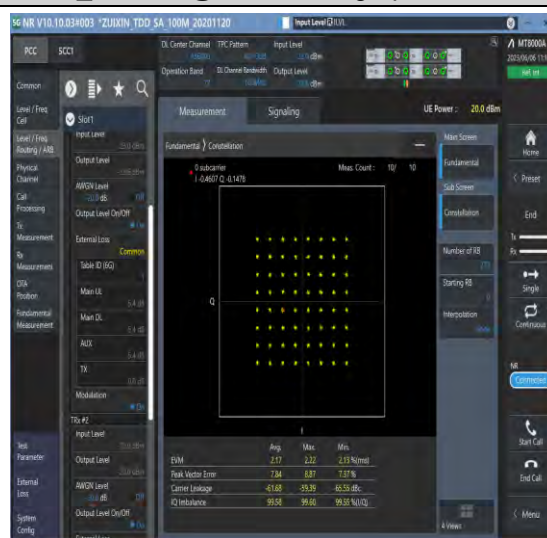
1-N77-3700-3980-PC3-30-100-M-8-CP-64QAM-Outer_Full-273@0-Ant1-see graph-PASS
