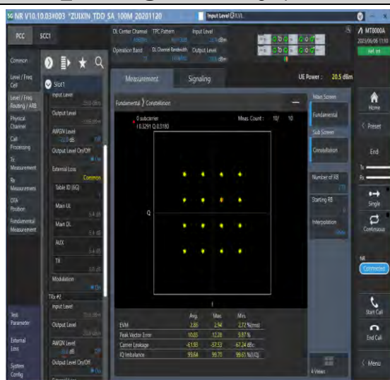
1-N77-3700-3980-PC3-30-100-M-7-CP-16QAM-Outer_Full-273@0-Ant1-see graph-PASS
