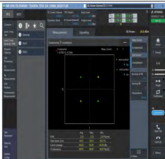
1-N77-3700-3980-30-100-M-1-DFT-PI2BPSK-Outer_Full-270@0-Ant1-see graph-PASS
