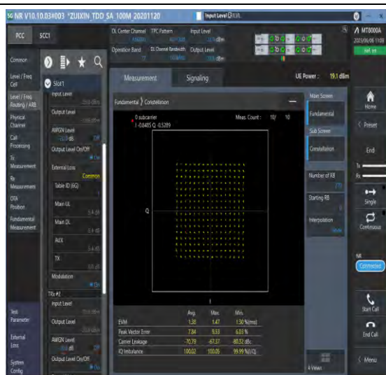
1-N77-3700-3980-PC3-30-100-M-5-DFT-25QAM-Outer_Full-270@0-Ant1-see graph-PASS
