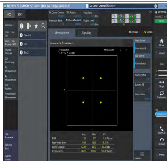
1-N77-3700-3980-30-100-M-2-DFT-QPSK-Outer_Full-270@0-Ant1-see graph-PASS
