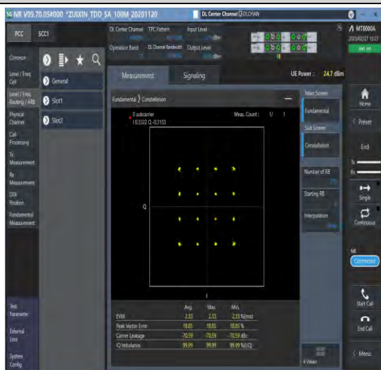
1-N77-3700-3980-30-100-M-3-DFT-16QAM-Outer_Full-270@0-Ant1-see graph-PASS
