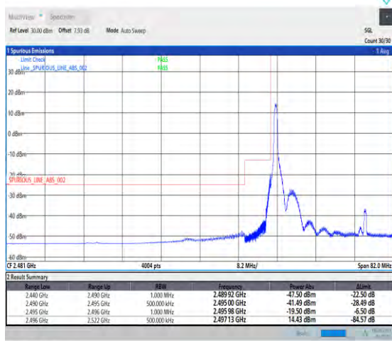
1-N41-PC3-30-40-L-4-CP-QPSK-Edge_1RB_Left-1@0-Ant1-1--PASS-see graph
