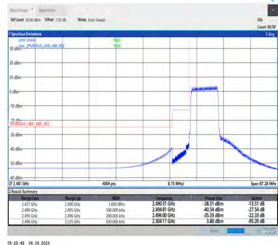
1-N41-PC3-30-10-L-6-CP-QPSK-Outer_Full-24@0-Ant1-1--PASS-see graph
