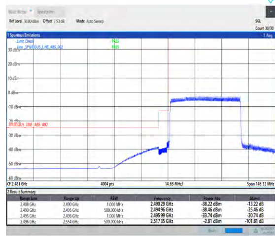
1-N41-PC3-30-40-L-6-CP-QPSK-Outer_Full-106@0-Ant1-1--PASS-see graph
