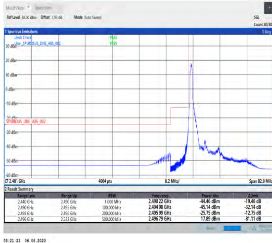
1-N41-PC3-30-10-L-1-DFT-PI2BPSK-Edge_1RB_Left-1@0-Ant1-1--PASS-see graph
