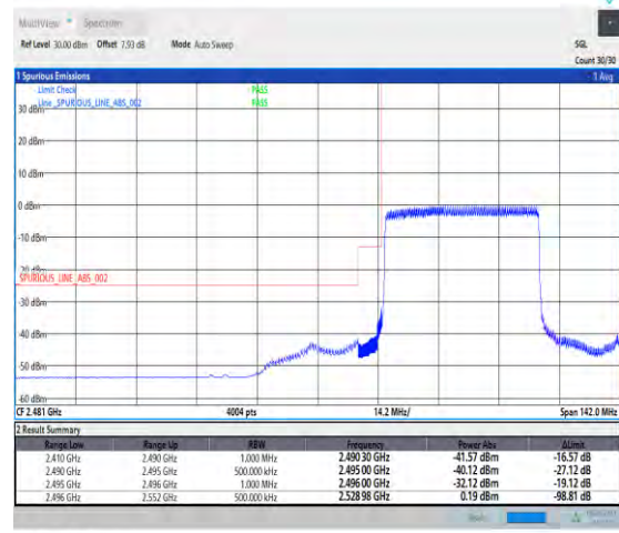
1-N41-PC3-30-40-L-3-DFT-PI2BPSK-Outer_Full-100@0-Ant1-1--PASS-see graph
