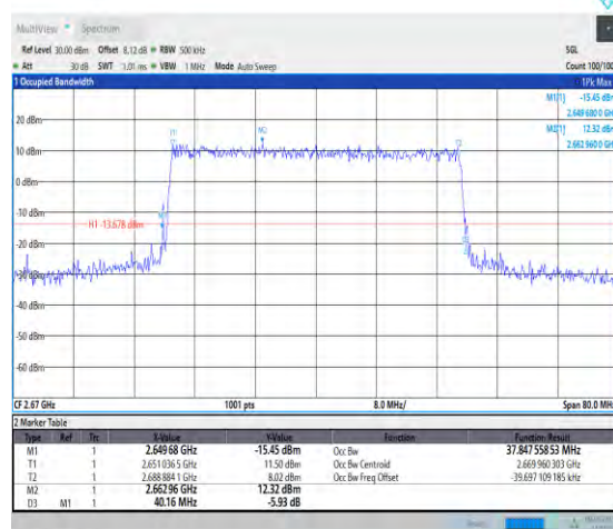
1-N41-PC3-30-40-H-6-CP-QPSK-Outer_Full-106@0 -Ant1-37.848-40.160-≤40-PASS
