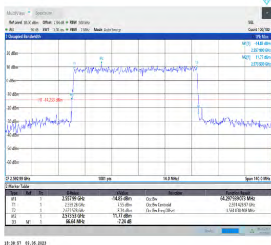
1-N41-PC3-30-70-M-3-DFT-16QAM-Out_ Full-180 @0-Ant1-64.298-66.640-≤70-PASS
