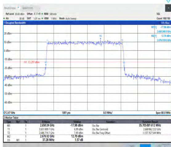
1-N41-PC3-30-40-H-5-DFT-256QAM-Outer_Full-100 @0-Ant1-35.705-37.28-≤40-PASS
