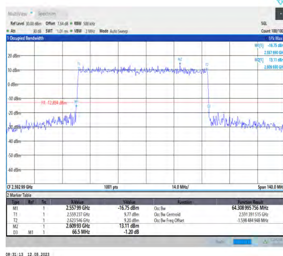
1-N41-PC3-30-70-M-4-DFT-64QAM-Out_ Full-180 @0-Ant1-64.309-66.50-≤70-PASS
