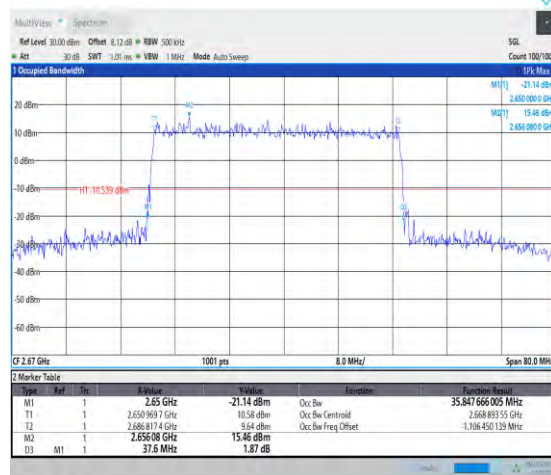
1-N41-PC3-30-40-H-4-DFT-64QAM-Outer_Full-100 @0-Ant1-35.848-37.600-≤40-PASS
