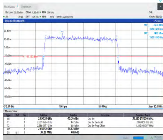
1-N41-PC3-30-40-H-3-DFT-16QAM-Outer_Full-100 @0-Ant1-35.595-37.280-≤40-PASS
