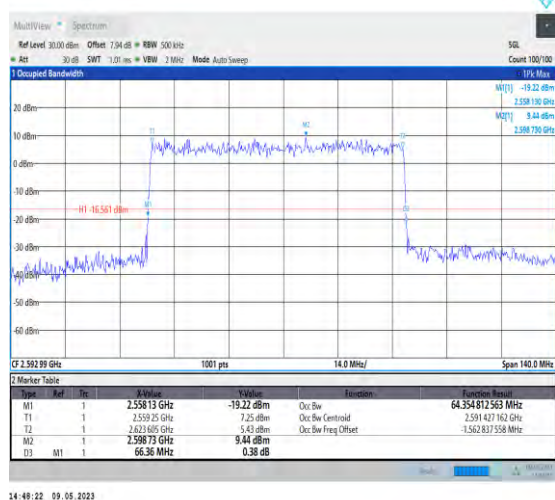
1-N41-PC3-30-70-M-5-DFT-256QAM-Out_ Full-180 @0-Ant1-64.355-66.360-≤70-PASS
