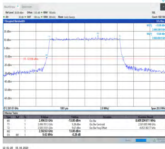
1-N41-PC3-30-10-L-4-DFT-64QAM-Outer_Full-24@0 -Ant1-8.609-9.420≤10-PASS
