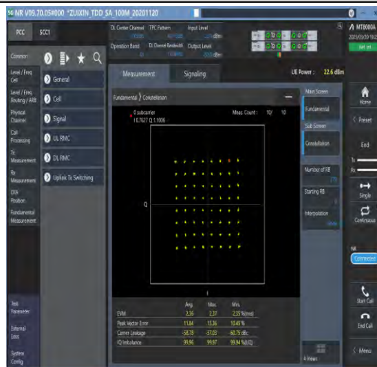
1-N41-30-100-M-4-DFT-64QAM-Outer_Full-270@0-Ant1-see graph-PASS
