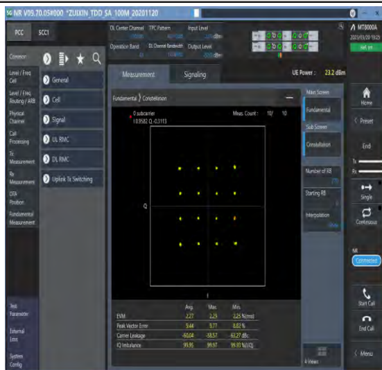
1-N41-30-100-M-3-DFT-16QAM-Outer_Full-270@0-Ant1-see graph-PASS
