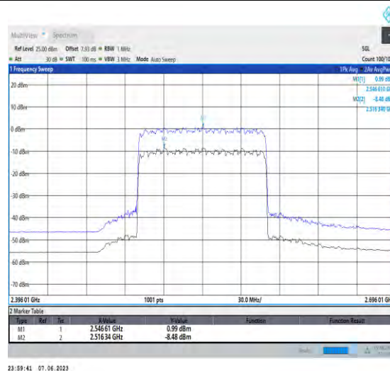
1-N41-PC3-30-100-L-2-CP-256QAM-Outer_Full-273 @0-Ant1-9.47-100%-0.00-9.47-PASS-≤13
