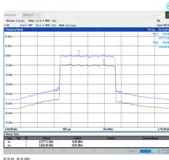
1-N41-PC3-30-100-M-2-CP-256QAM-Outer_Full-27 3@0-Ant1-9.54-100%-0.00-9.54-PASS-≤13
