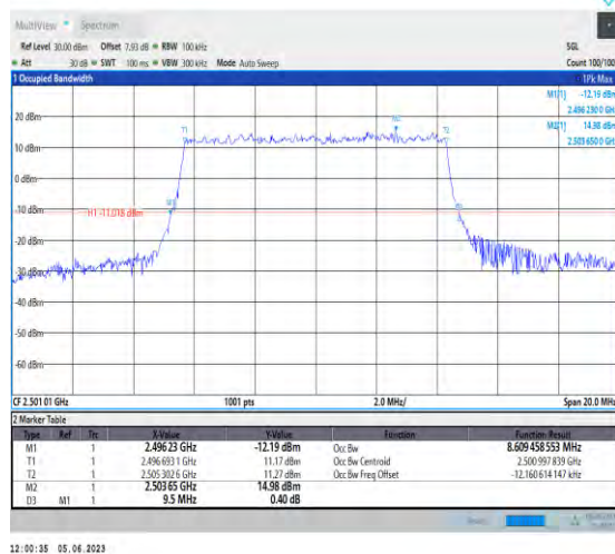
1-N41-PC3-30-10-L-2-DFT-PI2BPSK-Outer_Full-24@0 @0-Ant1-8.609-9.500≤10-PASS
