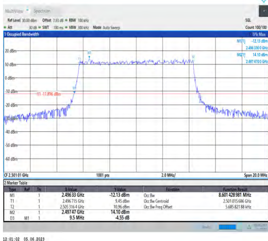
1-N41-PC3-30-10-L-3-DFT-16QAM-Outer_Full-24@0 0-Ant1-8.601-9.500≤10-PASS
