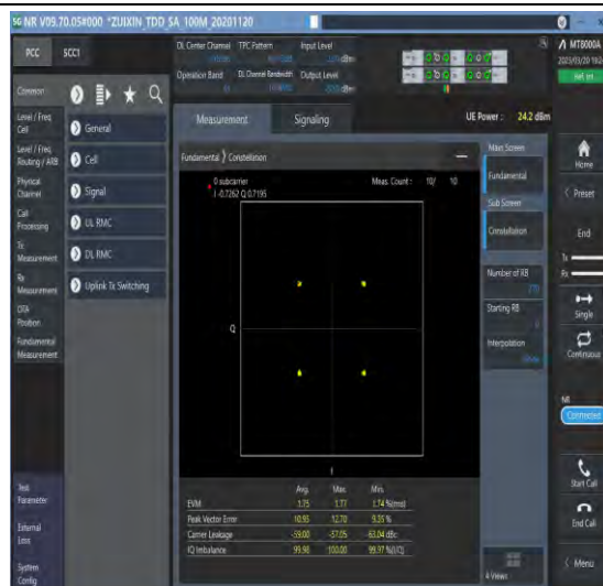
1-N41-30-100-M-2-DFT-QPSK-Outer_Full-270@0-Ant1-see graph-PASS
