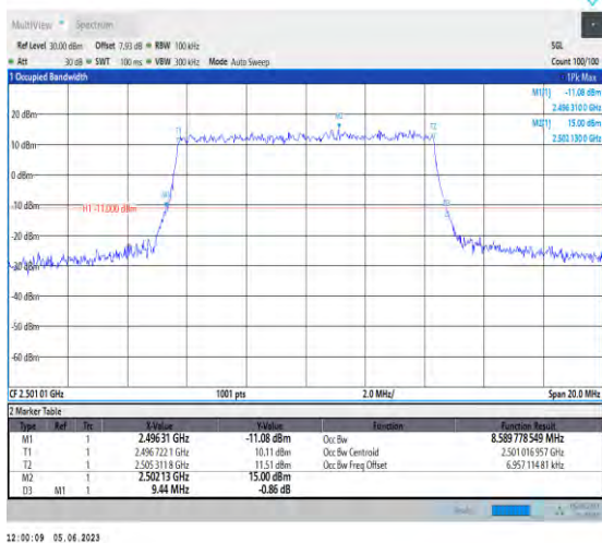
1-N41-PC3-30-10-L-1-DFT-QPSK-Outer_Full-24@0 -Ant1-8.59-9.440≤10-PASS
