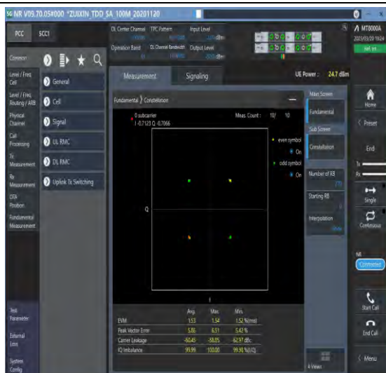
1-N41-30-100-M-1-DFT-PI2BPSK-Outer_Full-270@0-Ant1-see graph-PASS
