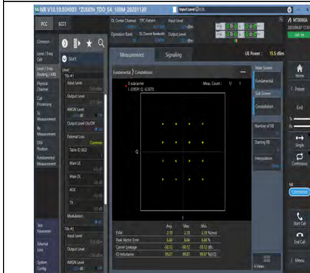
1-N38-PC3-30-20-M-7-CP-16QAM-Outer_Full-51@0-Ant1-see graph-PASS
