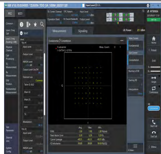
1-N38-PC3-30-20-M-8-CP-64QAM-Outer_Full-51@0-Ant1-see graph-PASS
