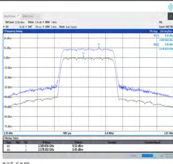
1-N38-PC3-30-20-L-1-DFT-256QAM-Outer_Full-50@ 0-Ant1-9.07-100%-0.00-9.07-PASS-≤13
