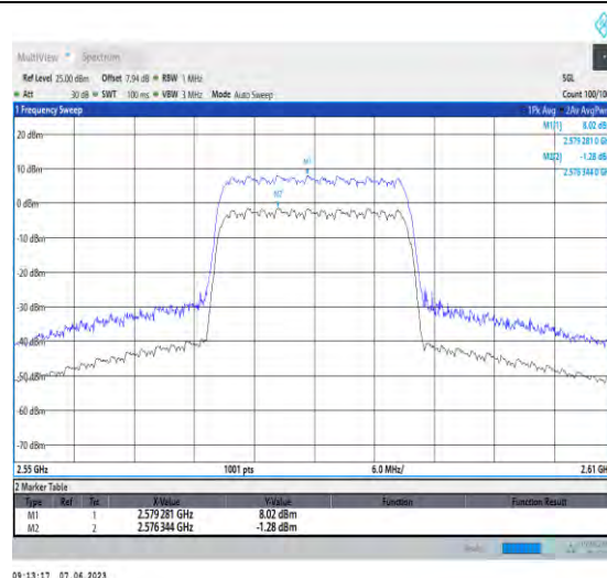
1-N38-PC3-30-20-L-2-CP-256QAM-Outer_Full-51@ 0-Ant1-9.30-100%-0.00-9.30-PASS-≤13
