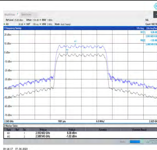
1-N38-PC3-30-20-M-2-CP-256QAM-Outer_Full-51 @0-Ant1-9.40-100%-0.00-9.40-PASS-≤13
