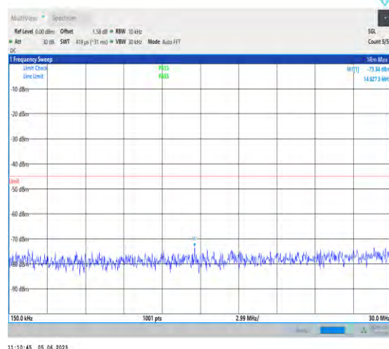
1-N38-PC3-30-20-M-1-N/A-DFT-PI2BPSK-Inner_1RB _Left-1@1-0.15-30-Ant1-14.63--73.34--45-PASS
