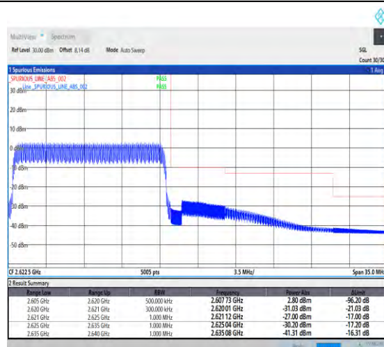
1-N38-PC3-30-15-H-3-DFT-PI2BPSK-Outer_Full-36@0-Ant1-1--PASS-see graph
