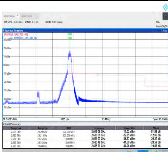
1-N38-PC3-30-15-H-2-DFT-PI2BPSK-Edge_1RB_Right-t-1@37-Ant1-1--PASS-see graph
