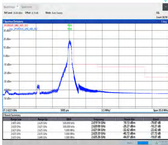
1-N38-PC3-30-15-H-2-DFT-PI2BPSK-Edge_1RB_Right-t-1@37-Ant1-1--PASS-see graph
