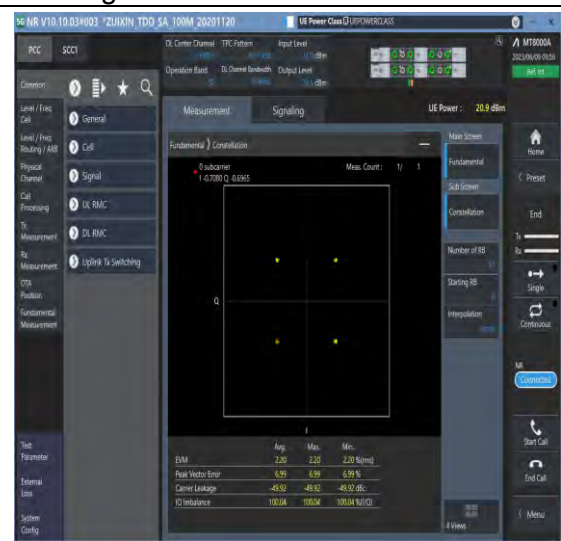
1-N38-PC3-30-20-M-6-CP-QPSK-Outer_Full-51@0-Ant1-see graph-PASS
