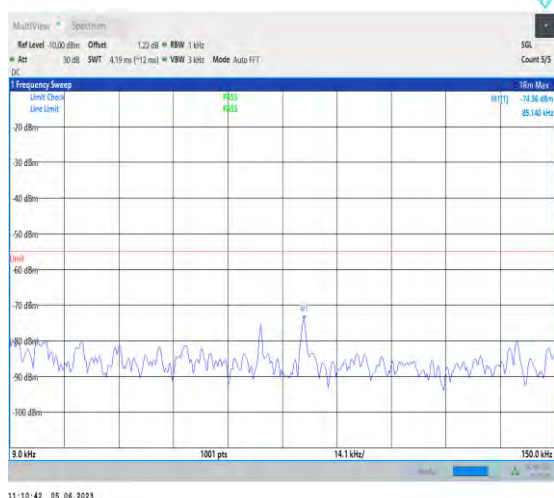
1-N38-PC3-30-20-M-1-N/A-DFT-PI2BPSK-Inner_1R B_Left-1@1-0.009-0.15-Ant1-0.09--74.36--55-PASS
