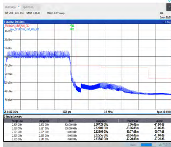
1-N38-PC3-30-15-H-3-DFT-PI2BPSK-Outer_Full-36@0-Ant1-1--PASS-see graph
