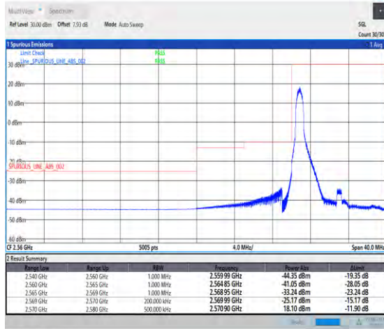
1-N38-PC3-30-10-L-1-DFT-PI2BPSK-Edge_1RB_Left-1@0-Ant1-1--PASS-see graph
