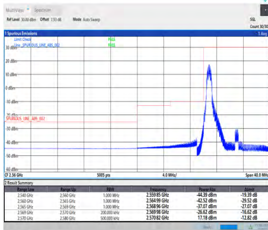
1-N38-PC3-30-10-L-4-CP-QPSK-Edge_1RB_Left-1@0-Ant1-1--PASS-see graph
