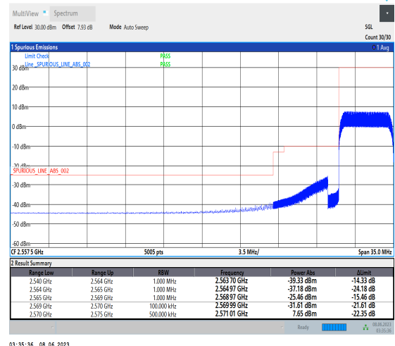
1-N38-PC3-15-5-L-6-CP-QPSK-Outer_Full-25@0-Ant1-1--PASS-see graph
