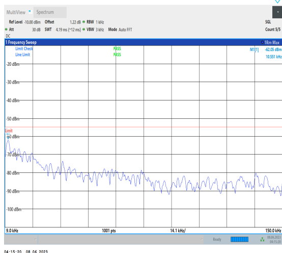
1-N38-PC3-15-5-M-1-N/A-DFT-PI2BPSK-Inner_1RB _Left-1@1-0.009-0.15-Ant1-0.01--62.05--55-PASS
