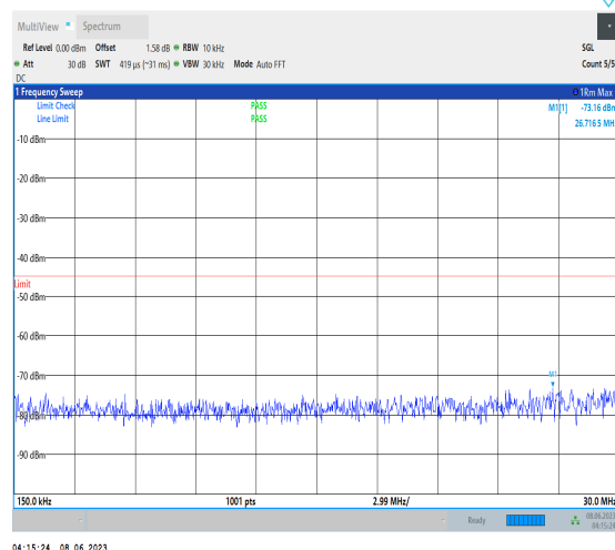
1-N38-PC3-15-5-M-1-N/A-DFT-PI2BPSK-Inner_1RB_ Left-1@1-0.15-30-Ant1-28.21--73.16--45-PASS
