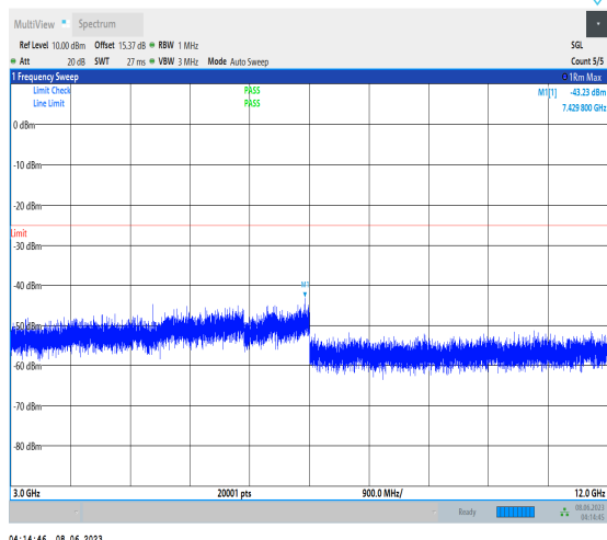
1-N38-PC3-15-5-L-1-N/A-DFT-PI2BPSK-Inner_1RB _Left-1@1-3000-12000-Ant1-5141.10--43.23--25-PA SS
