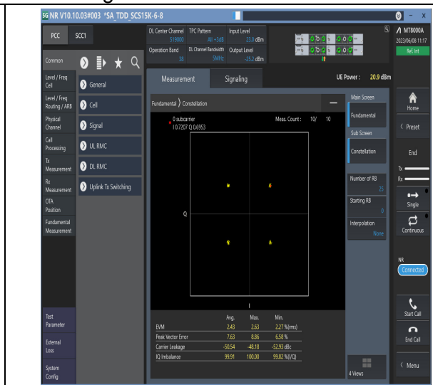
1-N38-PC3-15-5-M-6-CP-QPSK-Outer_Full-25@0-Ant1-see graph-PASS
