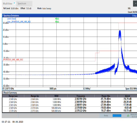
1-N38-PC3-15-5-L-1-DFT-PI2BPSK-Edge_1RB_Left-1 @0-Ant1-1--PASS-see graph
