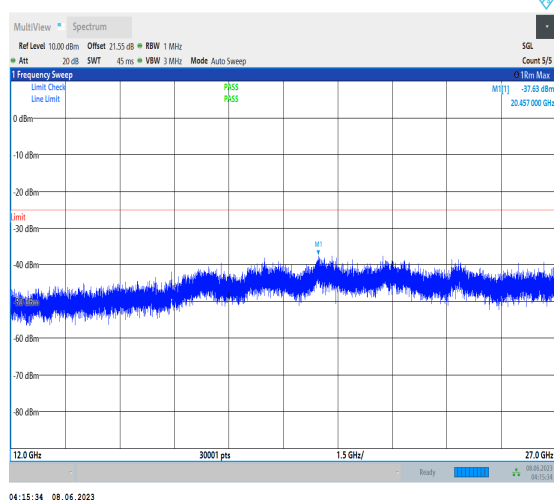
1-N38-PC3-15-5-M-1-N/A-DFT-PI2BPSK-Inner_1RB_ Left-1@1-12000-27000-Ant1-20492.00--37.63--25-PA SS
