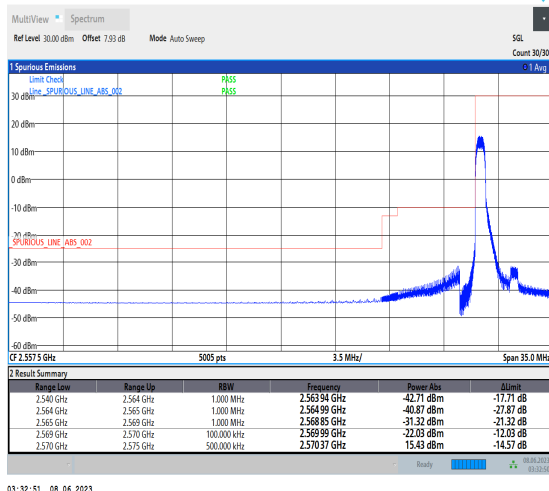
1-N38-PC3-15-5-L-4-CP-QPSK-Edge_1RB_Left-1@0-Ant1-1--PASS-see graph
