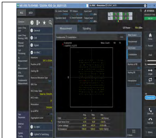
1-N26-824-849-PC3-15-20-M-5-DFT-256QAM-Outer_Fu II-100@0-Ant1-see graph-PASS
