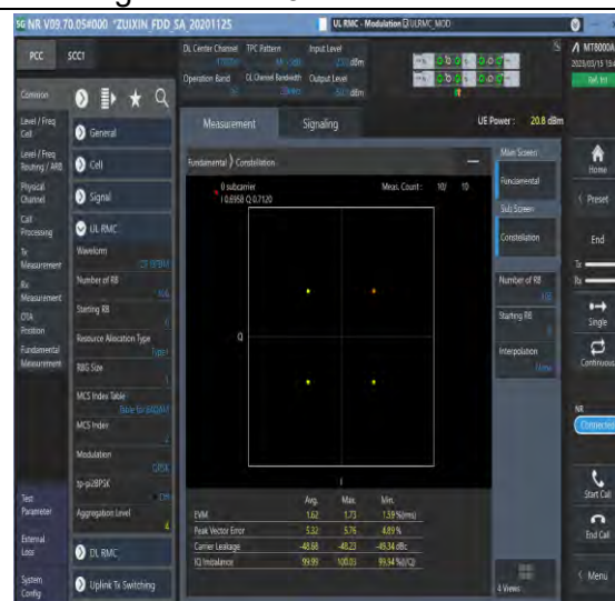
1-N26-824-849-PC3-15-20-M-6-CP-QPSK-Outer_Full-1 06@0-Ant1-see graph-PASS
