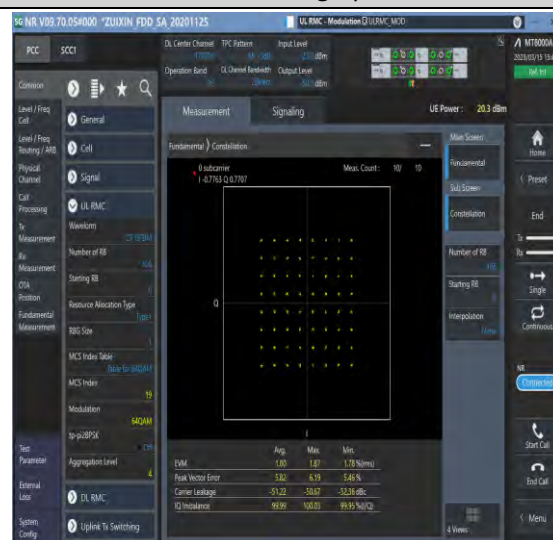
1-N26-824-849-PC3-15-20-M-8-CP-64QAM-Outer_Full -106@0-Ant1-see graph-PASS
