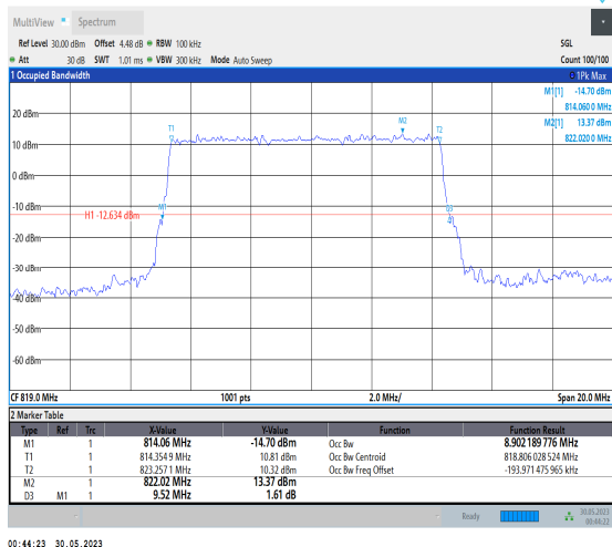
NTNV_N26-814-824_PC3_15_10_M_TID2_Ant1#1
