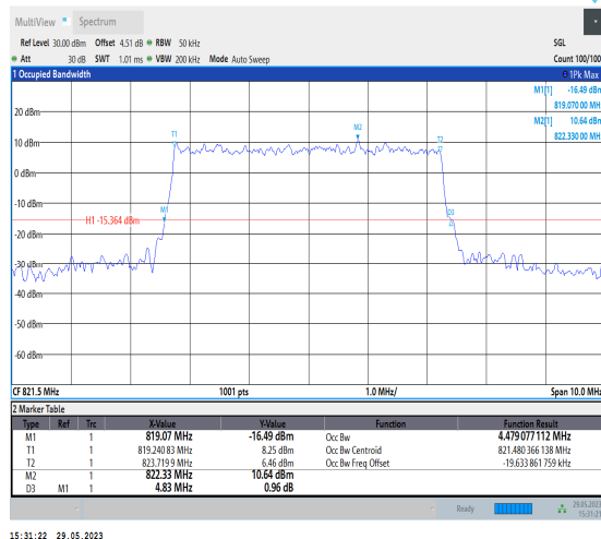
NTNV_N26-814-824_PC3_15_5_H_TID8_Ant1#1
