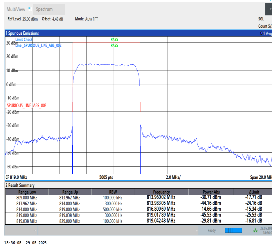
1-N26-814-824-PC3-15-5-L-3-DFT-PI2BPSK-Outer_Full-25@0-Ant1-1--PASS-see graph
