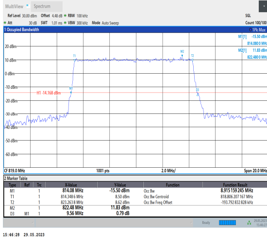
NTVN_N26-814-824_PC3_15_10_M_TID4_Ant1#1
