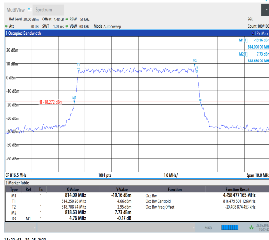
NTNV_N26-814-824_PC3_15_5_L_TID9_Ant1#1
