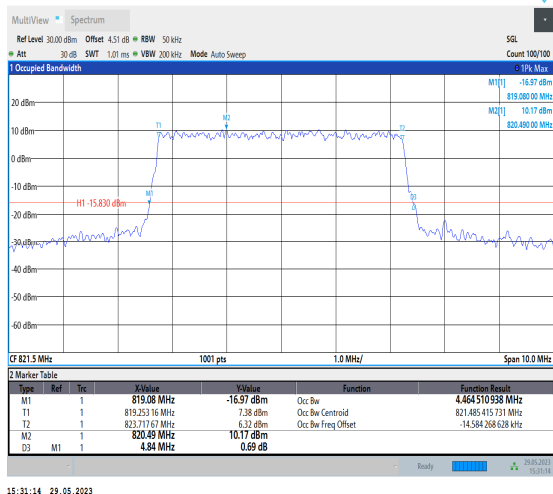
NTNV_N26-814-824_PC3_15_5_H_TID7_Ant1#1
