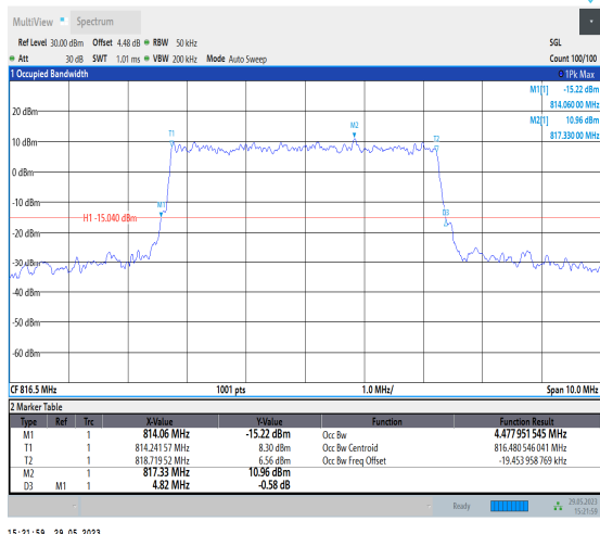
NTNV_N26-814-824_PC3_15_5_L_TID8_Ant1#1
