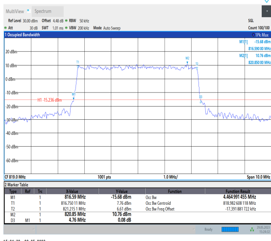
NTNV_N26-814-824_PC3_15_5_M_TID7_Ant1#1
