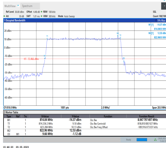
NTNV_N26-814-824_PC3_15_10_M_TID3_Ant1#1
