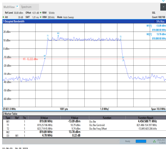
NTNV_N26-814-824_PC3_15_5_H_TID2_Ant1#1
