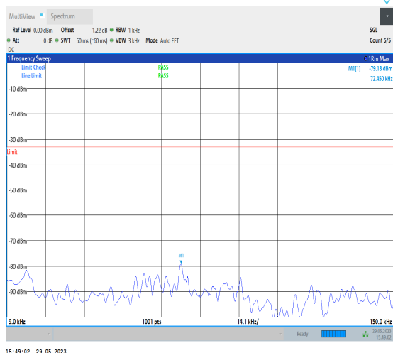
NTNV_N26-814-824_PC3_15_10_M_TID1_N/A_0.009_0.15_#1
