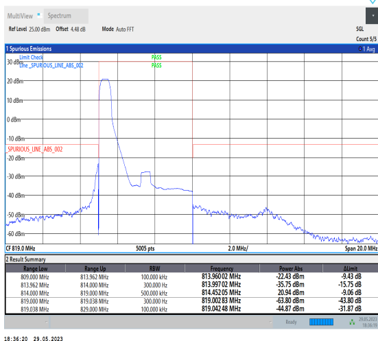
1-N26-814-824-PC3-15-5-L-4-CP-QPSK-Edge_1RB_L_eff-1@0-Ant1-1--PASS-see graph
