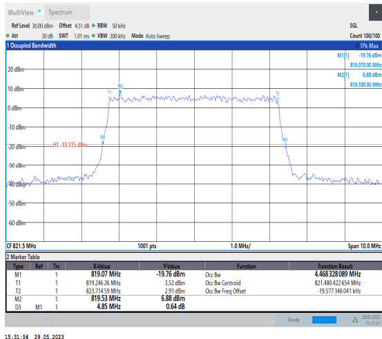
NTNV_N26-814-824_PC3_15_5_H_TID9_Ant1#1
