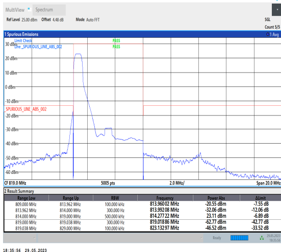
1-N26-814-824-PC3-15-5-L-1-DFT-PI2BPSK-Edge_1R_B_Left-1@0-Ant1-1--PASS-see graph
