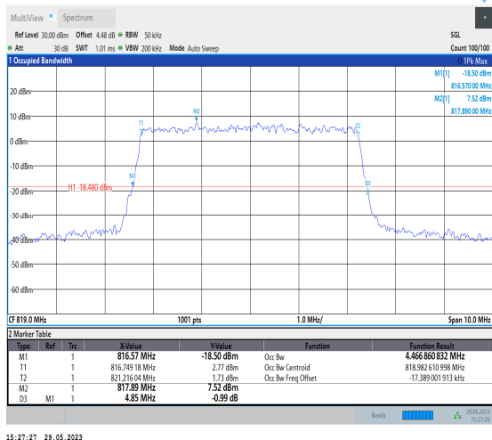
NTNV_N26-814-824_PC3_15_5_M_TID9_Ant1#1
