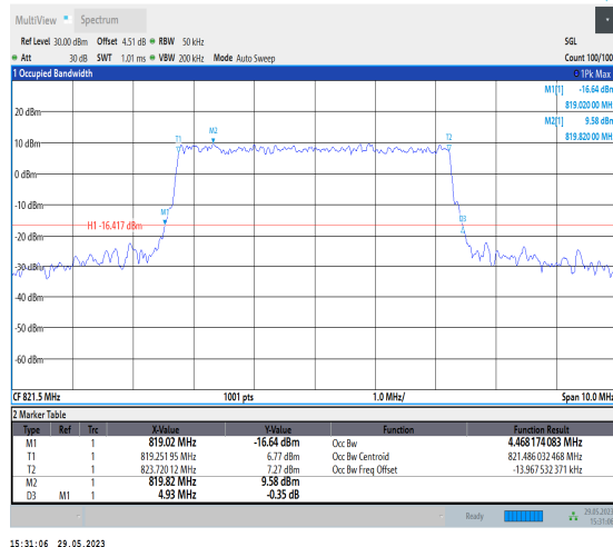
NTNV_N26-814-824_PC3_15_5_H_TID6_Ant1#1
