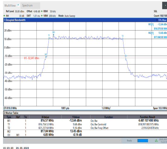
NTNV_N26-814-824_PC3_15_5_M_TID2_Ant1#1
