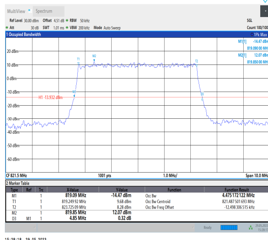
NTNV_N26-814-824_PC3_15_5_H_TID3_Ant1#1
