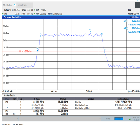
NTNV_N26-814-824_PC3_15_5_M_TID5_Ant1#1
