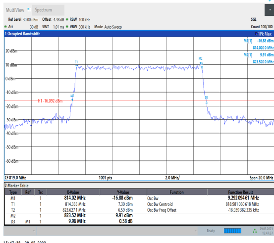
NTNV_N26-814-824_PC3_15_10_M_TID8_Ant1#1
