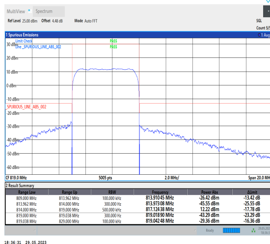
1-N26-814-824-PC3-15-5-L-6-CP-QPSK-Outer_Ful_I-25@0-Ant1-1--PASS-see graph
