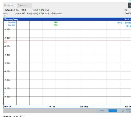
NTNV_N26-814-824_PC3_15_10_M_TID1_N/A_0.15_30_#1
