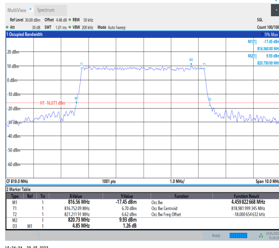
NTNV_N26-814-824_PC3_15_5_M_TID6_Ant1#1
