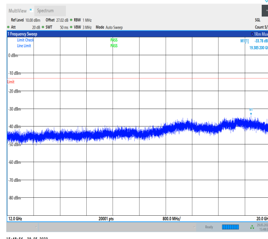
NTNV_N26-814-824_PC3_15_10_L_TID1_N/A_12000_20_000_#1
