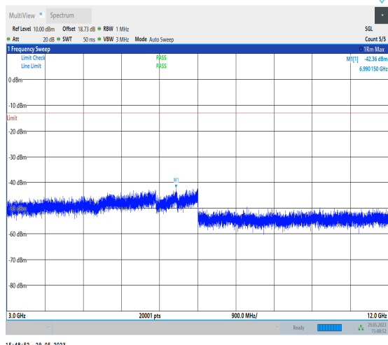
NTNV_N26-814-824_PC3_15_10_L_TID1_N/A_3000_12_000_#1
