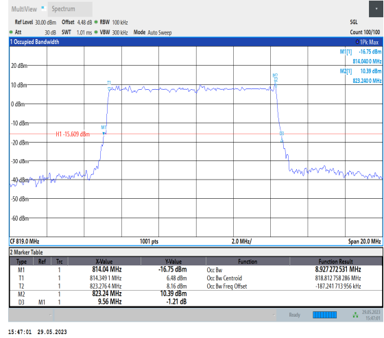
NTVN_N26-814-824_PC3_15_10_M_TID5_Ant1#1
