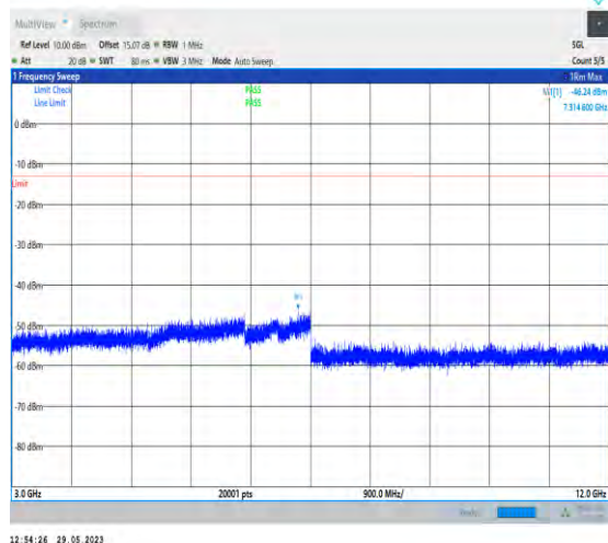
1-N5-PC3-15-20-L-1-N/A-DFT-PI2BPSK-Inner_1RB_Left-1@1-3000-12000-Ant1-7314.60--46.24--13-PASS
