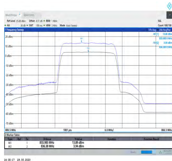
1-N5-PC3-15-20-M-2-CP-256QAM-Outet_Full-106 @0-Ant1-9.95-100%-0.00-9.95-PASS-≤13
