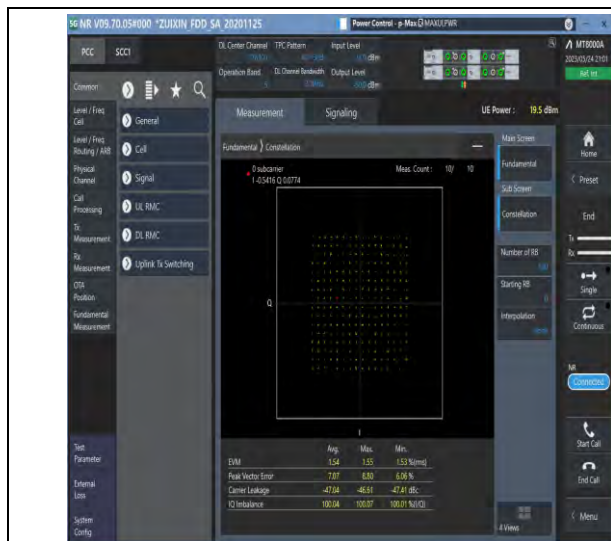
1-N5-PC3-15-20-M-5-DFT-256QAM-Outer_Full-100@0-Ant1-see graph-PASS
