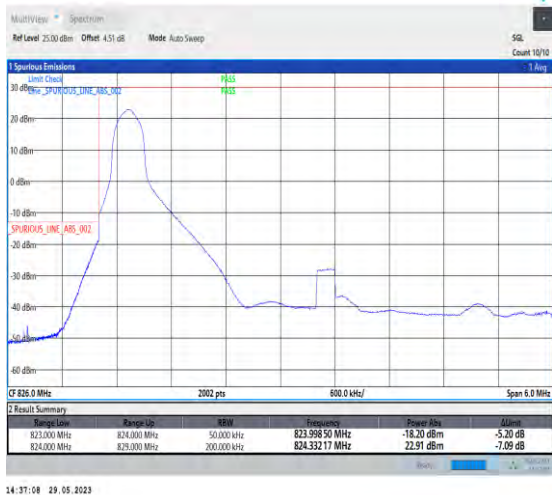
1-N5-PC3-15-5-L-1-DFT-PI2BPSK-Edge_1RB_Left-1@0-Ant1-1-seegraph-PASS-see graph
