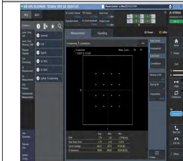
1-N5-PC3-15-20-M-7-CP-16QAM-Outer_Full-106@0-Ant1-see graph-PASS
