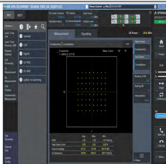
1-N5-PC3-15-20-M-8-CP-64QAM-Outer_Full-106@0-Ant1-see graph-PASS
