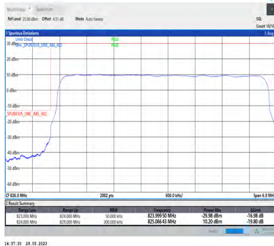
1-N5-PC3-15-5-L-3-DFT-PI2BPSK-Outer_Full-25@0-Ant1-1-seegraph-PASS-see graph
