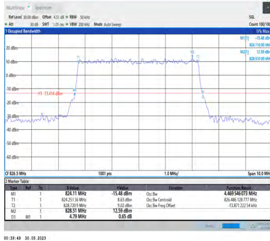
1-N5-PC3-15-5-L-1-DFT-QPSK-Outer_Full-25@0-An t1-4.47-4.790-≤5-PASS
