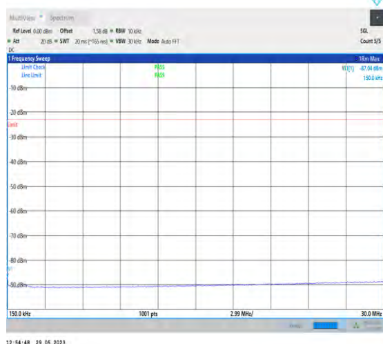
1-N5-PC3-15-20-M-1-N/A-DFT-PI2BPSK-Inner_1RB_Left-1@1-0.15-30-Ant1-0.15--87.04--23-PASS
