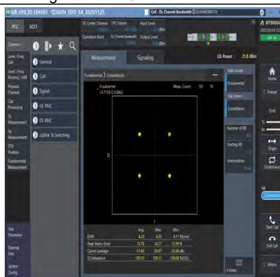
1-N5-PC3-15-20-M-6-CP-QPSK-Outer_Full-106@0-Ant1-see graph-PASS
