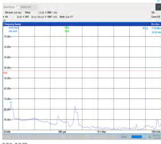
1-N2-PC3-15-20-H-1-N/A-DFT-PI2BPSK-Inner_1RB _Left-1@1-0.009-0.15-Ant1-0.02--77.04--43-PASS
