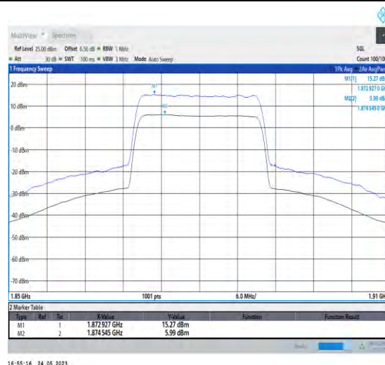
1-N2-PC3-15-20-M-2-CP-256QAM-Outter_Full-106 @0-Ant1-9.28-100%-0.00-9.28-PASS-≤13
