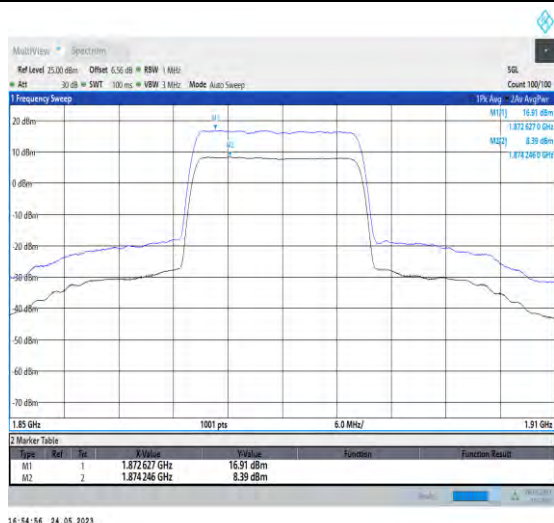
1-N2-PC3-15-20-M-1-DFT-256QAM-Outter_Full-100 @0-Ant1-8.52-100%-0.00-8.52-PASS-≤13
