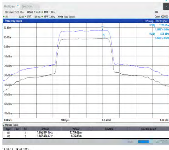
1-N2-PC3-15-20-L-1-DFT-256QAM-Outter_Full-100@ 0-Ant1-8.43-100%-0.00-8.43-PASS-≤13
