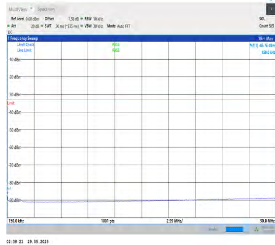
1-N2-PC3-15-20-L-1-N/A-DFT-PI2BPSK-Inner_1RB_ Left-1@1-0.15-30-Ant1-0.15--86.76--33-PASS
