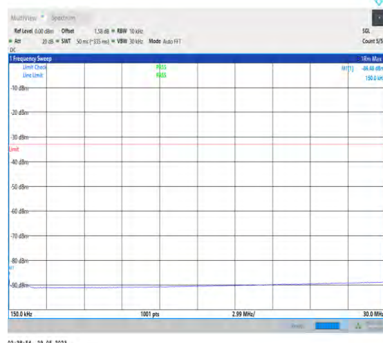
1-N2-PC3-15-20-M-1-N/A-DFT-PI2BPSK-Inner_1RB_ Left-1@1-0.15-30-Ant1-0.15--86.48--33-PASS
