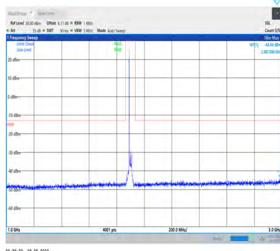
1-N2-PC3-15-20-H-1-N/A-DFT-PI2BPSK-Inner_1RB_ Left-1@1-1000-3000-Ant1-2982.50--43.44--13-PASS
