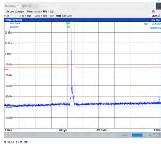
1-N2-PC3-15-20-L-1-N/A-DFT-PI2BPSK-Inner_1RB_ Left-1@1-1000-3000-Ant1-2973.00--44.21--13-PASS
