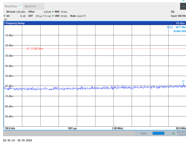
Band26-15MHz-QPSK-26865-1RB#0-Range2:0.15~30MHz
