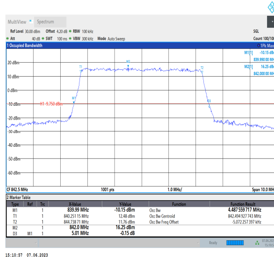
Band19-5MHz-64QAM-24125-25RB#0
