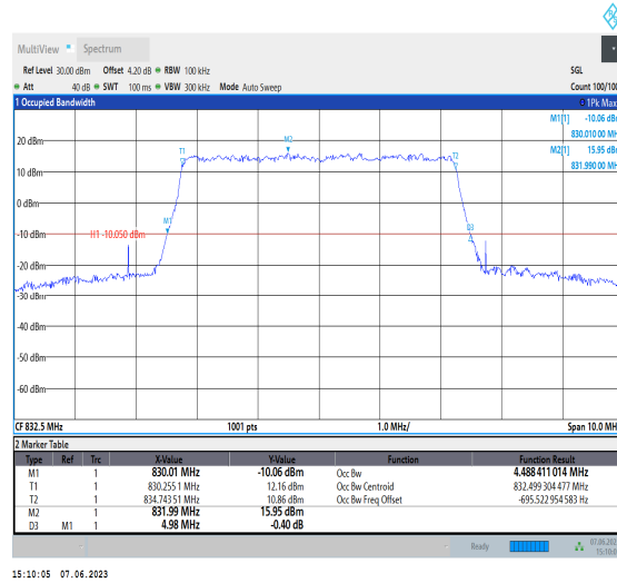
Band19-5MHz-64QAM-24025-25RB#0
