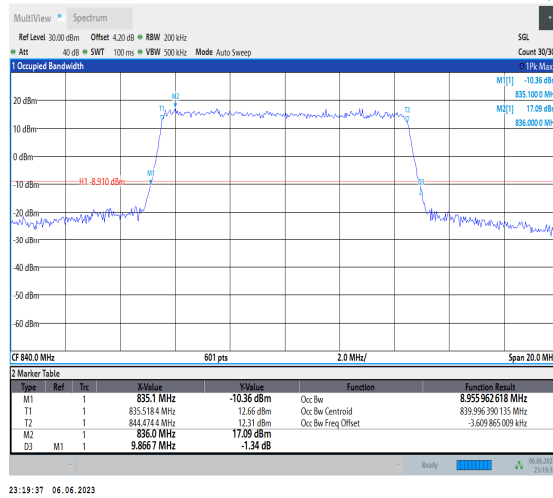
Band19-10MHz-16QAM-24100-50RB#0
