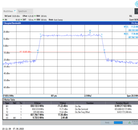
Band19-10MHz-64QAM-24050-50RB#0
