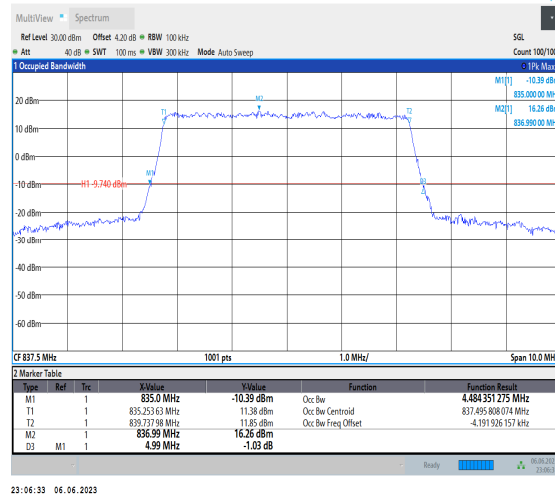
Band19-5MHz-16QAM-24075-25RB#0
