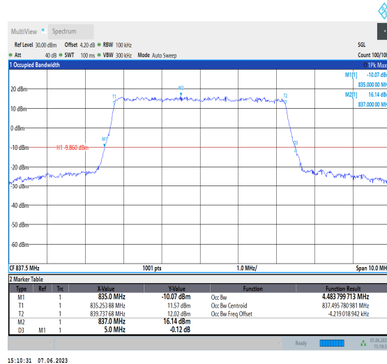
Band19-5MHz-64QAM-24075-25RB#0
