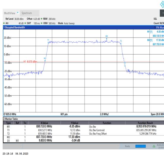
Band19-10MHz-16QAM-24050-50RB#0
