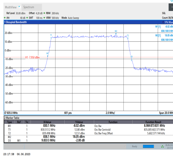
Band19-10MHz-QPSK-24050-50RB#0
