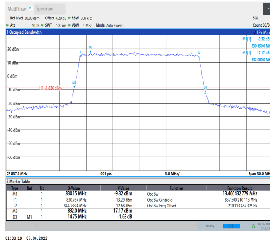
Band19-15MHz-QPSK-24075-75RB#0
