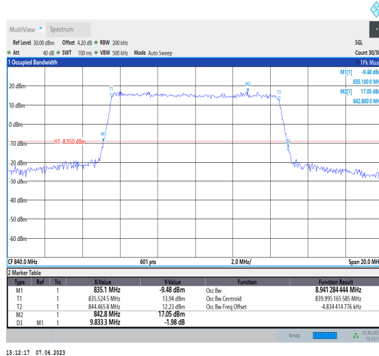
Band19-10MHz-64QAM-24100-50RB#0
