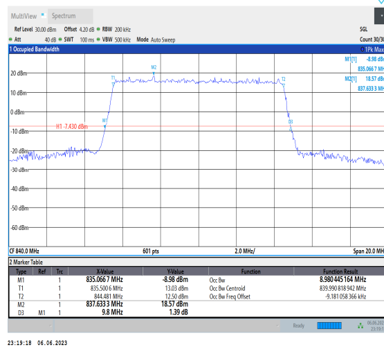
Band19-10MHz-QPSK-24100-50RB#
