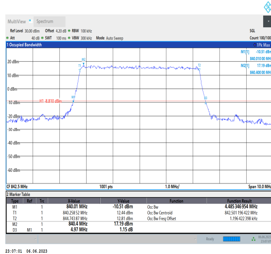
Band19-5MHz-QPSK-24125-25RB#0
