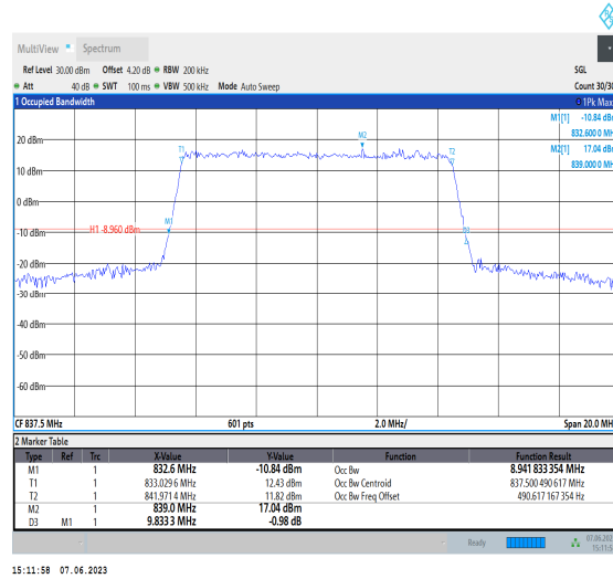
Band19-10MHz-64QAM-24075-50RB#0
