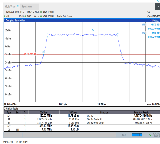
Band19-5MHz-16QAM-24025-25RB#0
