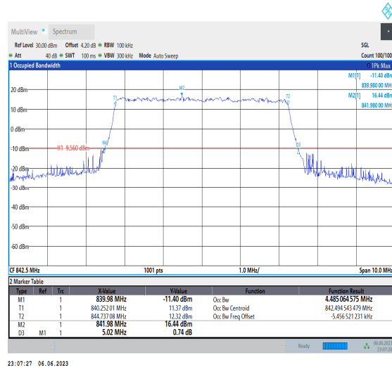
Band19-5MHz-16QAM-24125-25RB#0
