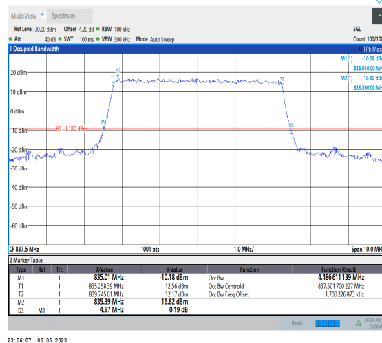
Band19-5MHz-QPSK-24075-25RB#0
