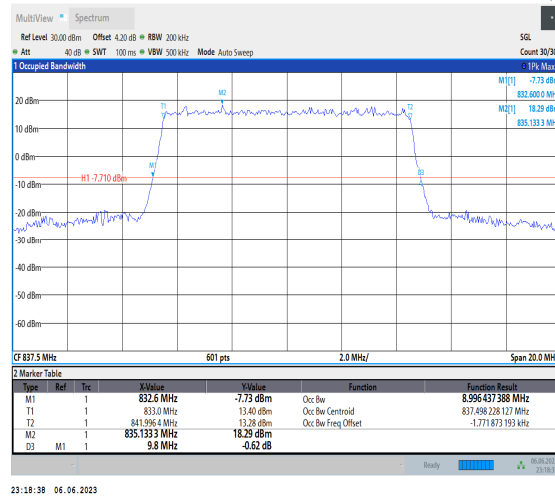
Band19-10MHz-QPSK-24075-50RB#0
