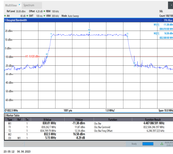
Band19-5MHz-QPSK-24025-25RB#0
