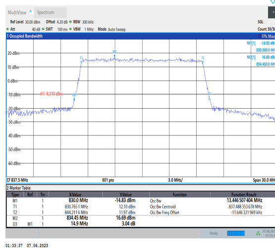
Band19-15MHz-16QAM-24075-75RB#0
