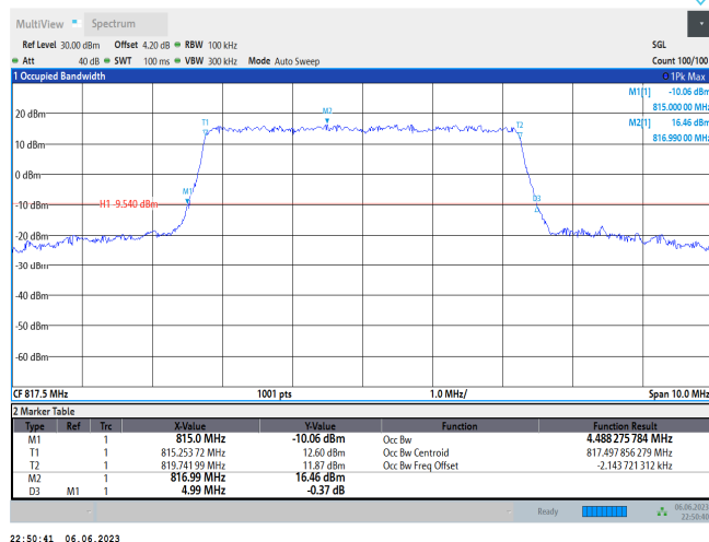
Band18(815-824)-5MHz-16QAM-23875-25RB#0
