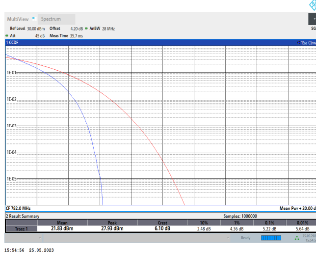
Band13-10MHz-16QAM-23230-50RB#0
