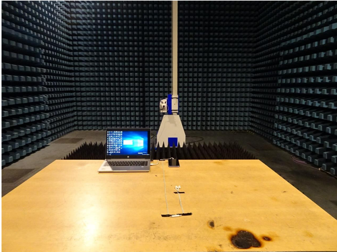
FCC Part15B Radiated Emission 18GHz-26.5GHz -Front
