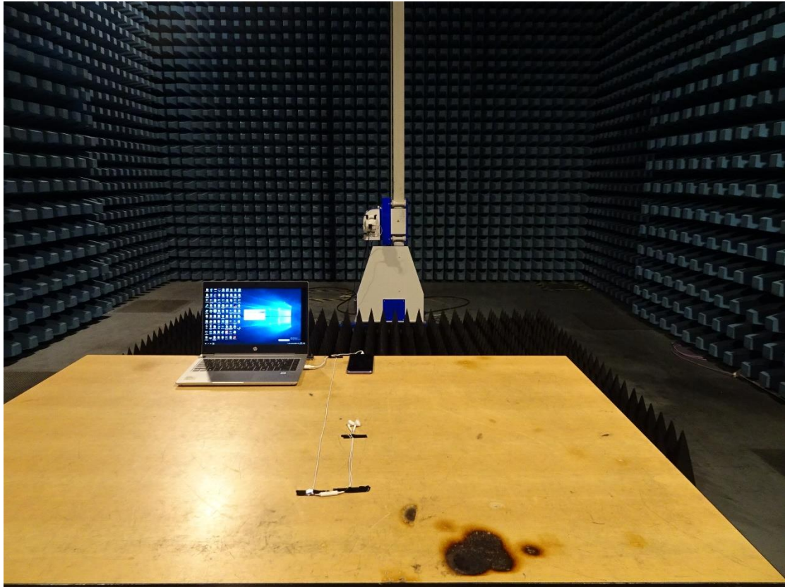
FCC Part15B Radiated Emission 26.5GHz-40GHz -Front
