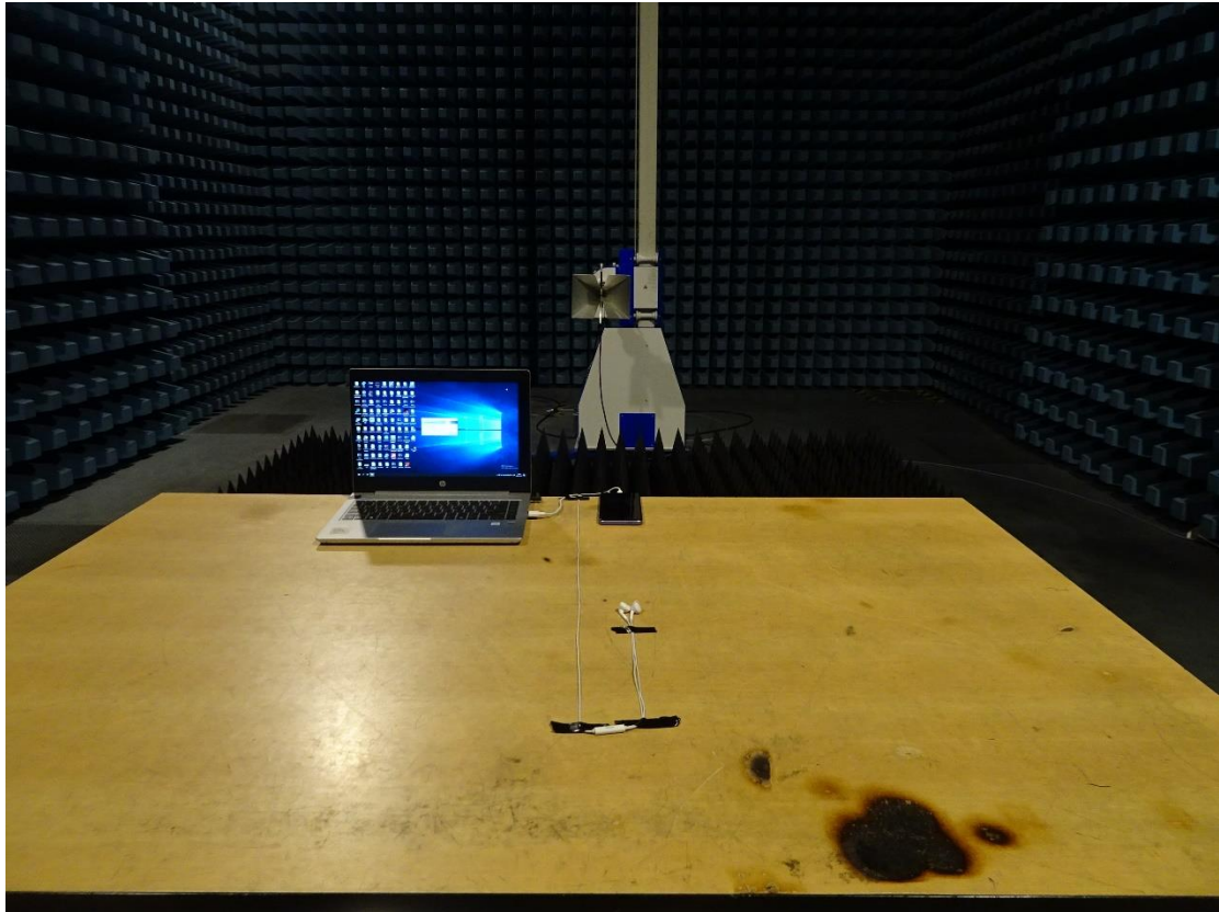
FCC Part15B Radiated Emission 1GHz-18GHz -Front
