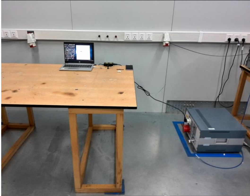
AC Conducted Emission Test Setup -Front
