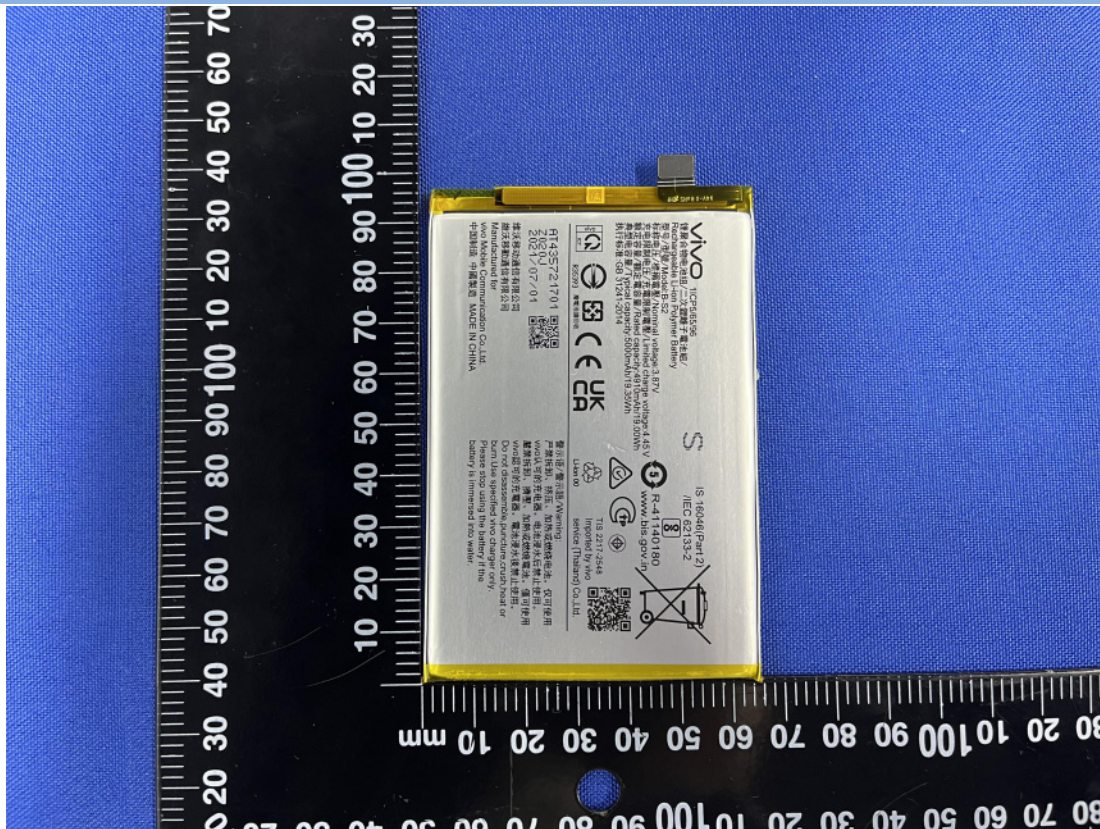
Battery Photo(REAR)
