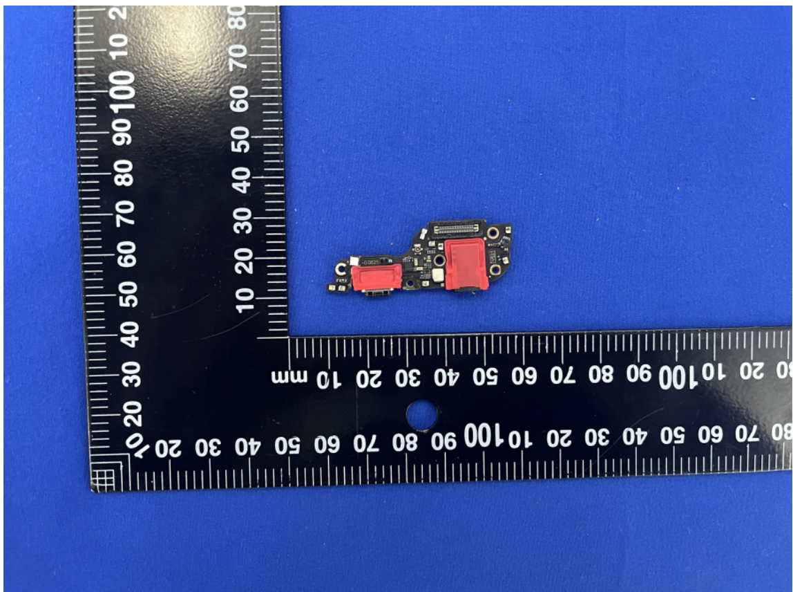
SUB BOARD REAR VIEW (WITH SHIELDING)
