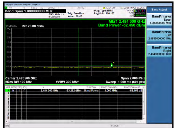
802.11n-20 MHz CHANNEL 10, Reference level
