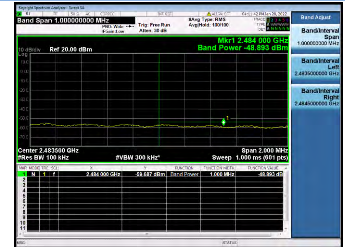
802.11g CHANNEL 11, Reference level
