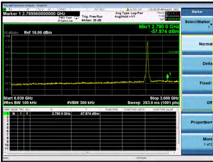
802.11n-20 CHANNEL 6, SPURIOUS 30 MHz ~ 3 GHz
