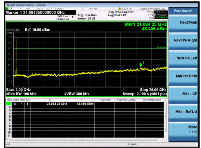
802.11n-20 CHANNEL 6, SPURIOUS 2 GHz ~ 25 GHz
