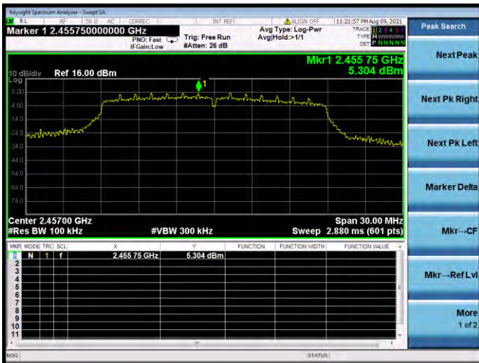
802.11n-20 CHANNEL 10 CARRIER LEVEL
