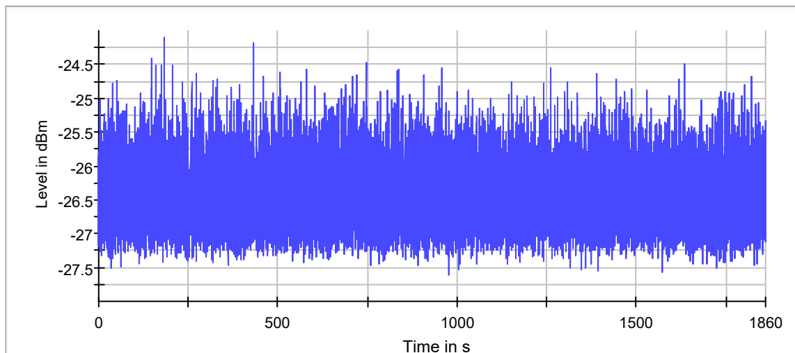
802.11a Channel 100
