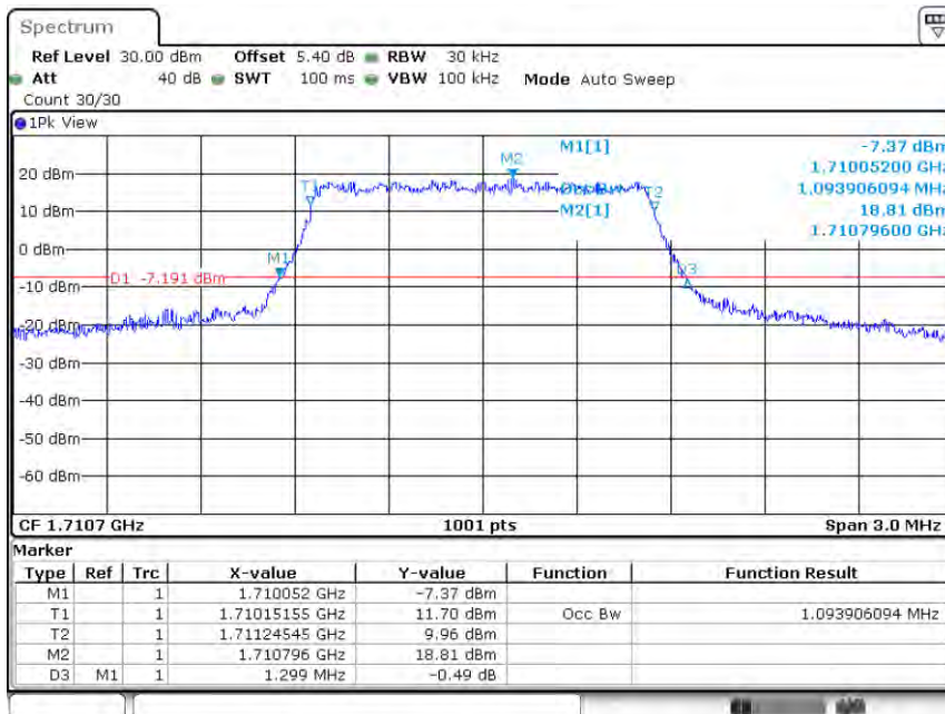
Band4-1.4MHz-QPSK-19957-6RB#0-1.094
