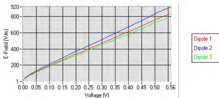
Calibration curves
