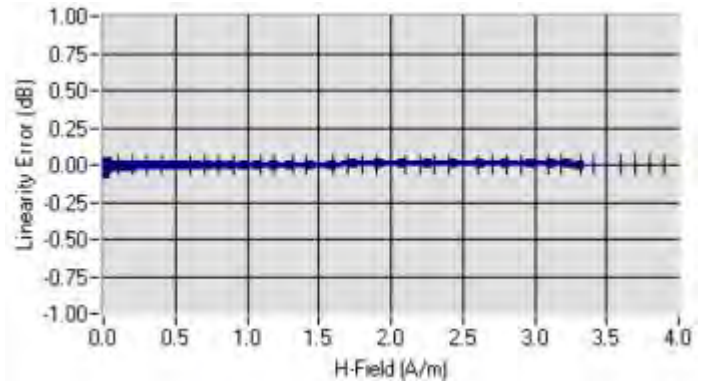
Linearity @ 1900MHz
