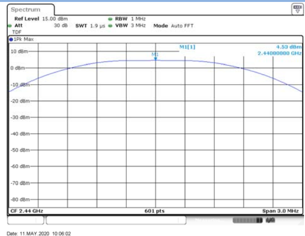
GFSK (BLE 1Mbps) MIDDLE CHANNEL
