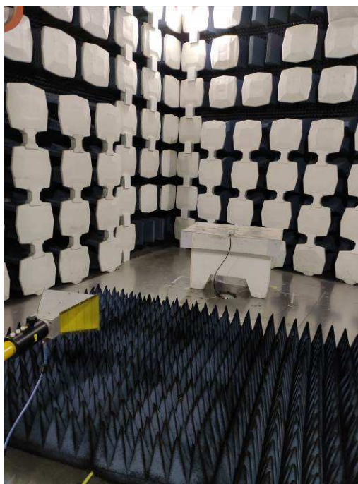
(2) Radiated spurious emission Test Setup(Above 1GHz)
