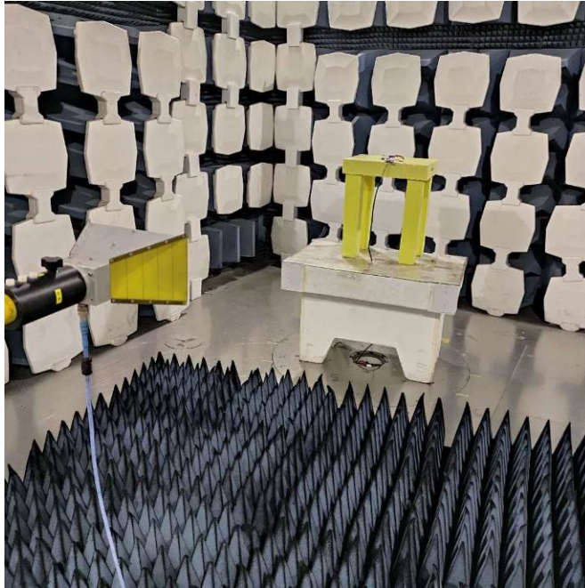
(3) Radiated spurious emission Test Setup-3(Above 1GHz)
