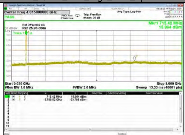
B17_QPSK_10M_High_CDT_Spurious
