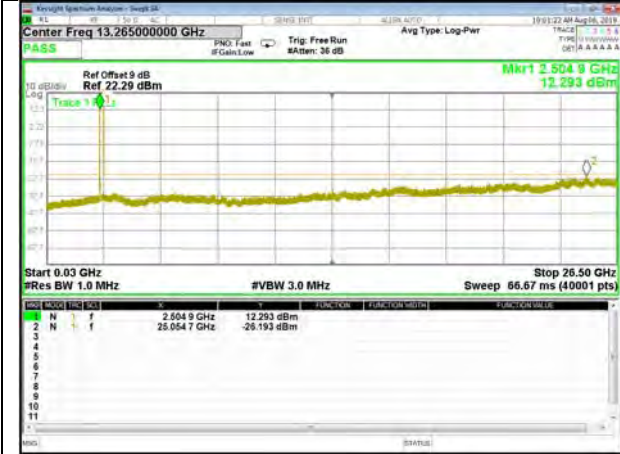
B41_QPSK_10M_Mid_CDT_Spurious
