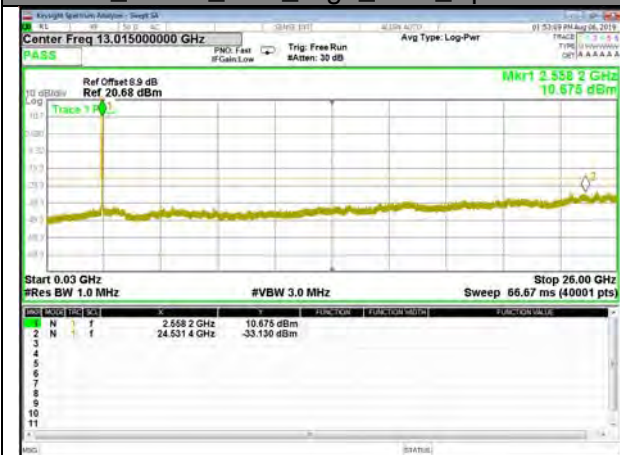
B7_QPSK_15M_High_CDT_Spurious
