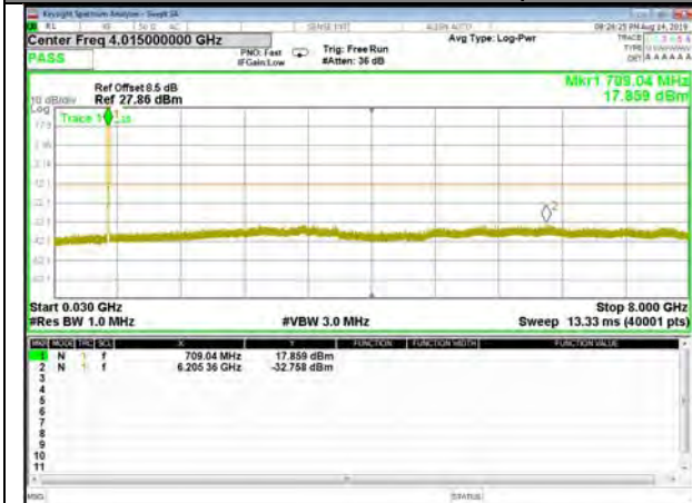
B17_QPSK_5M_High_CDT_Spurious
