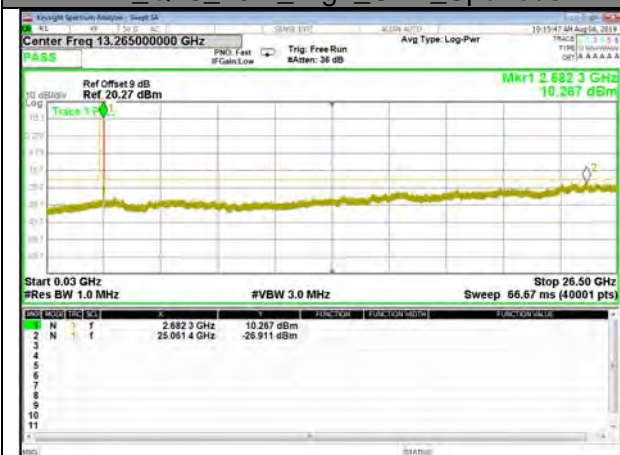
B41_Q16_15M_High_CDT_Spurious
