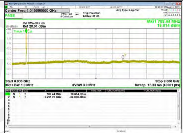
B17_Q16_5M_High_CDT_Spurious
