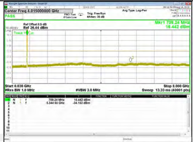
B17_QPSK_10M_Mid_CDT_Spurious
