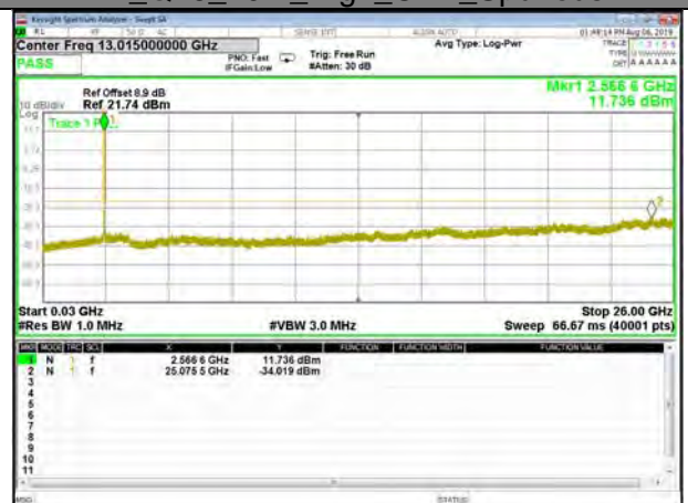
B7_Q16_10M_High_CDT_Spurious
