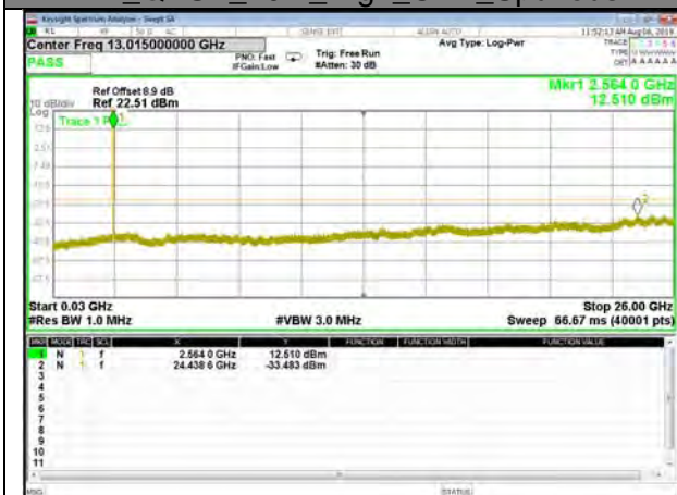
B7_QPSK_10M_High_CDT_Spurious
