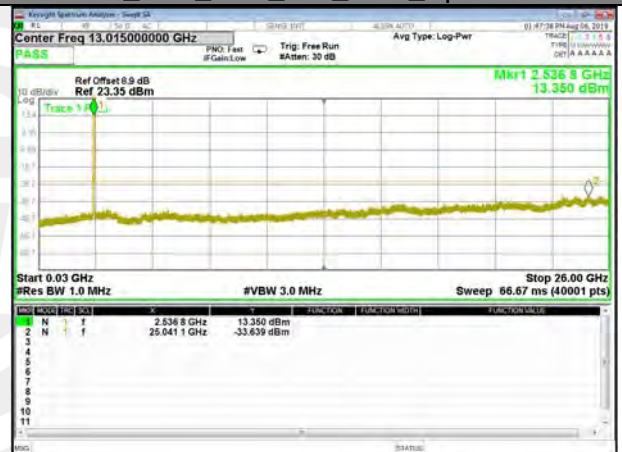
B7_Q16_10M_High_CDT_Spurious
