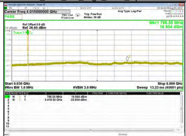
B13_Q16_5M_High_CDT_Spurious
