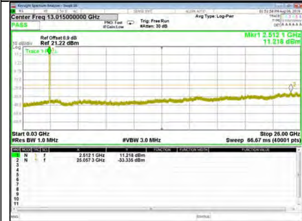
B7_QPSK_15M_Mid_CDT_Spurious
