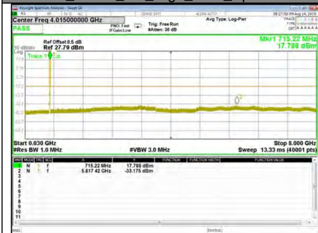
B17_QPSK_5M_High_CDT_Spurious
