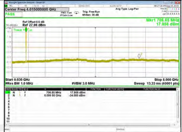
B17_Q16_5M_Mid_CDT_Spurious
