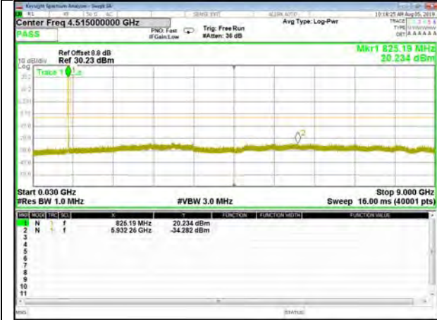
B5_QPSK_1.4M_Mid_CDT_Spurious
