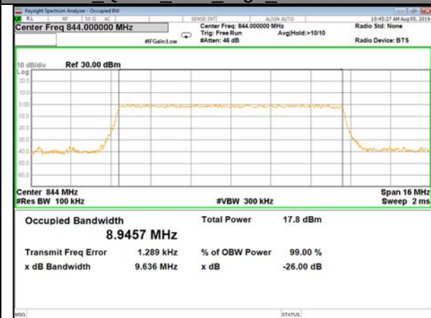
B5_QPSK_10M_High_26BW-99%
