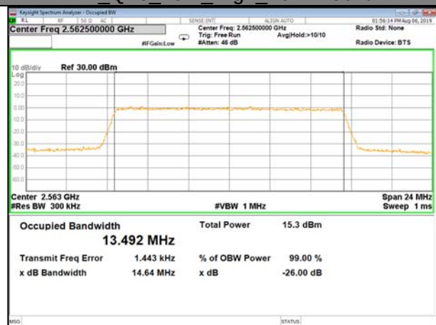
B7_Q16_15M_High_26BW-99%
