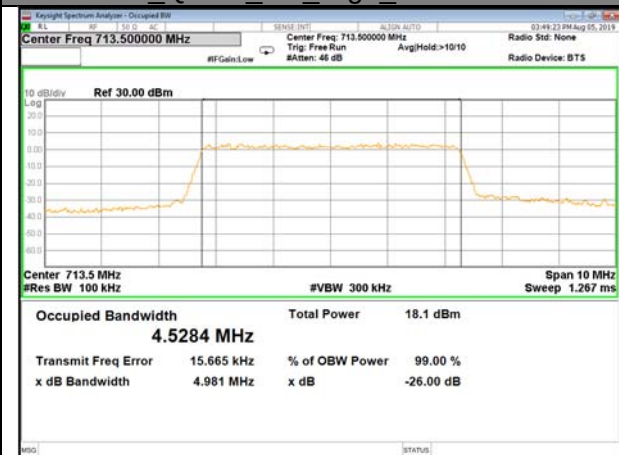
B17_QPSK_5M_High_26BW-99%
