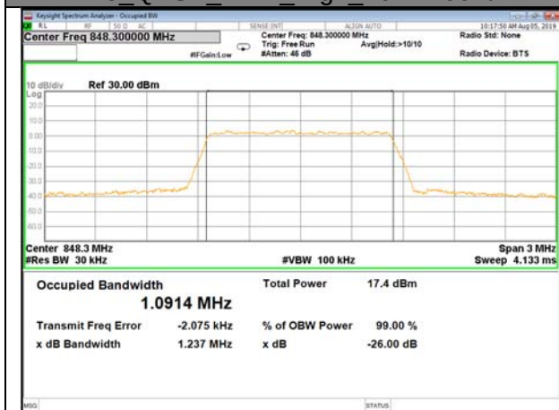
B5_QPSK_1.4M_High_26BW-99%
