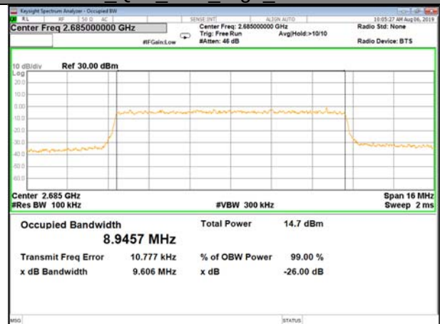
B41_Q16_10M_High_26BW-99%
