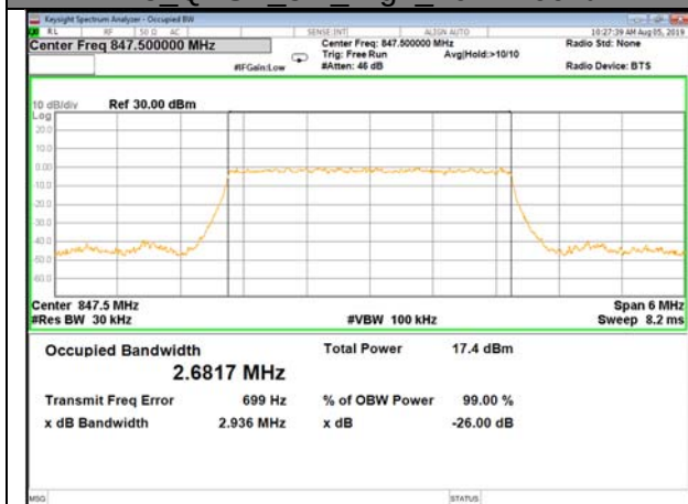
B5_QPSK_3M_High_26BW-99%
