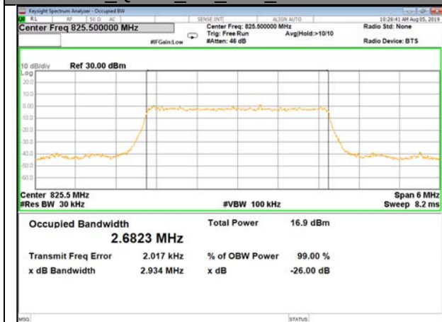
B5_QPSK_3M_Mid_26BW-99%
