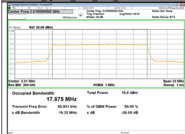
B7_QPSK_20M_Mid_26BW-99%
