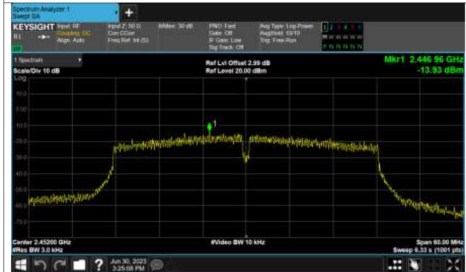
PSD NVNT n40 2452MHz Ant2
