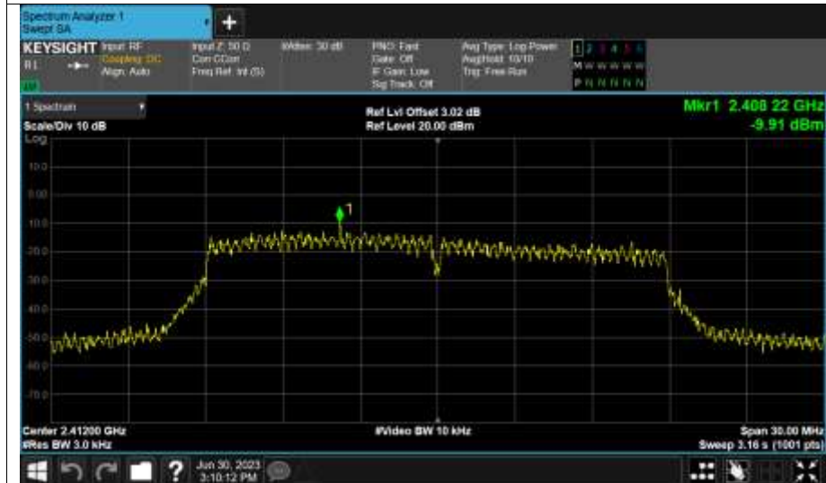
PSD NVNT n20 2412MHz Ant2
