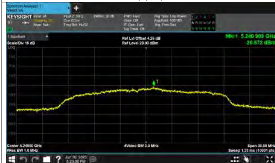
PSD NVNT n20 5240MHz Ant2
