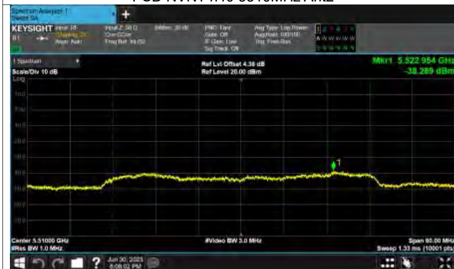
PSD NVNT n40 5510MHz Ant2
