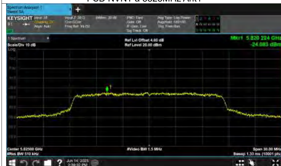
PSD NVNT a 5825MHz Ant1
