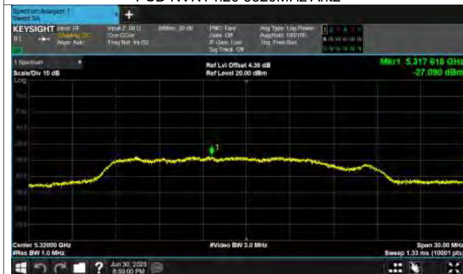
PSD NVNT n20 5320MHz Ant2
