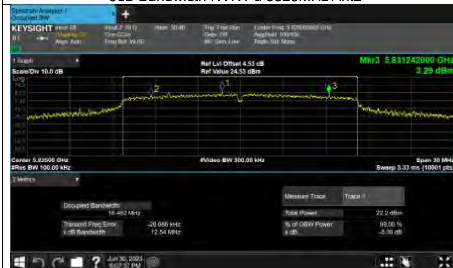
-6dB Bandwidth NVNT a 5825MHz Ant2
