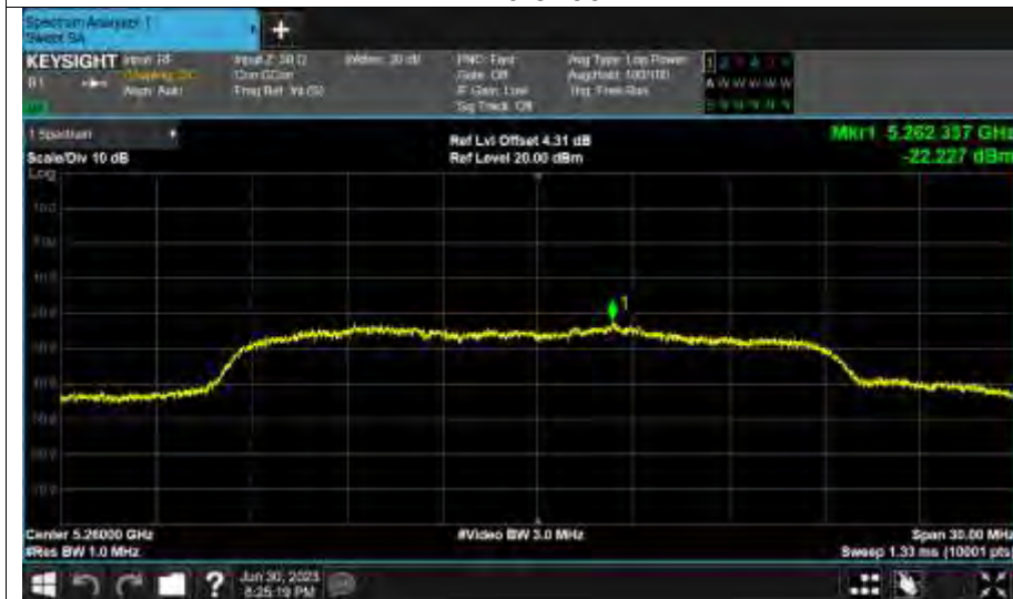
PSD NVNT n20 5260MHz Ant2
