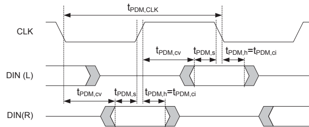
Figure 45: PDM timing diagram
