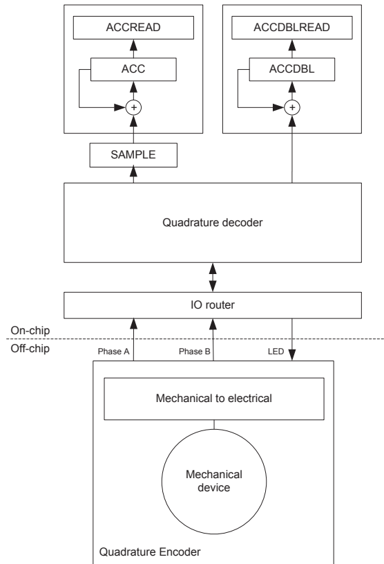
Figure 56: Quadrature decoder configuration
