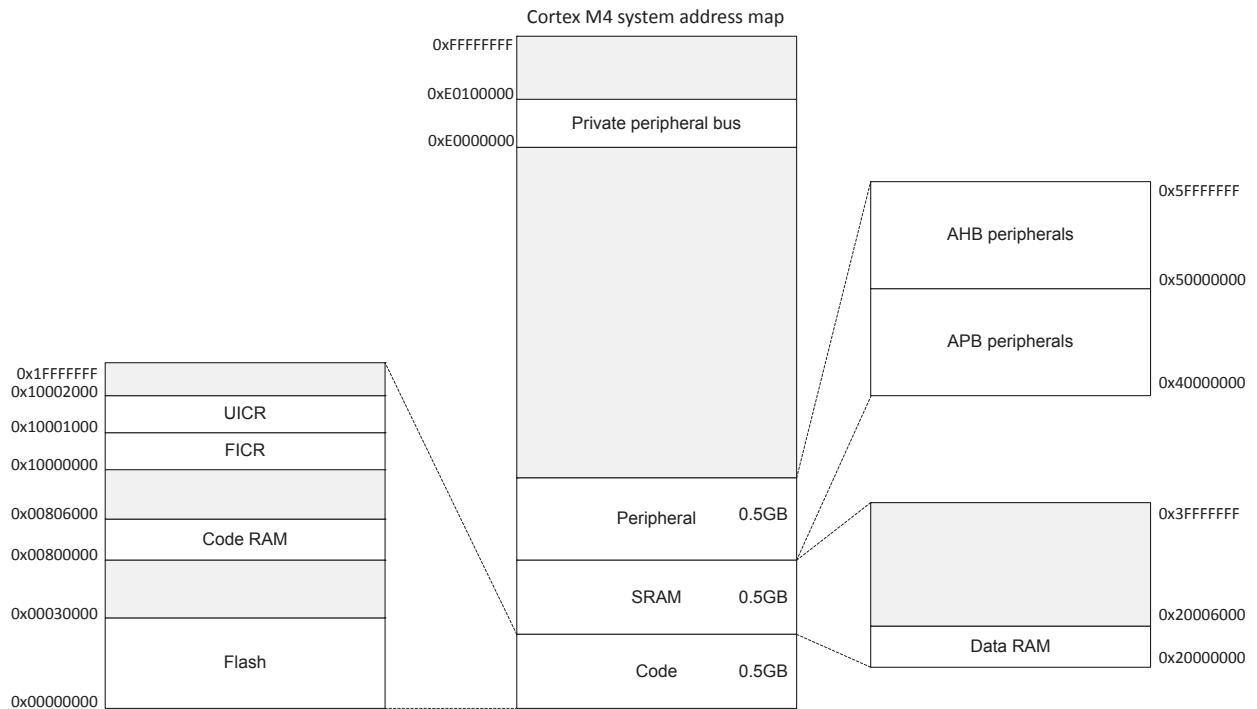
Figure 3: Memory map
