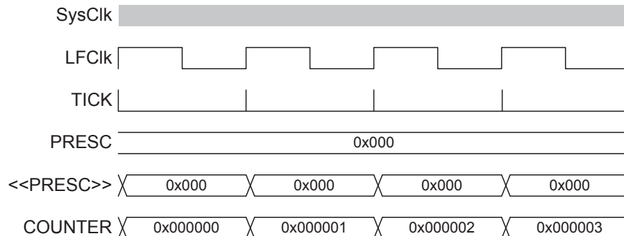
Figure 76: Timing diagram - COUNTER_PRESCALER_0
