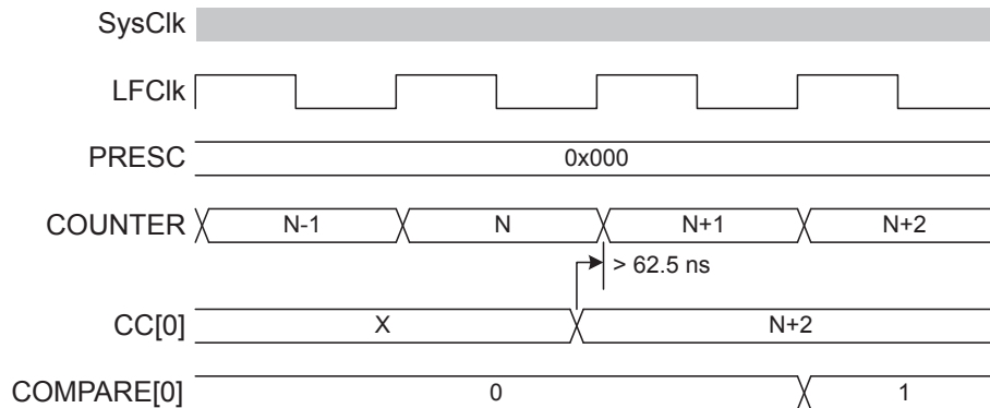
Figure 82: Timing diagram - COMPARE_N+2
