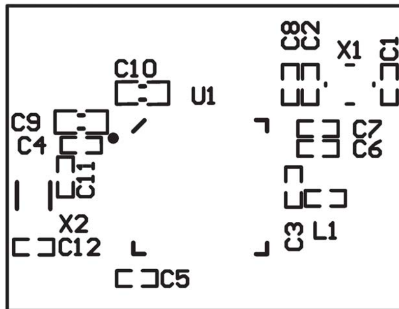
Figure 133: Top silk layer
