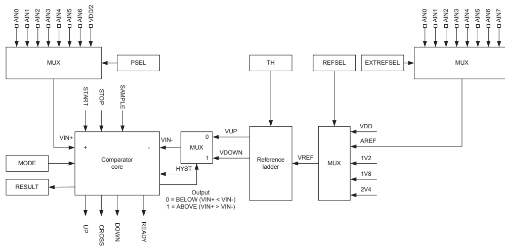
Figure 36: Comparator in single-ended mode
