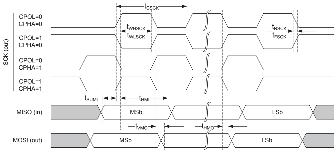
Figure 100: SPIM timing diagram
