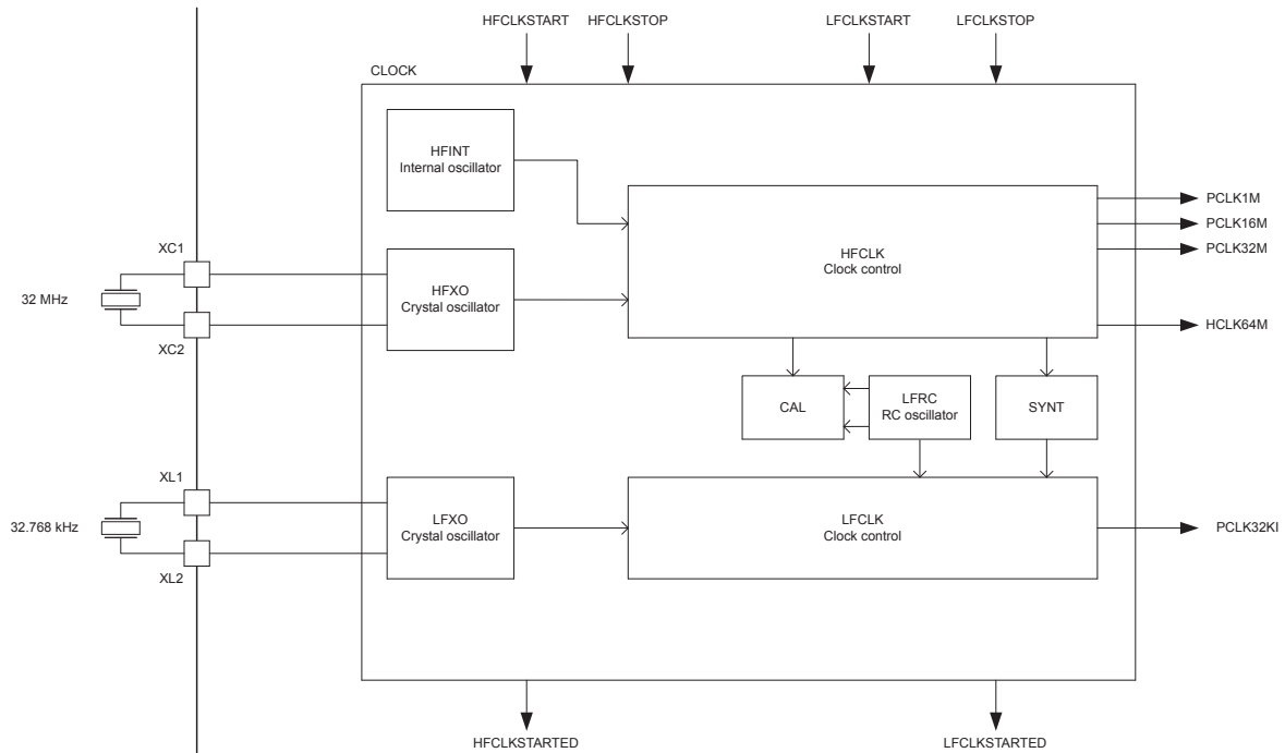
Figure 17: Clock control
