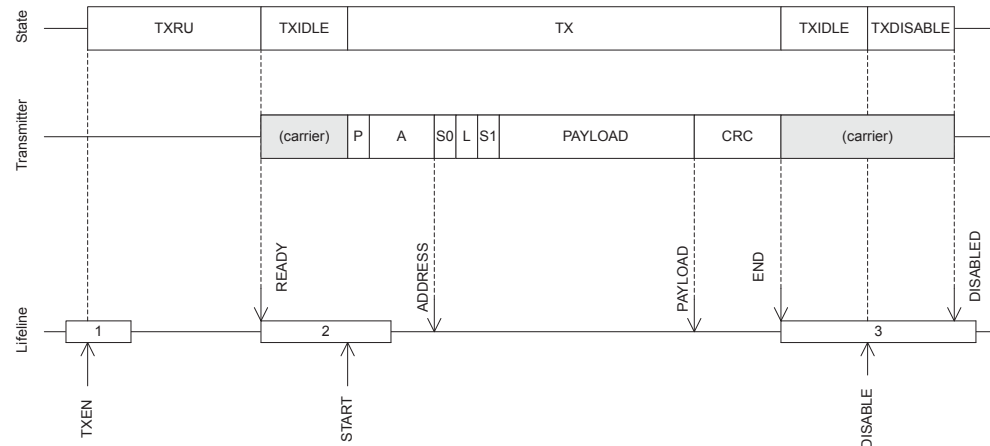
Figure 63: Transmit sequence
