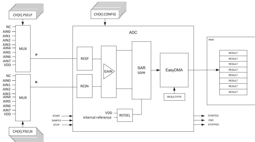
Figure 90: Simplified ADC block diagram
