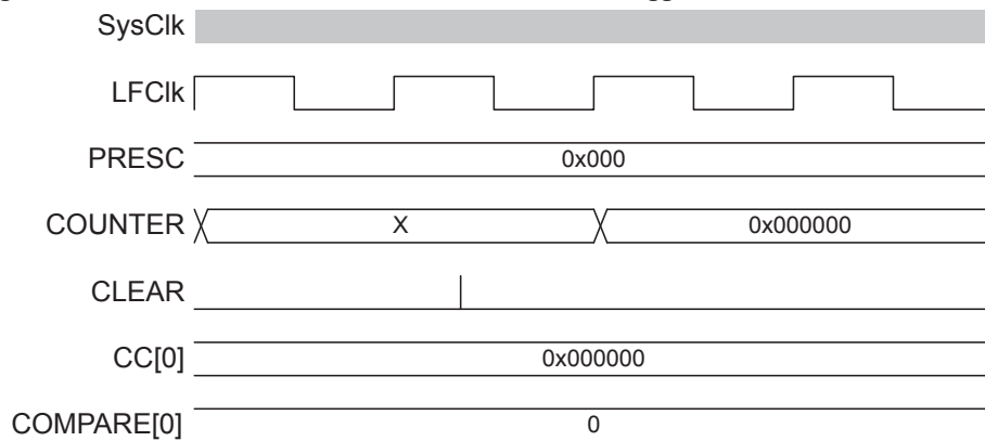
Figure 79: Timing diagram - COMPARE_CLEAR
