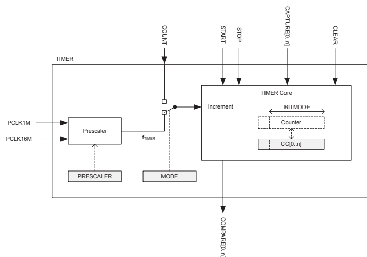
Figure 105: Block schematic for timer/counter
