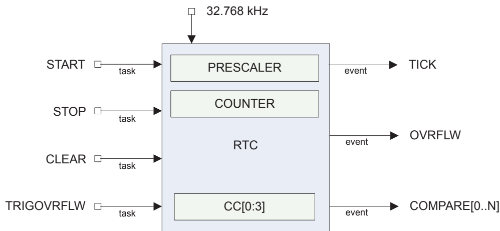
Figure 75: RTC block schematic
