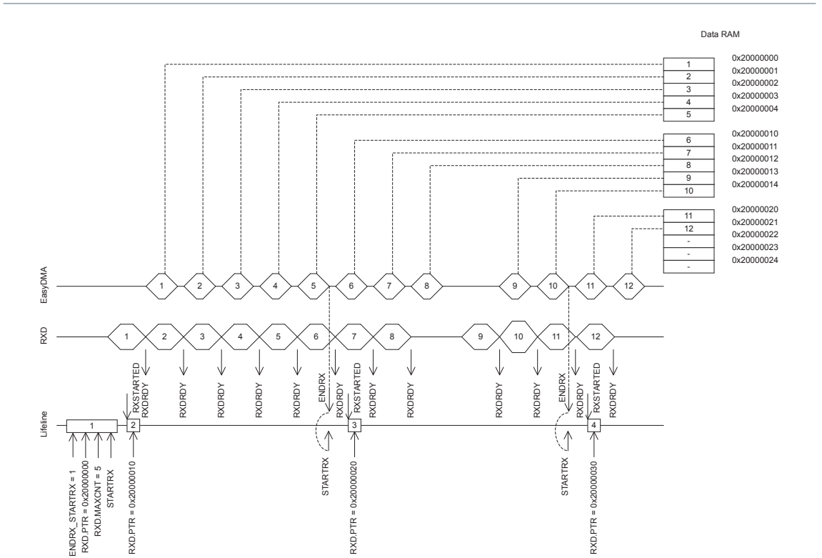
Figure 123: UARTE reception
