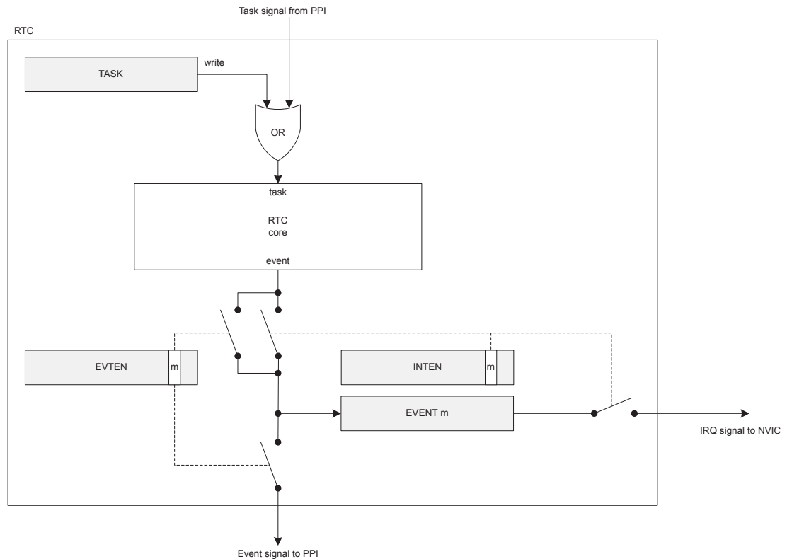
Figure 78: Tasks, events and interrupts in the RTC
