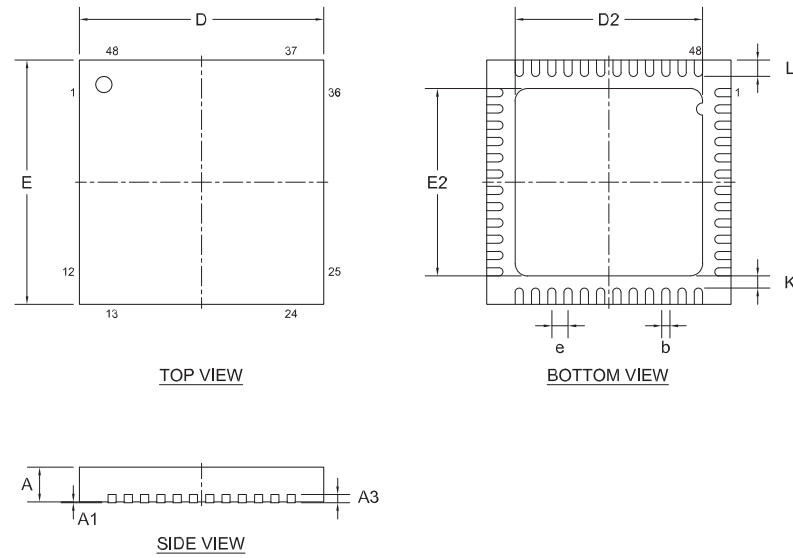
Figure 127: QFN48 6 x 6 mm package
