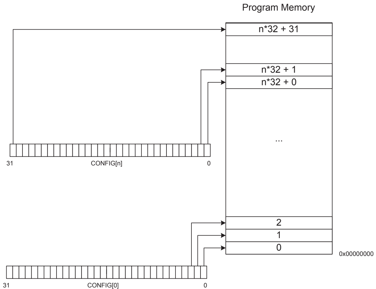
Figure 25: Protected regions of program memory
