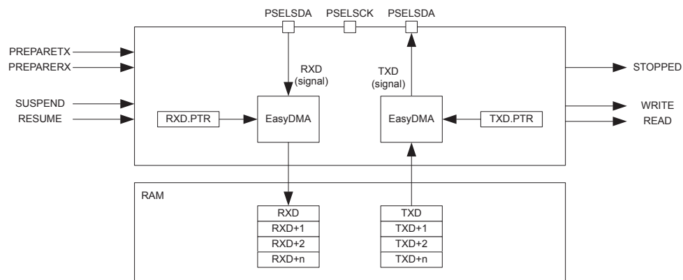
Figure 114: TWI slave with EasyDMA
