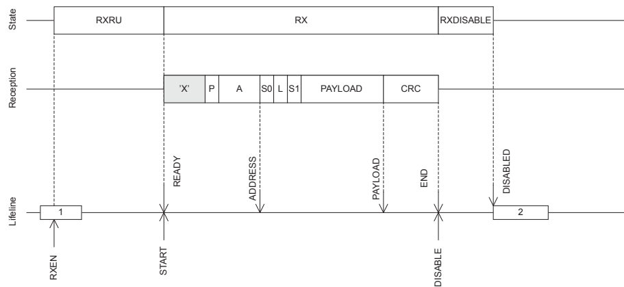
Figure 67: Receive sequence using shortcuts to avoid delays
