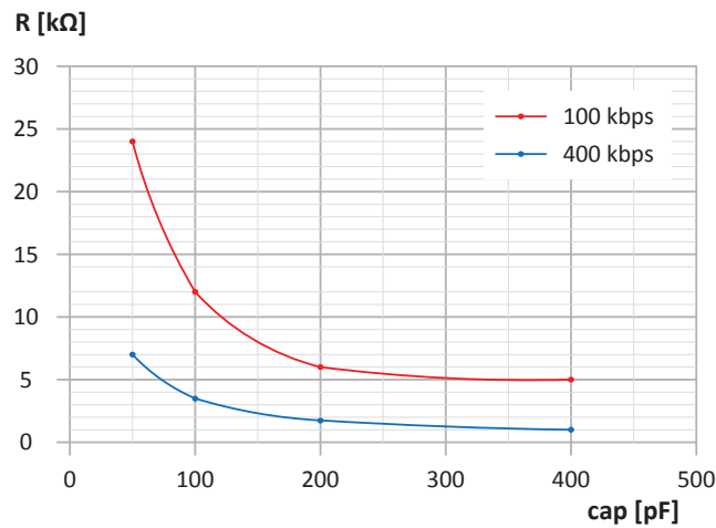
Figure 113: Recommended TWIM pullup value vs. line capacitance
