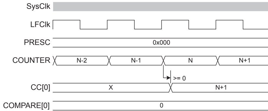
Figure 83: Timing diagram - COMPARE_N+1
