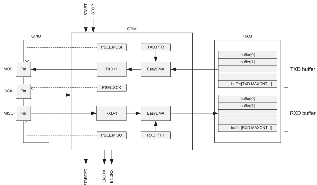
Figure 97: SPIM — SPI master with EasyDMA
