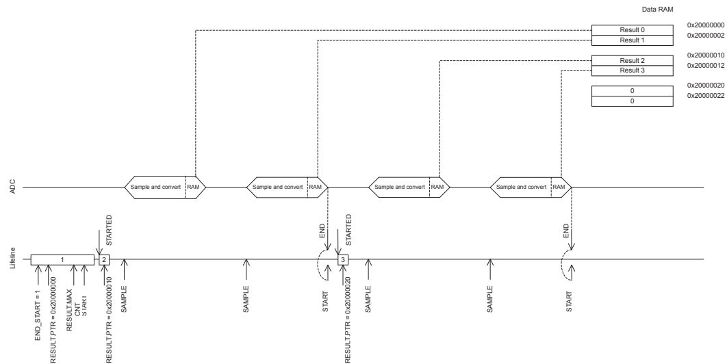
Figure 93: ADC
