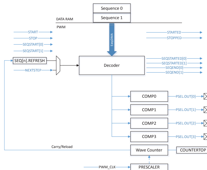
Figure 47: PWM module
