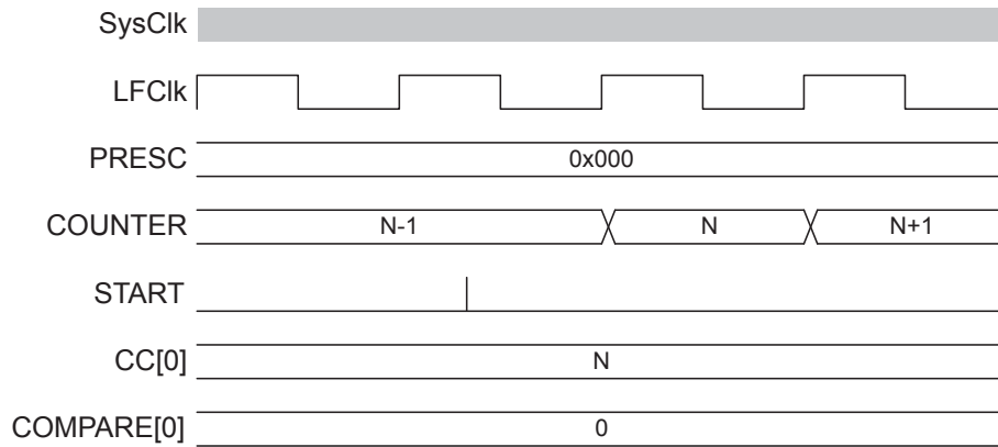
Figure 80: Timing diagram - COMPARE_START
