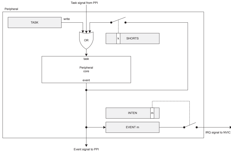
Figure 21: Tasks, events, shortcuts, and interrupts
