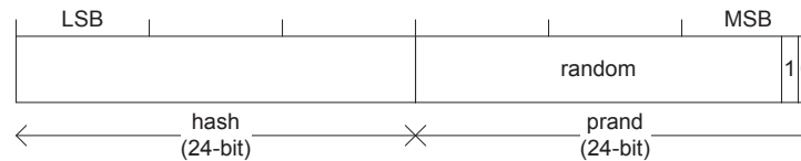
Figure 22: Resolvable address
