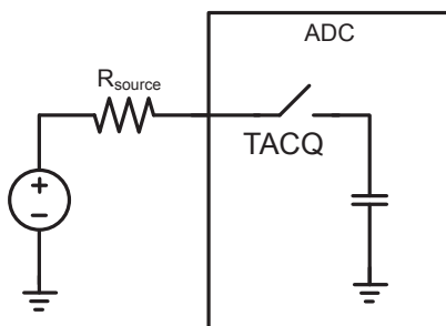
Figure 95: Simplified ADC sample network
