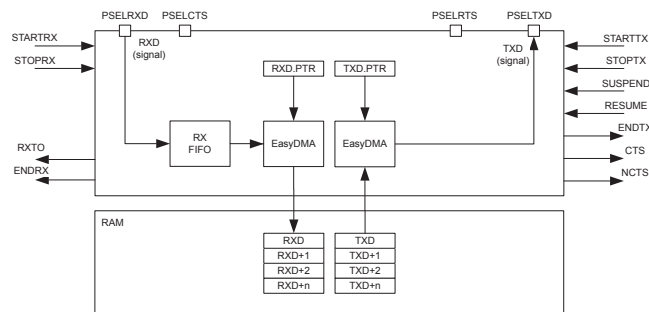
Figure 121: UARTE configuration
