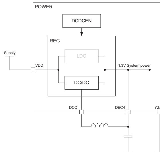
Figure 14: DC/DC regulator setup
