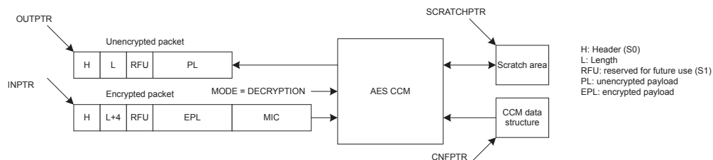
Figure 28: Decryption
