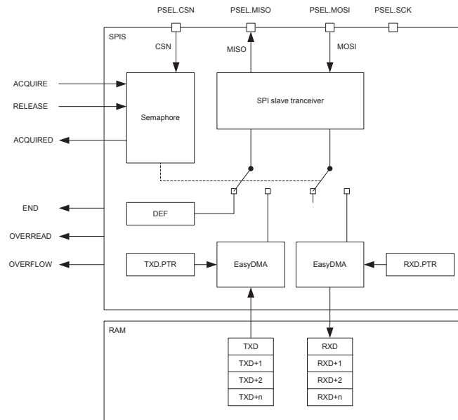
Figure 101: SPI slave
