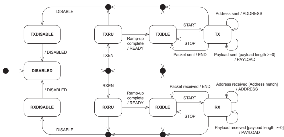
Figure 62: Radio states
