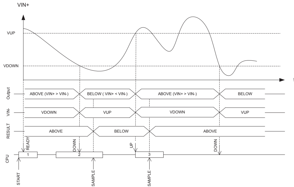
Figure 38: Hysteresis example where VIN+ starts above VUP
