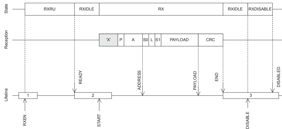
Figure 66: Receive sequence
