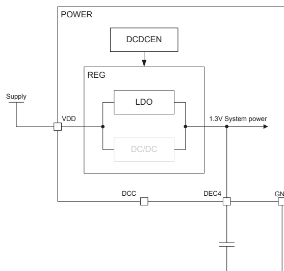
Figure 13: LDO regulator setup
