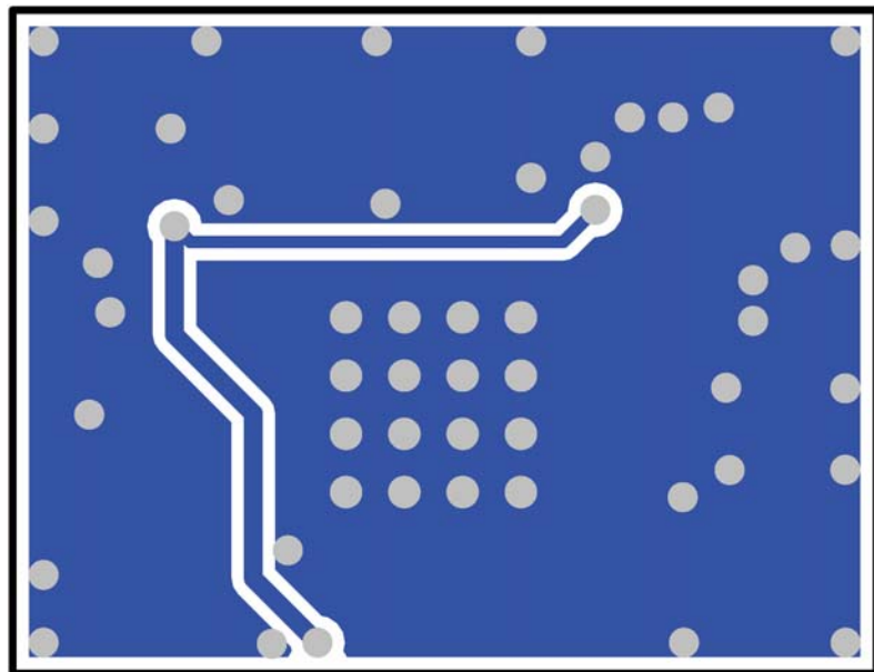
Figure 135: Bottom layer
