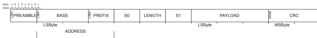
Figure 58: On-air packet layout
