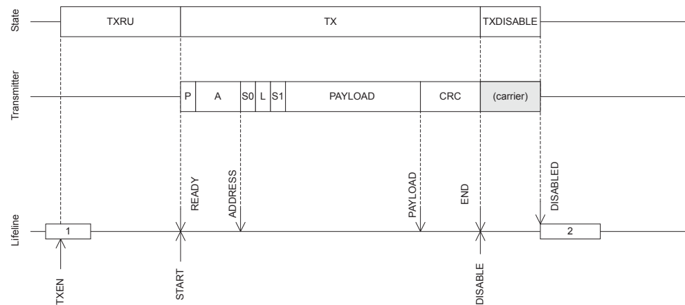
Figure 64: Transmit sequence using shortcuts to avoid delays
