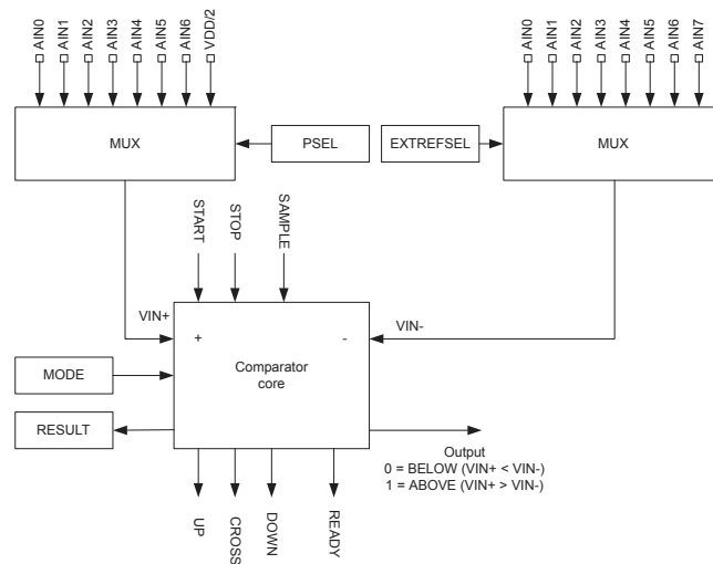
Figure 34: Comparator in differential mode
