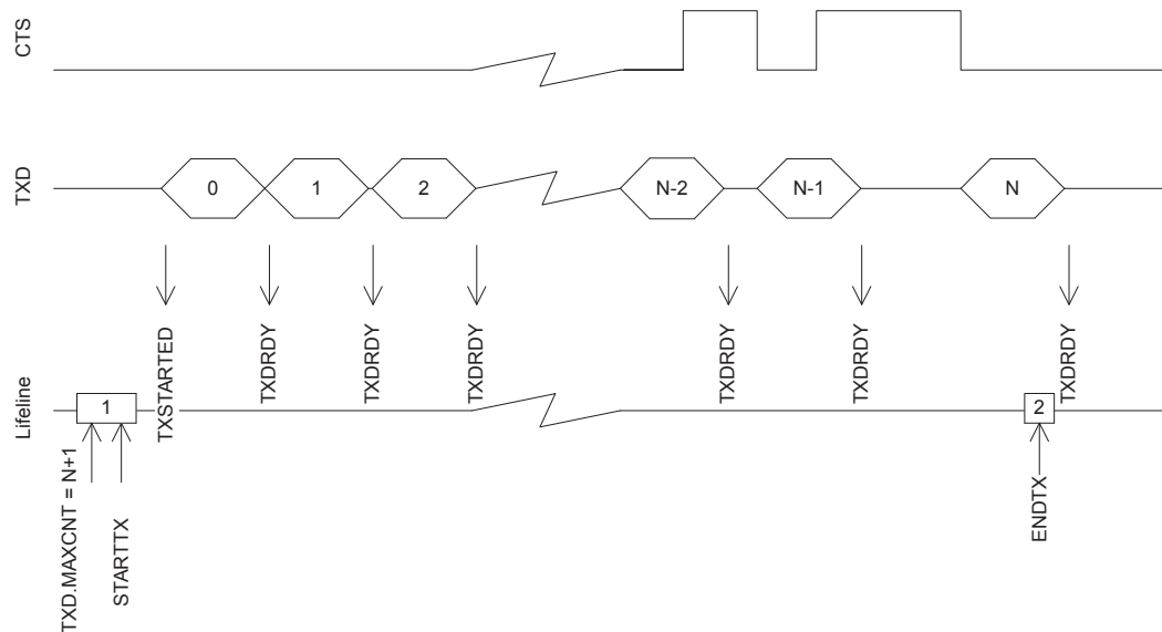
Figure 122: UARTe transmission
