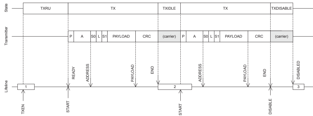
Figure 65: Transmission of multiple packets
