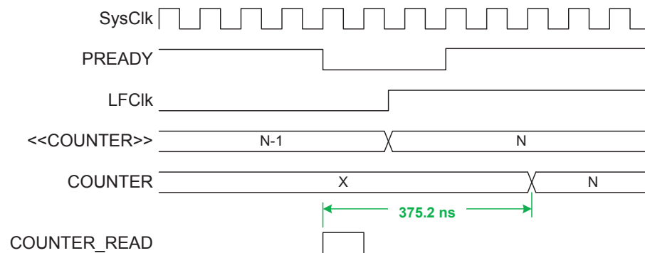
Figure 89: Timing diagram - COUNTER_READ
