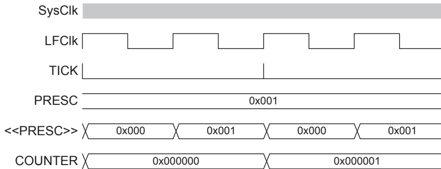
Figure 77: Timing diagram - COUNTER_PRESCALER_1
