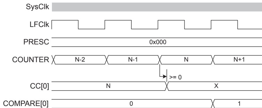
Figure 84: Timing diagram - COMPARE_N-1
