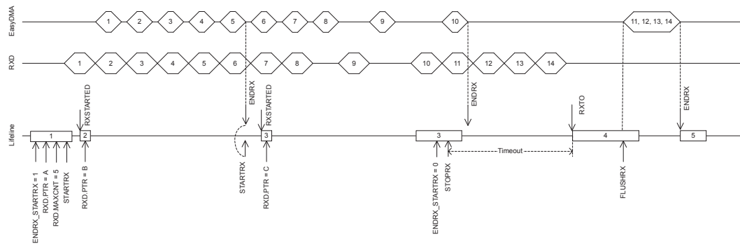
Figure 124: UARTE reception with forced stop via STOPRX
