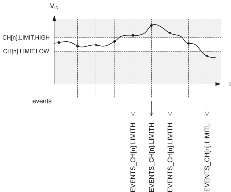
Figure 96: Example of limits monitoring on channel 'n'
