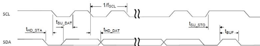
Figure 120: TWIS timing diagram, 1 byte transaction
