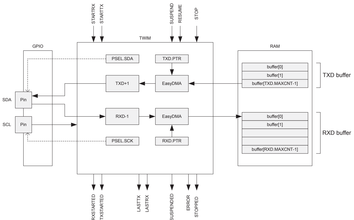
Figure 106: TWI master with EasyDMA
