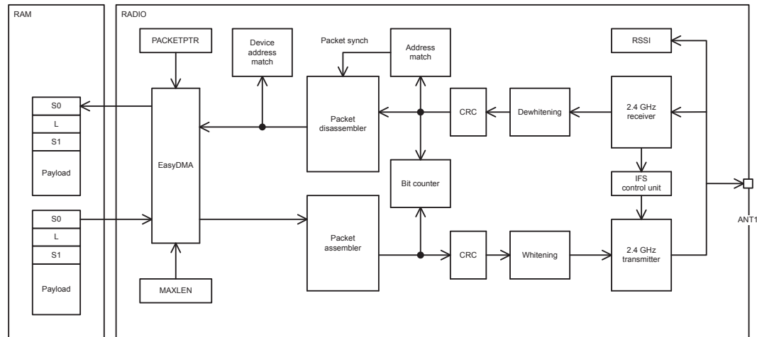
Figure 57: RADIO block diagram
