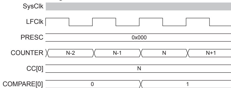
Figure 81: Timing diagram - COMPARE
