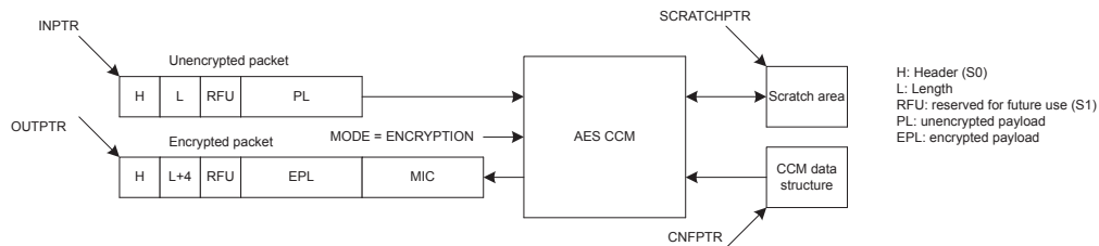
Figure 27: Encryption
