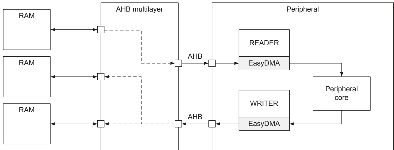
Figure 4: EasyDMA example
