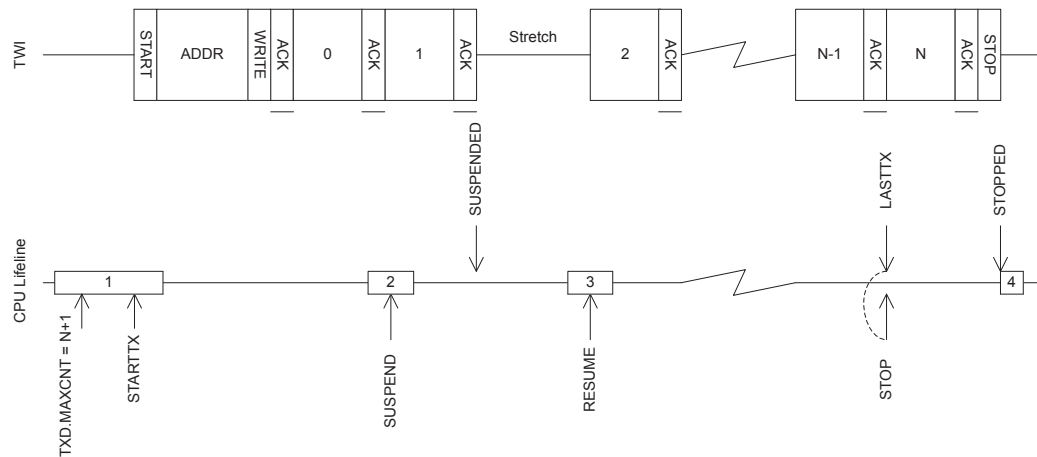
Figure 108: TWI master writing data to a slave
