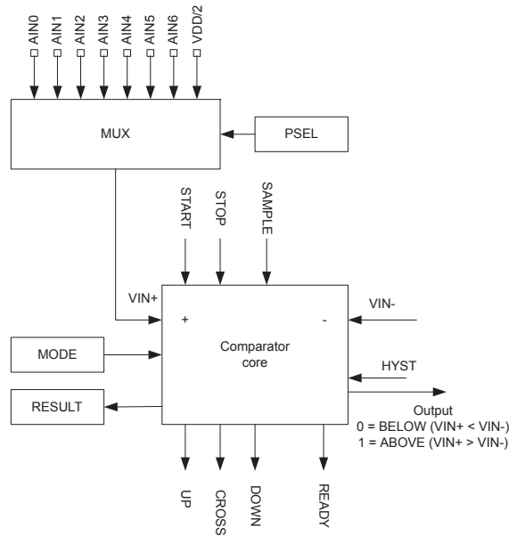
Figure 33: Comparator overview
