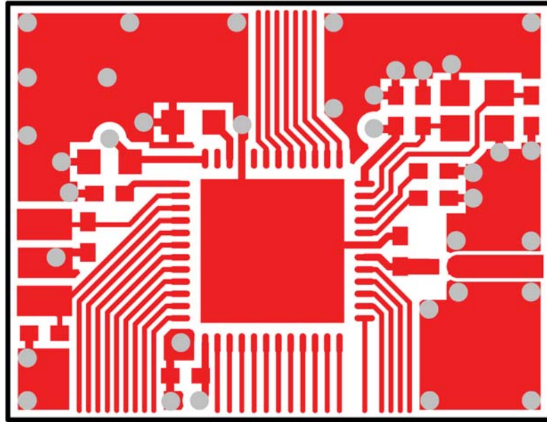
Figure 134: Top layer
