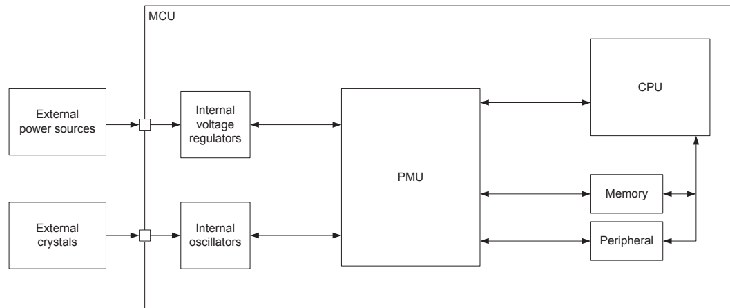
Figure 8: Power management unit
