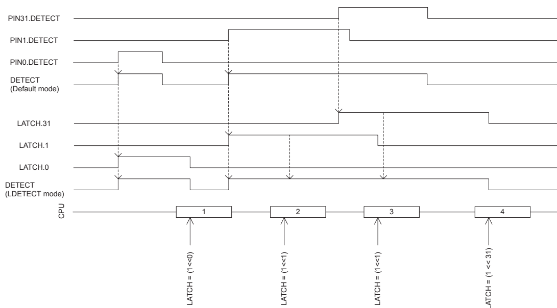
Figure 40: DETECT signal behavior
