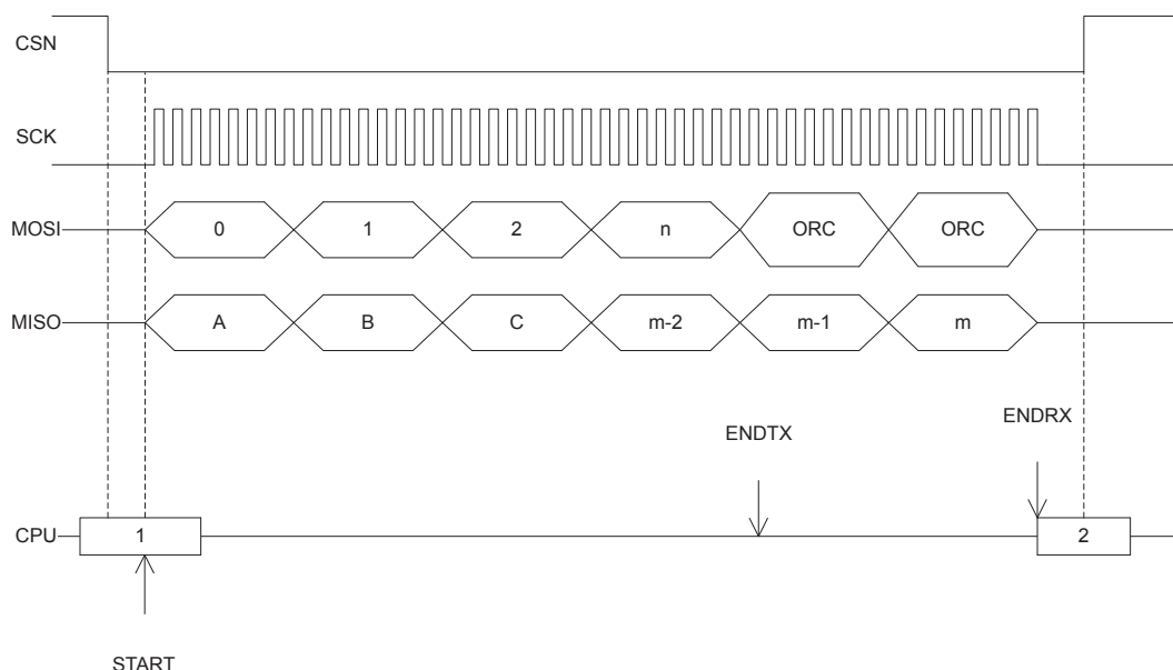
Figure 98: SPI master transaction
