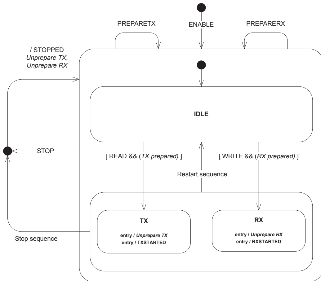
Figure 116: TWI slave state machine
