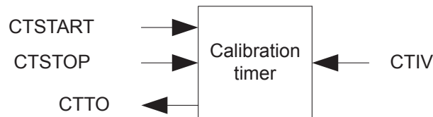
Figure 19: Calibration timer
