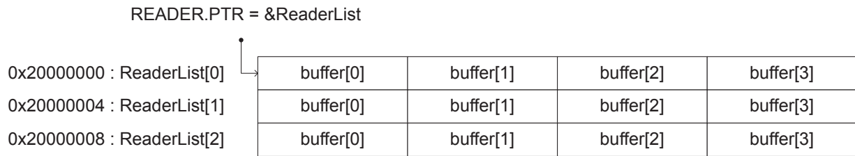
Figure 6: EasyDMA array list
