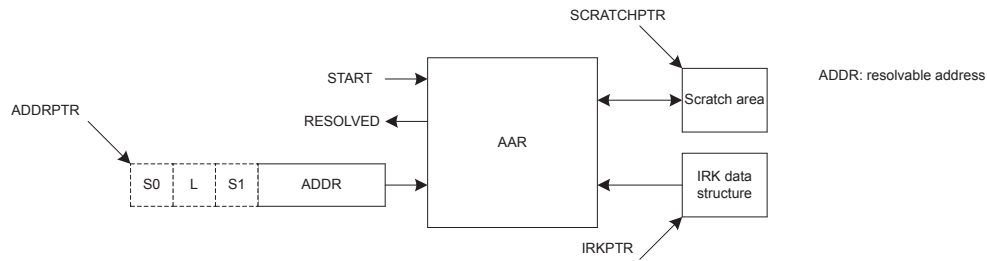
Figure 23: Address resolution with packet preloaded into RAM
