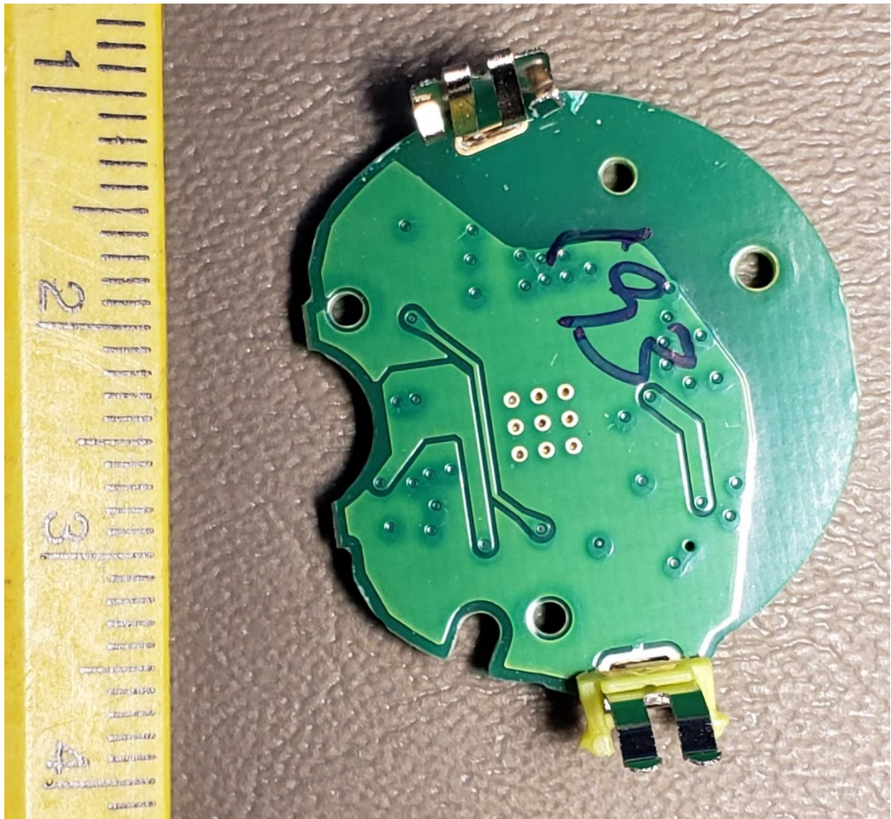
Circuit board bottom, contacts bent away
