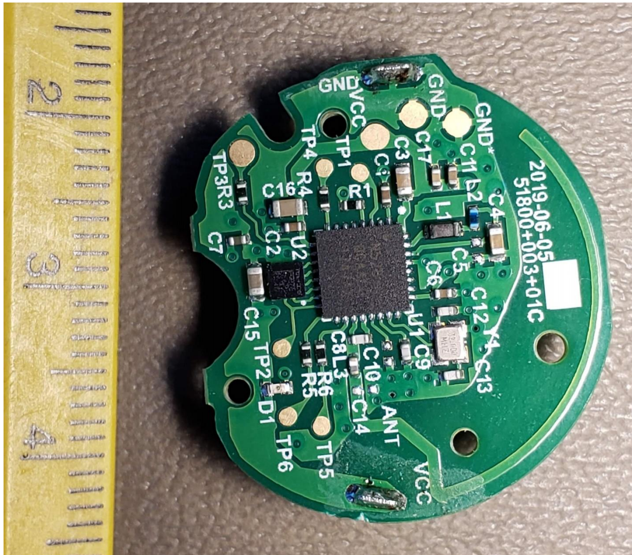
Circuit Board Top
