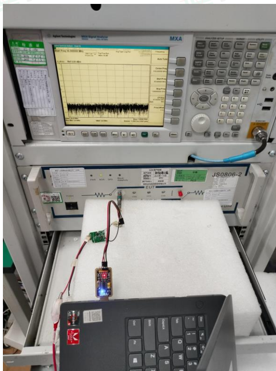
Test Setup Photo(s) of RF Conducted
