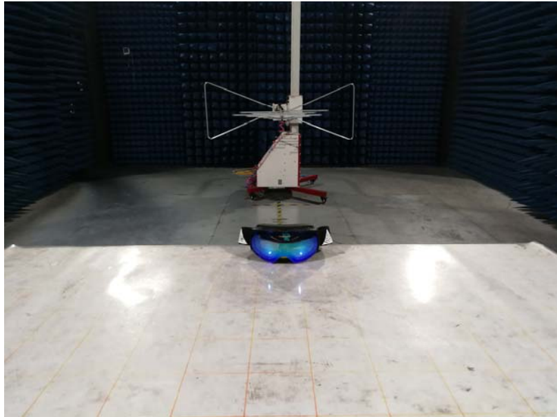
Radiated Emission
