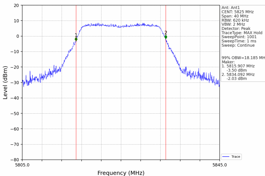
802.11a_HCH_5825MHz_Ant1_NTNV
