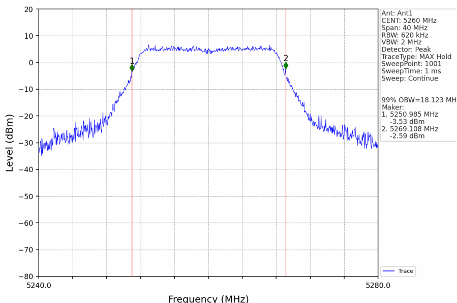
802.11a_LCH_5260MHz_Ant1_NTNV
