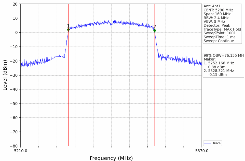
802.11ac(VHT80)_MCH_5290MHz_Ant1_NTNV
