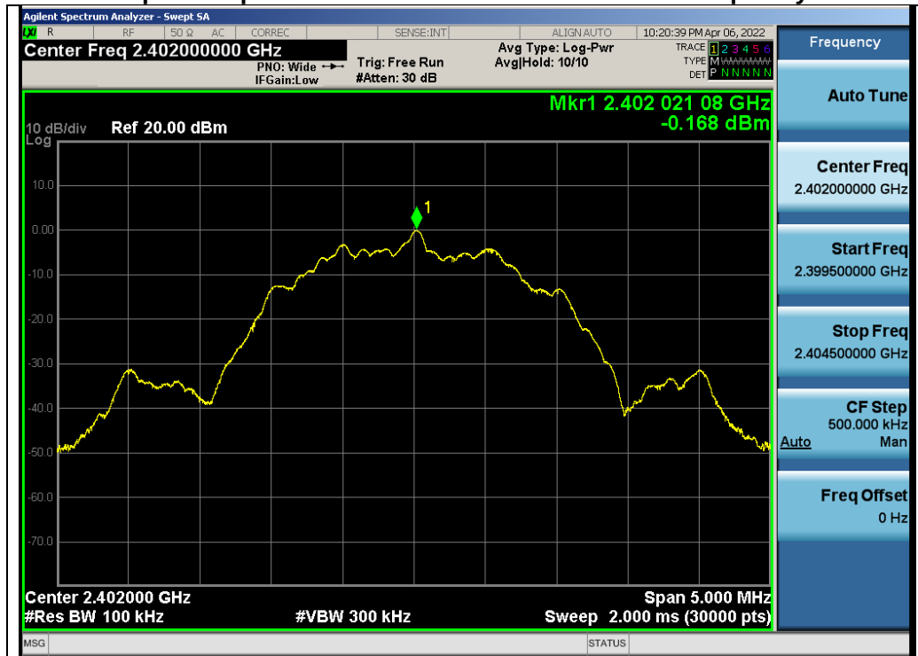
Test_Graph_LE2M_ANT1_2402_2Mbps_Reference Level
