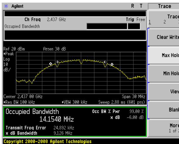
(802.11b) 6dB Bandwidth plot on channel 6
