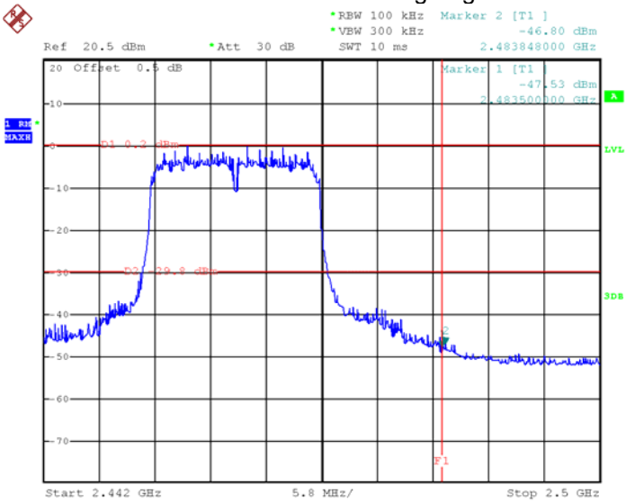
TX 11n HT20: Band edge-right side
