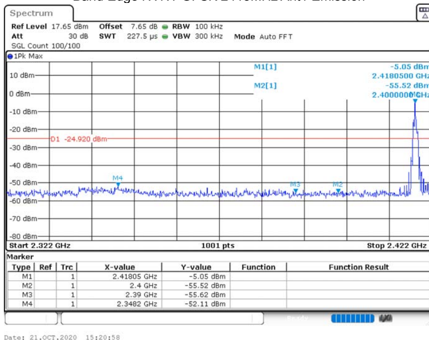
Band Edge NVNT GFSK 2418MHz Ant1 Emission
