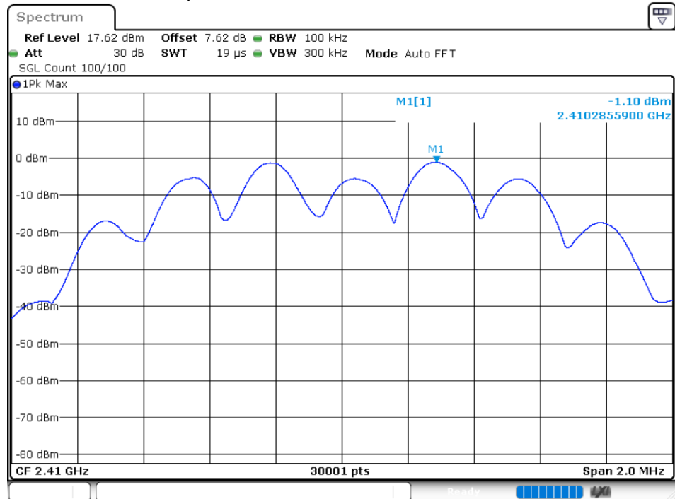
Tx. Spurious NVNT GFSK 2410MHz Ant1 Ref
