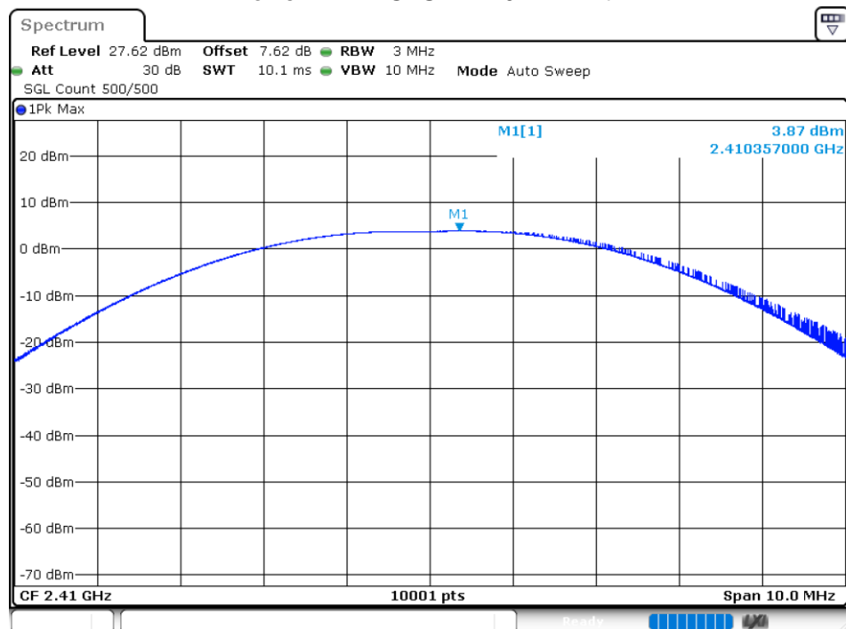
Power NVNT GFSK 2410MHz Ant1
