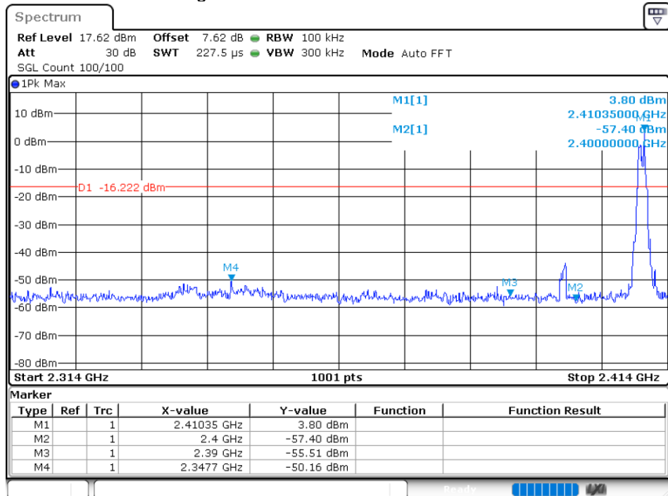
Band Edge NVNT GFSK 2410MHz Ant1 Emission
