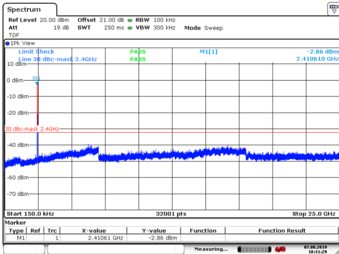
Figure 8.6-28: Conducted spurious emissions for 802.11n, MCS7, low channel
