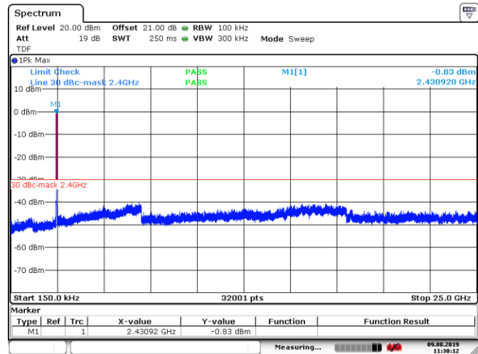
Figure 8.6-29: Conducted spurious emissions for 802.11n, MCS7, mid channel
