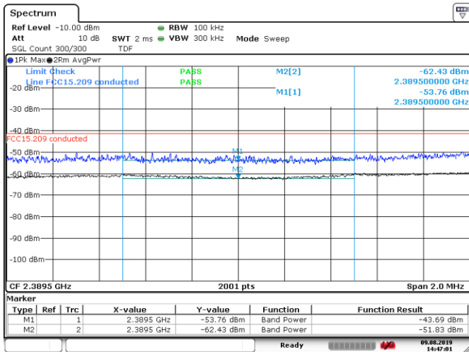
Figure 8.6-31: Conducted band edge emissions within restricted bands for 802.11b, 1 Mbps data rate, low channel
