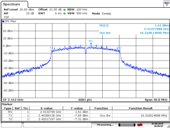
Figure 8.4-5: 99% bandwidth sample plot on 802.11g
