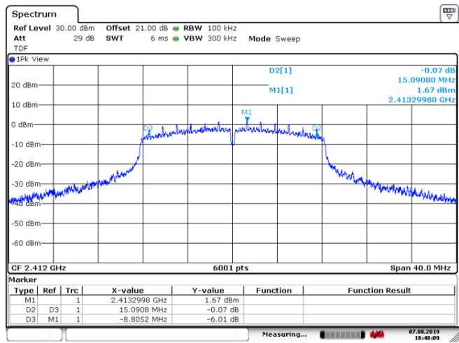
Figure 8.7-2: PSD sample plot on 802.11g
