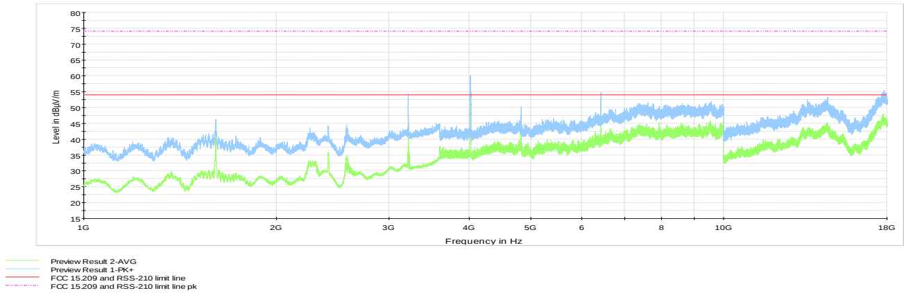
Figure 8.6-64: Cabinet radiated spurious emissions, low channel
