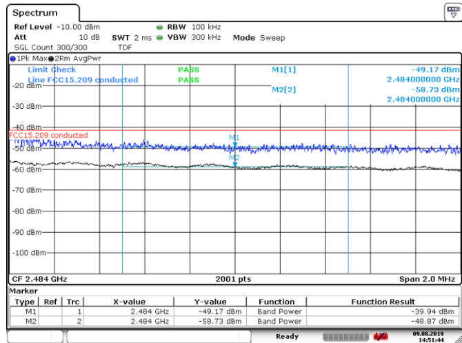
Figure 8.6-36: Conducted band edge emissions within restricted bands for 802.11g, 6 Mbps data rate, high channel
