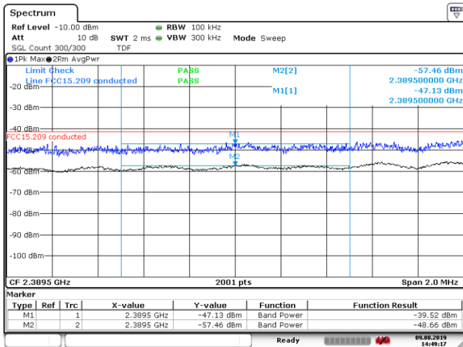
Figure 8.6-39: Conducted band edge emissions within restricted bands for 802.11n, MCS0, low channel
