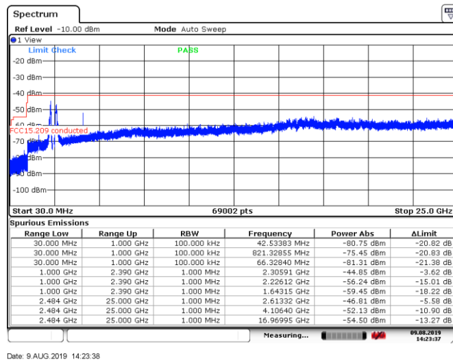
Figure 8.6-51: Conducted spurious emissions within restricted bands for 802.11g, 6 Mbps, high channel
