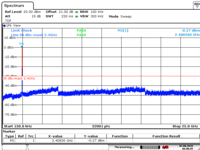
Figure 8.6-25: Conducted spurious emissions for 802.11n, MCS0, low channel
