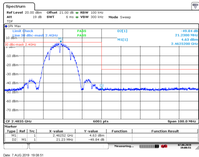
Figure 8.6-2: Conducted band edge emissions for 802.11b, 1 Mbps data rate, high channel
