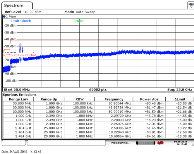
Figure 8.6-52: Conducted spurious emissions within restricted bands for 802.11g, 54 Mbps, low channel
