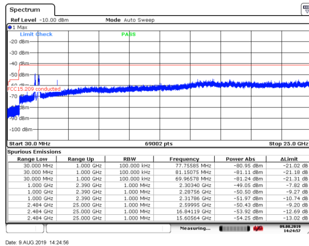
Figure 8.6-60: Conducted spurious emissions within restricted bands for 802.11n, MCS7, high channel
