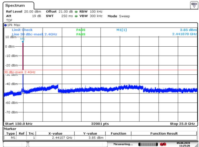
Figure 8.6-20: Conducted spurious emissions for 802.11g, 6 Mbps data rate, mid channel
