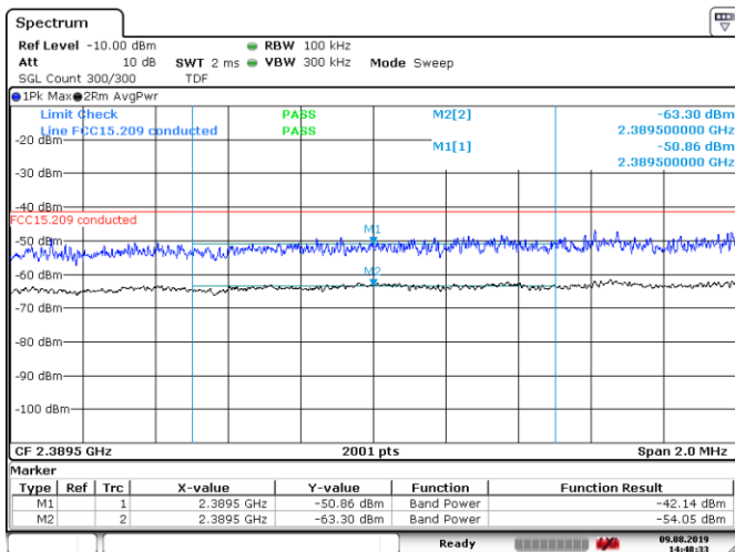
Figure 8.6-37: Conducted band edge emissions within restricted bands for 802.11g, 54 Mbps data rate, low channel
