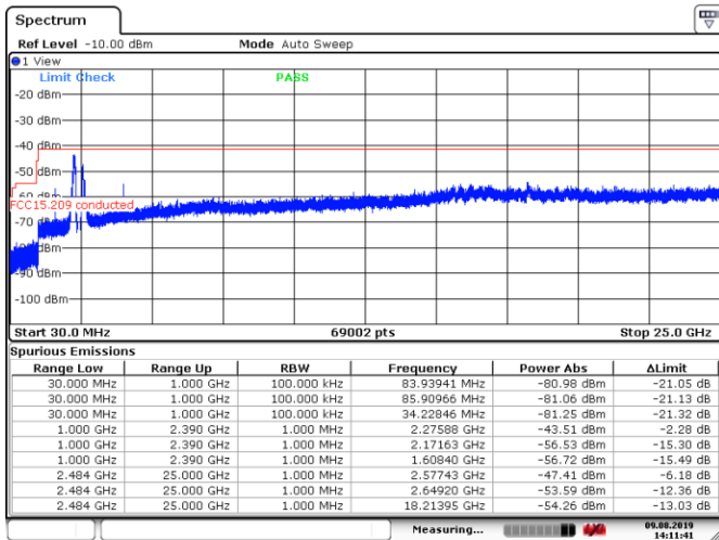
Figure 8.6-46: Conducted spurious emissions within restricted bands for 802.11b, 11 Mbps, low channel
