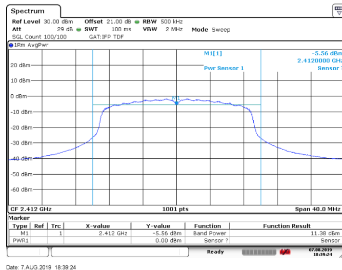
Figure 8.5-3: Output power sample plot on 802.11n
