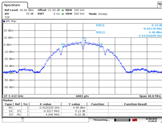
Figure 8.7-1: PSD sample plot on 802.11b
