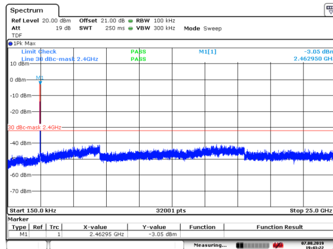
Figure 8.6-15: Conducted spurious emissions for 802.11b, 1 Mbps data rate, high channel
