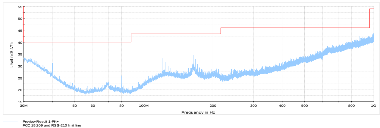
Figure 8.6-62: Cabinet radiated spurious emissions, mid channel
