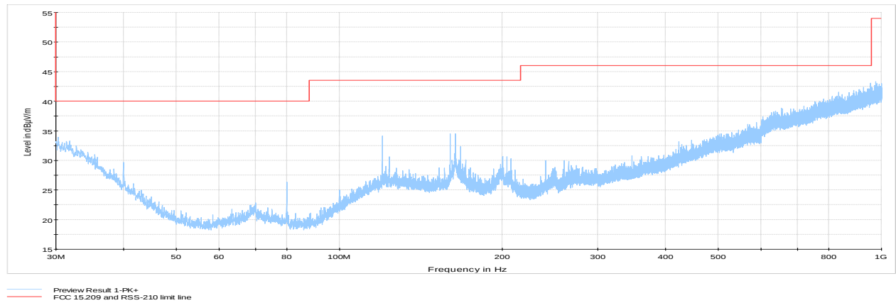
Figure 8.6-61: Cabinet radiated spurious emissions, low channel
