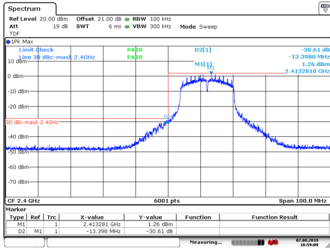
Figure 8.6-5: Conducted band edge emissions for 802.11g, 6 Mbps data rate, low channel
