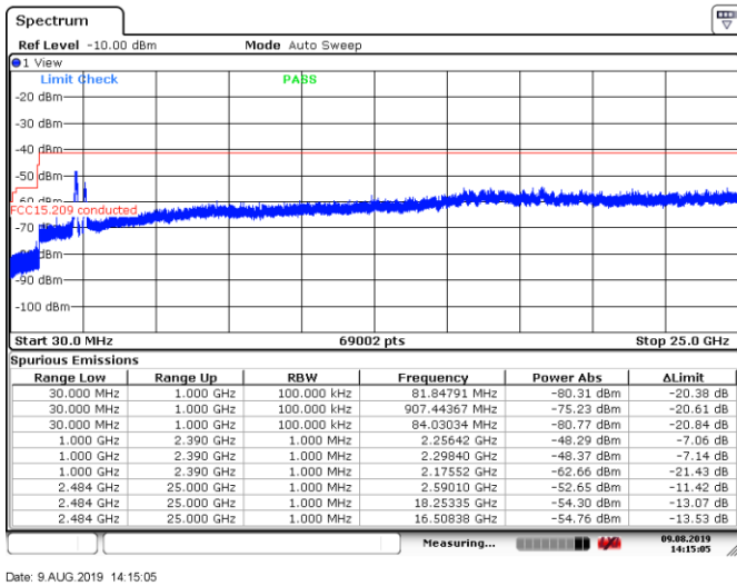
Figure 8.6-58: Conducted spurious emissions within restricted bands for 802.11n, MCS7, low channel
