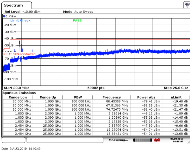
Figure 8.6-43: Conducted spurious emissions within restricted bands for 802.11b, 1Mbps, low channel
