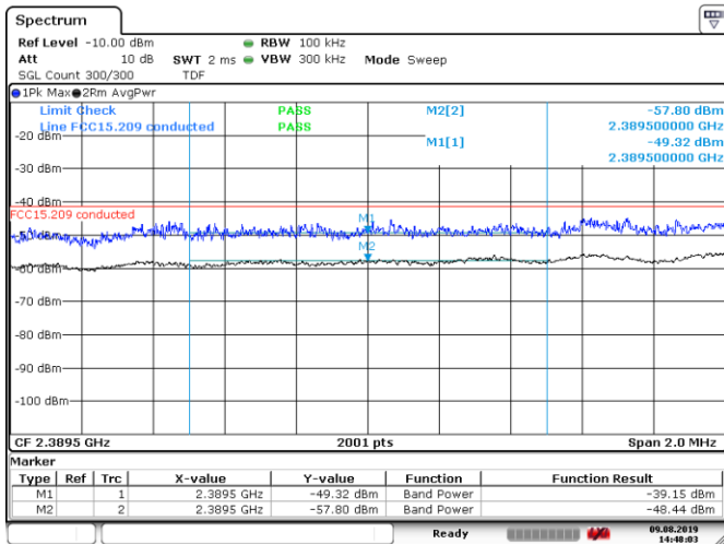
Figure 8.6-35: Conducted band edge emissions within restricted bands for 802.11g, 6 Mbps data rate, low channel
