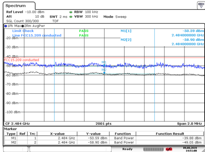
Figure 8.6-40: Conducted band edge emissions within restricted bands for 802.11n, MCS0, high channel
