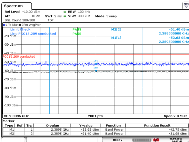
Figure 8.6-33: Conducted band edge emissions within restricted bands for 802.11b, 11 Mbps data rate, low channel
