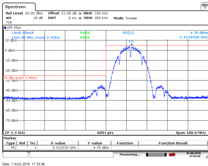
Figure 8.6-1: Conducted band edge emissions for 802.11b, 1 Mbps data rate, low channel
