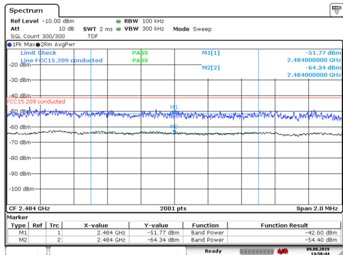
Figure 8.6-42: Conducted band edge emissions within restricted bands for 802.11n, MCS7, high channel
