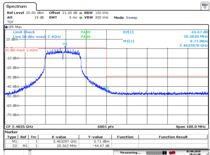
Figure 8.6-8: Conducted band edge emissions for 802.11g, 54 Mbps data rate, high channel
