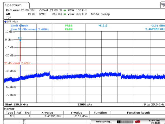
Figure 8.6-24: Conducted spurious emissions for 802.11g, 54 Mbps data rate, high channel
