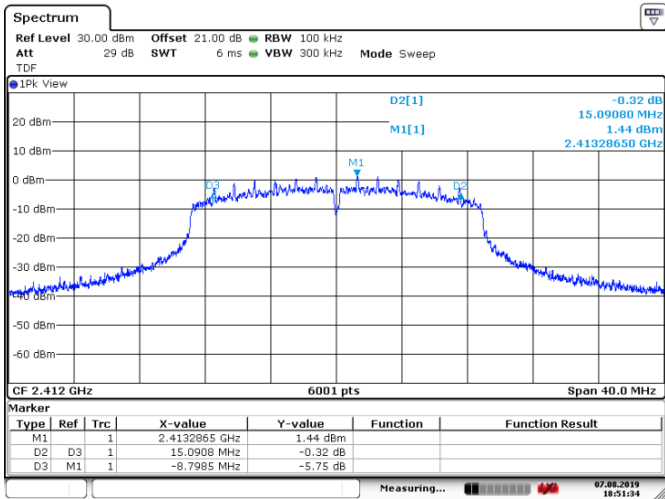
Figure 8.4-3: 6 dB bandwidth sample plot on 802.11n
