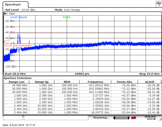
Figure 8.6-50: Conducted spurious emissions within restricted bands for 802.11g, 6 Mbps, mid channel
