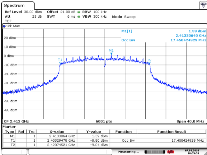
Figure 8.4-6: 99% bandwidth sample plot on 802.11n
