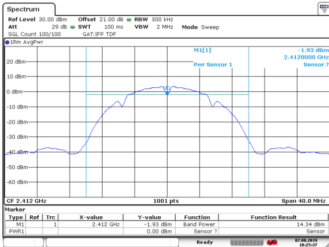
Figure 8.5-1: Output power sample plot on 802.11b
