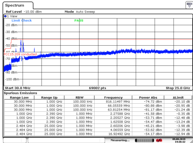
Figure 8.6-56: Conducted spurious emissions within restricted bands for 802.11n, MCS0, mid channel
