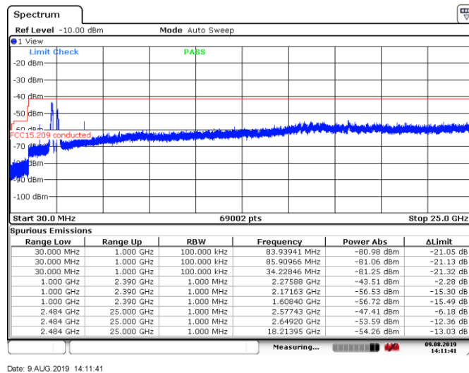
Figure 8.6-48: Conducted spurious emissions within restricted bands for 802.11b, 11 Mbps, high channel
