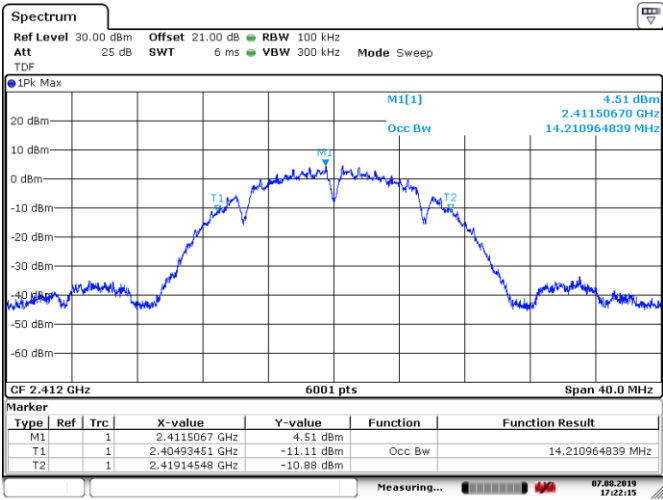
Figure 8.4-4: 99% bandwidth sample plot on 802.11b
