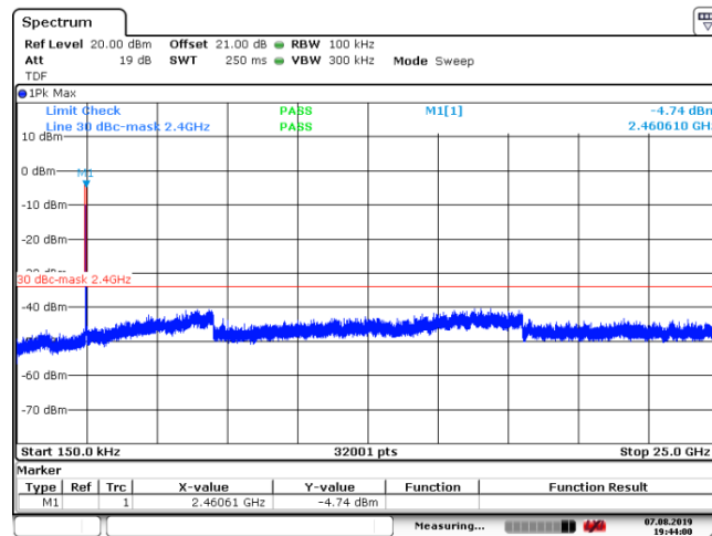
Figure 8.6-18: Conducted spurious emissions for 802.11b, 11 Mbps data rate, high channel
