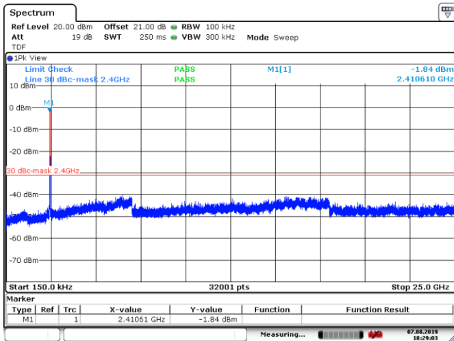
Figure 8.6-19: Conducted spurious emissions for 802.11g, 6 Mbps data rate, low channel
