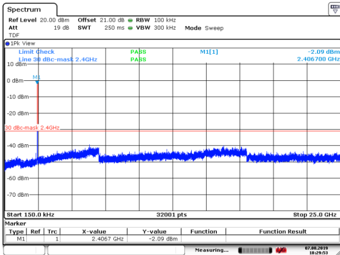
Figure 8.6-22: Conducted spurious emissions for 802.11g, 54 Mbps data rate, low channel
