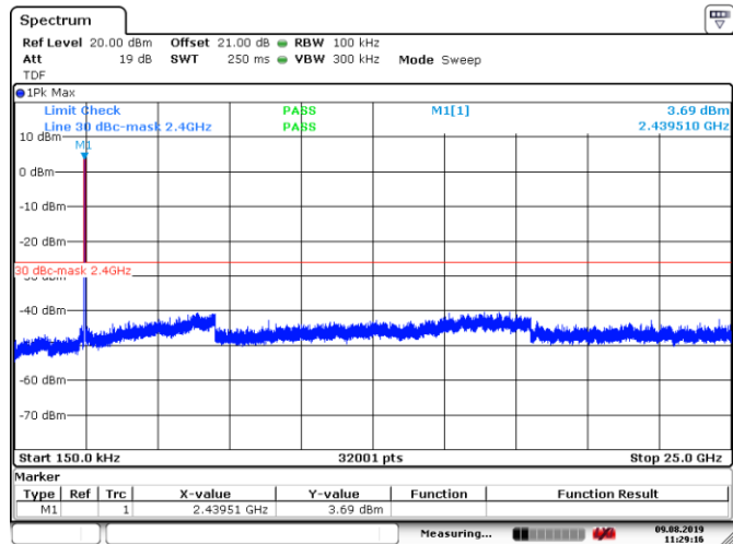
Figure 8.6-14: Conducted spurious emissions for 802.11b, 1 Mbps data rate, mid channel
