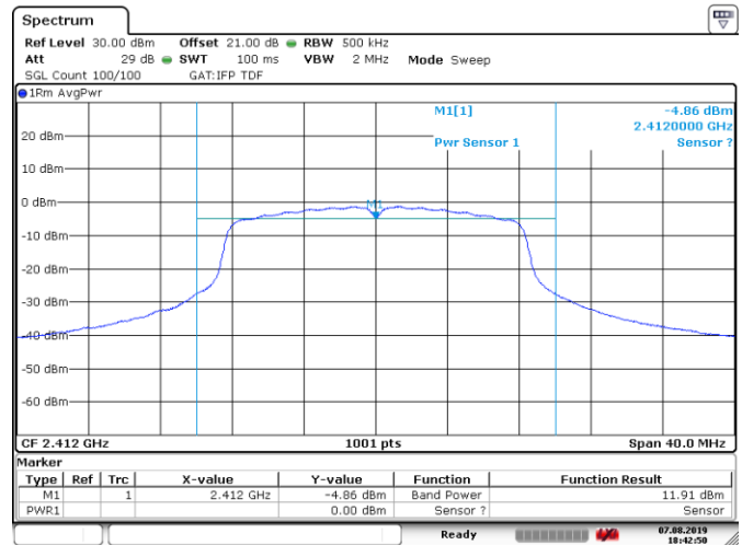
Figure 8.5-2: Output power sample plot on 802.11g
