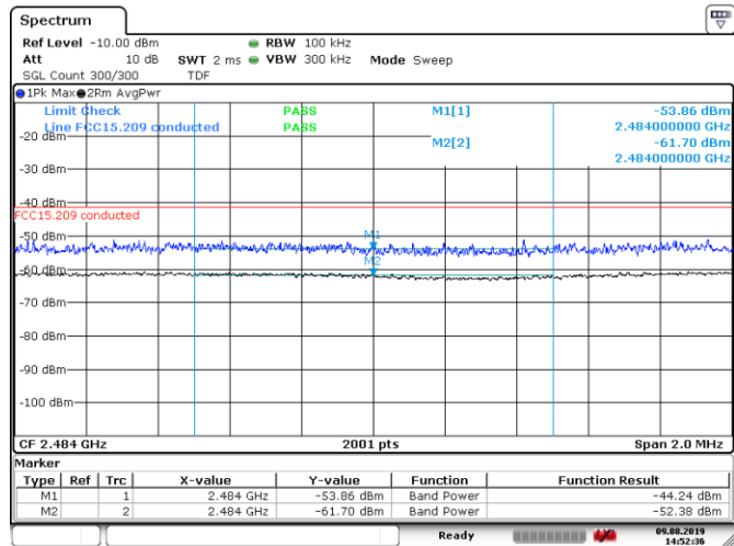
Figure 8.6-32: Conducted band edge emissions within restricted bands for 802.11b, 1 Mbps data rate, high channel
