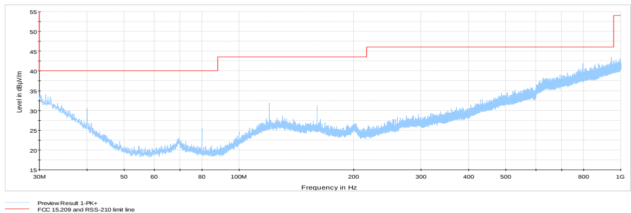
Figure 8.6-63: Cabinet radiated spurious emissions, high channel
