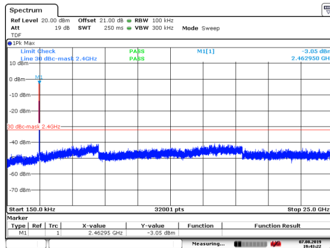
Figure 8.6-27: Conducted spurious emissions for 802.11n, MCS0, high channel
