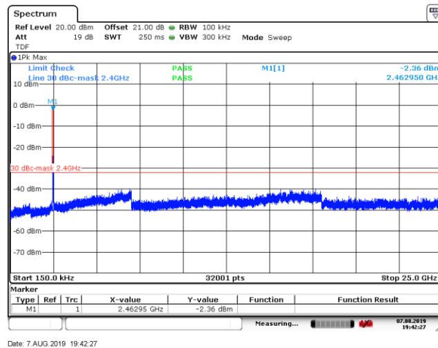
Figure 8.6-21: Conducted spurious emissions for 802.11g, 6 Mbps data rate, high channel
