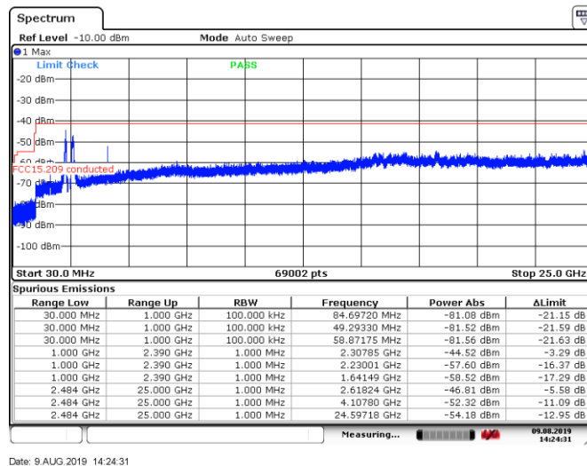
Figure 8.6-57: Conducted spurious emissions within restricted bands for 802.11n, MCS0, high channel
