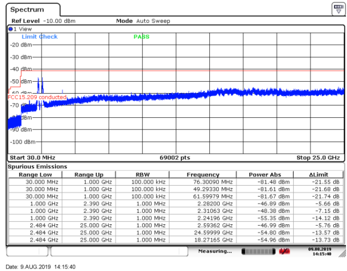
Figure 8.6-59: Conducted spurious emissions within restricted bands for 802.11n, MCS7, mid channel
