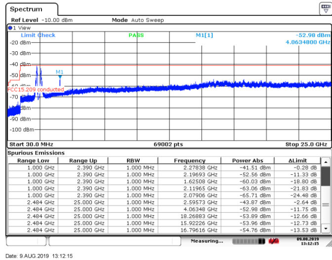
Figure 8.6-44: Conducted spurious emissions within restricted bands for 802.11b, 1Mbps, mid channel
