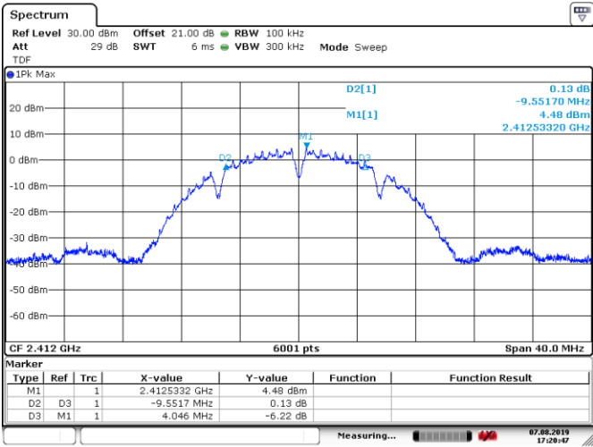
Figure 8.4-1: 6 dB bandwidth sample plot on 802.11b
