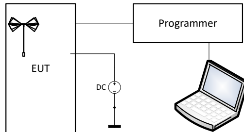
Figure 3.6-1: Setup diagram
