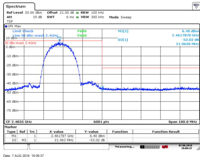
Figure 8.6-4: Conducted band edge emissions for 802.11b, 11 Mbps data rate, high channel
