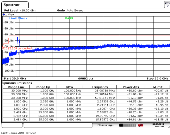
Figure 8.6-49: Conducted spurious emissions within restricted bands for 802.11g, 6 Mbps, low channel
