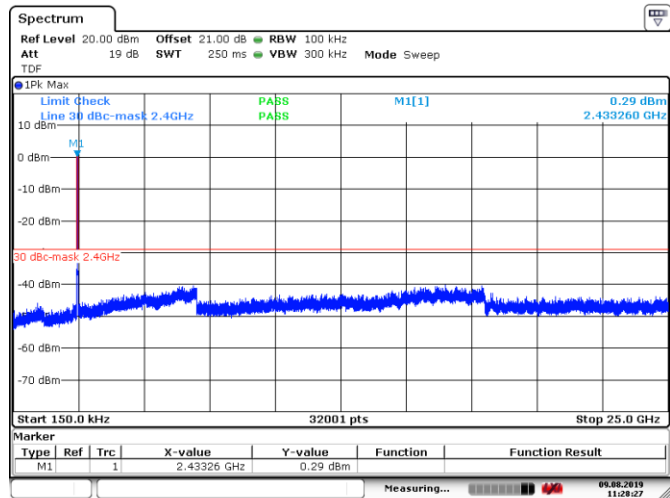
Figure 8.6-23: Conducted spurious emissions for 802.11g, 54 Mbps data rate, mid channel
