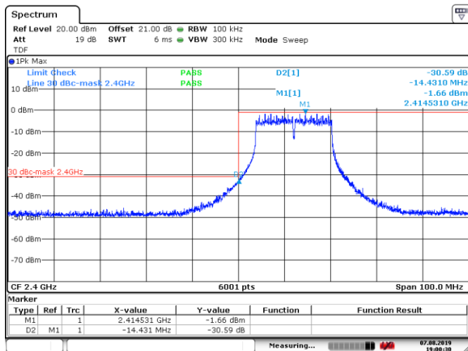
Figure 8.6-7: Conducted band edge emissions for 802.11g, 54 Mbps data rate, low channel
