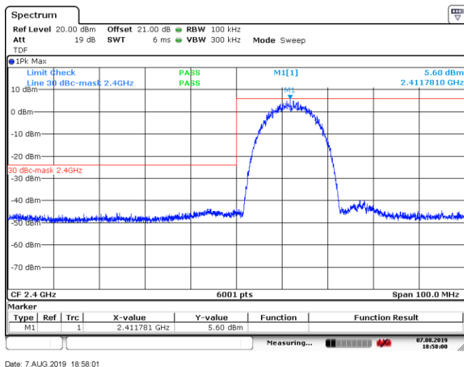
Figure 8.6-3: Conducted band edge emissions for 802.11b, 11 Mbps data rate, low channel
