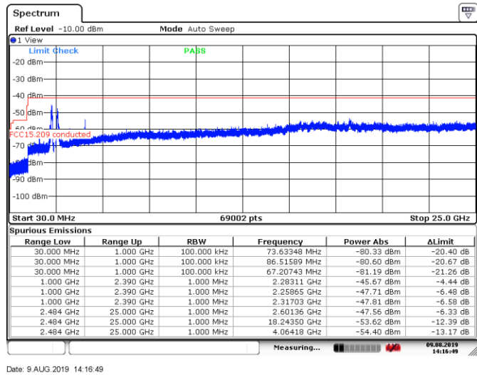
Figure 8.6-53: Conducted spurious emissions within restricted bands for 802.11g, 54 Mbps, mid channel
