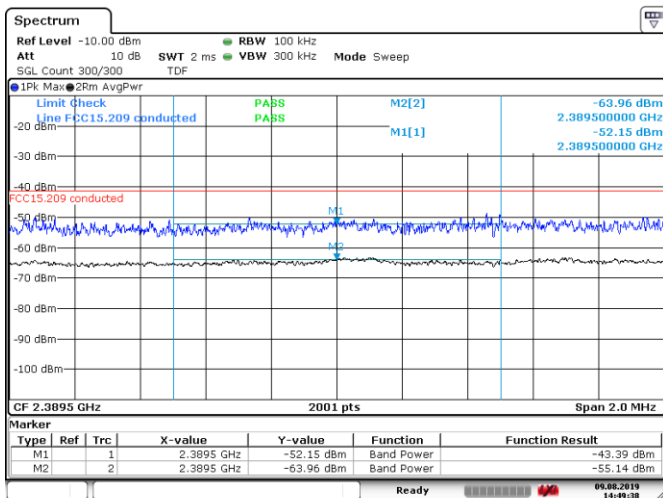
Figure 8.6-41: Conducted band edge emissions within restricted bands for 802.11n, MCS7, low channel
