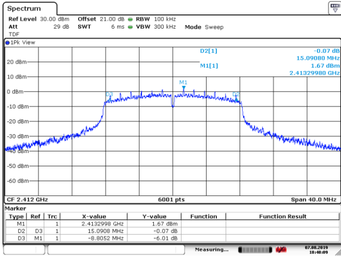
Figure 8.4-2: 6 dB bandwidth sample plot on 802.11g
