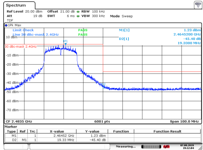
Figure 8.6-6: Conducted band edge emissions for 802.11g, 6 Mbps data rate, high channel
