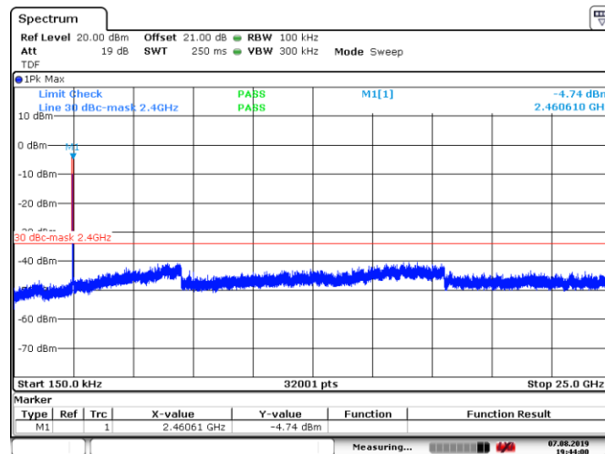
Figure 8.6-30: Conducted spurious emissions for 802.11n, MCS7, high channel
