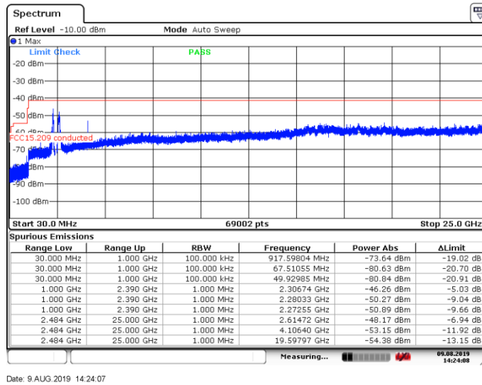
Figure 8.6-54: Conducted spurious emissions within restricted bands for 802.11g, 54 Mbps, high channel
