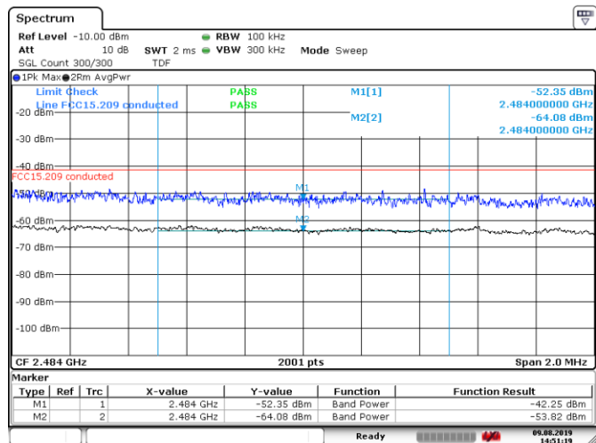
Figure 8.6-38: Conducted band edge emissions within restricted bands for 802.11g, 54 Mbps data rate, high channel
