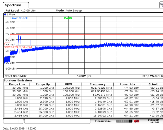
Figure 8.6-45: Conducted spurious emissions within restricted bands for 802.11b, 1Mbps, high channel
