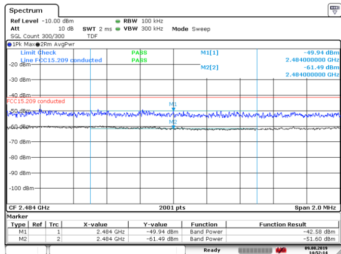
Figure 8.6-34: Conducted band edge emissions within restricted bands for 802.11b, 11 Mbps data rate, high channel
