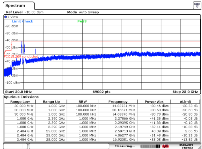
Figure 8.6-47: Conducted spurious emissions within restricted bands for 802.11b, 11 Mbps, mid channel
