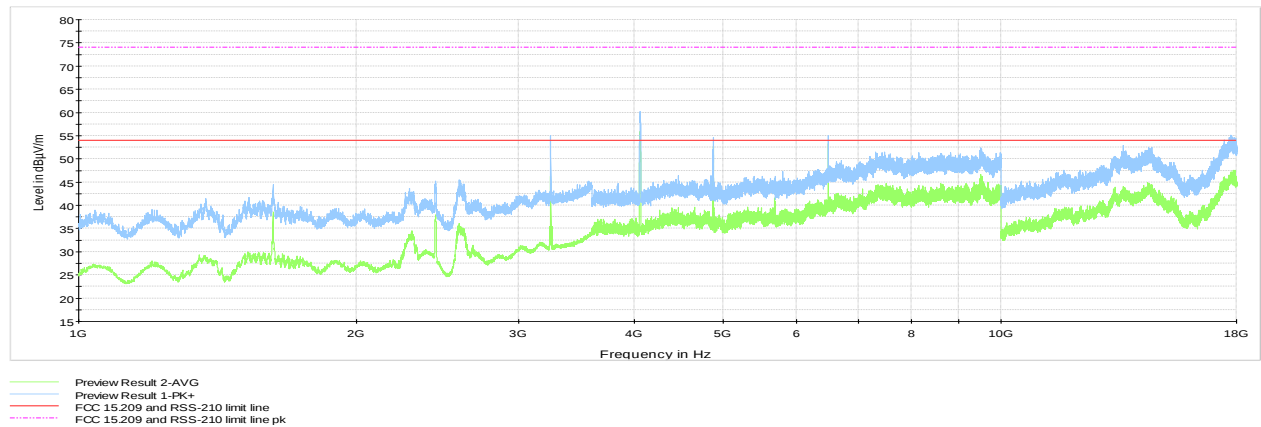
Figure 8.6-65: Cabinet radiated spurious emissions, mid channel
