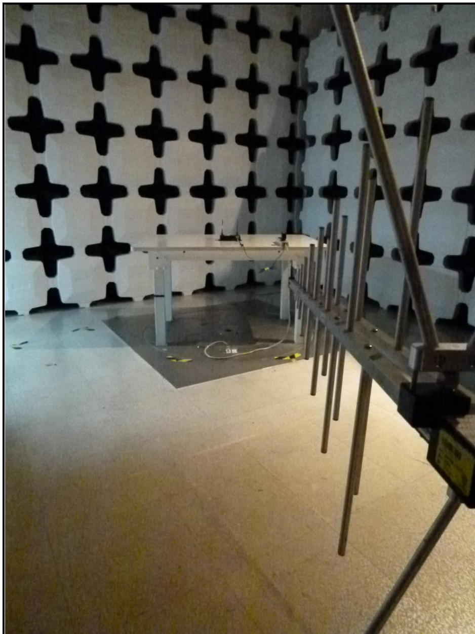
Antenna 1
