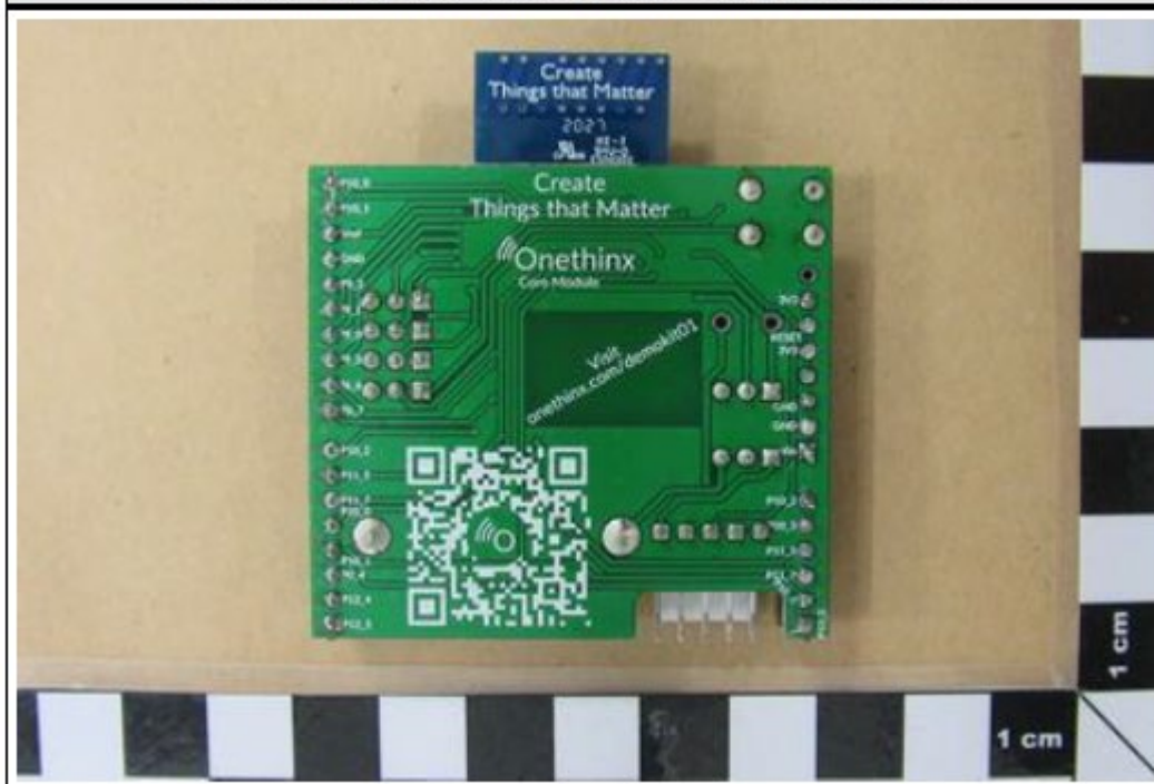
Evaluation board with LoRa module Bottom View
