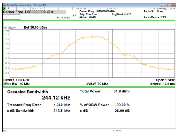
EGPRS_1900_Middle_26BW and 99%
