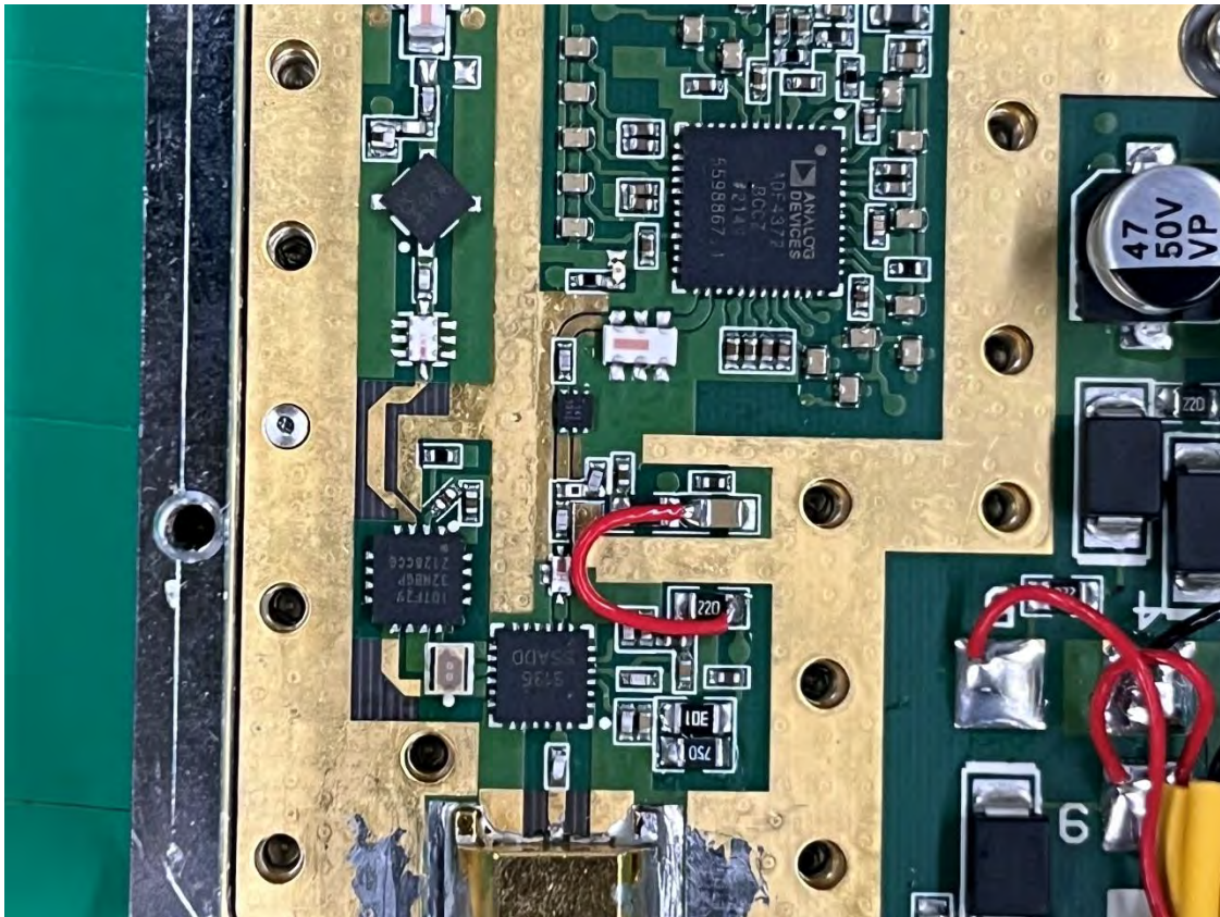
(32) EUT Photo
