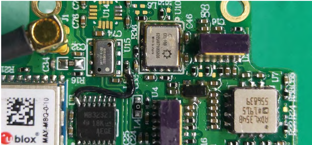
(43) EUT Photo
