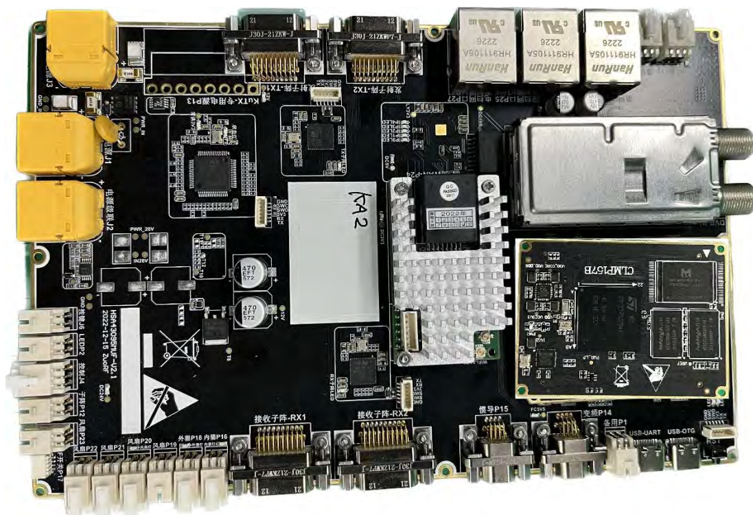
(7) EUT Photo
