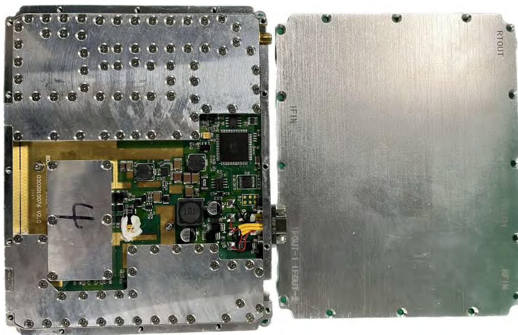
(26) EUT Photo
