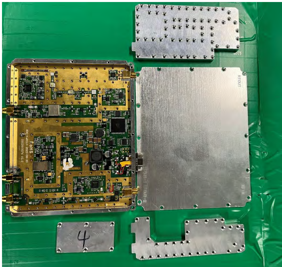
(28) EUT Photo
