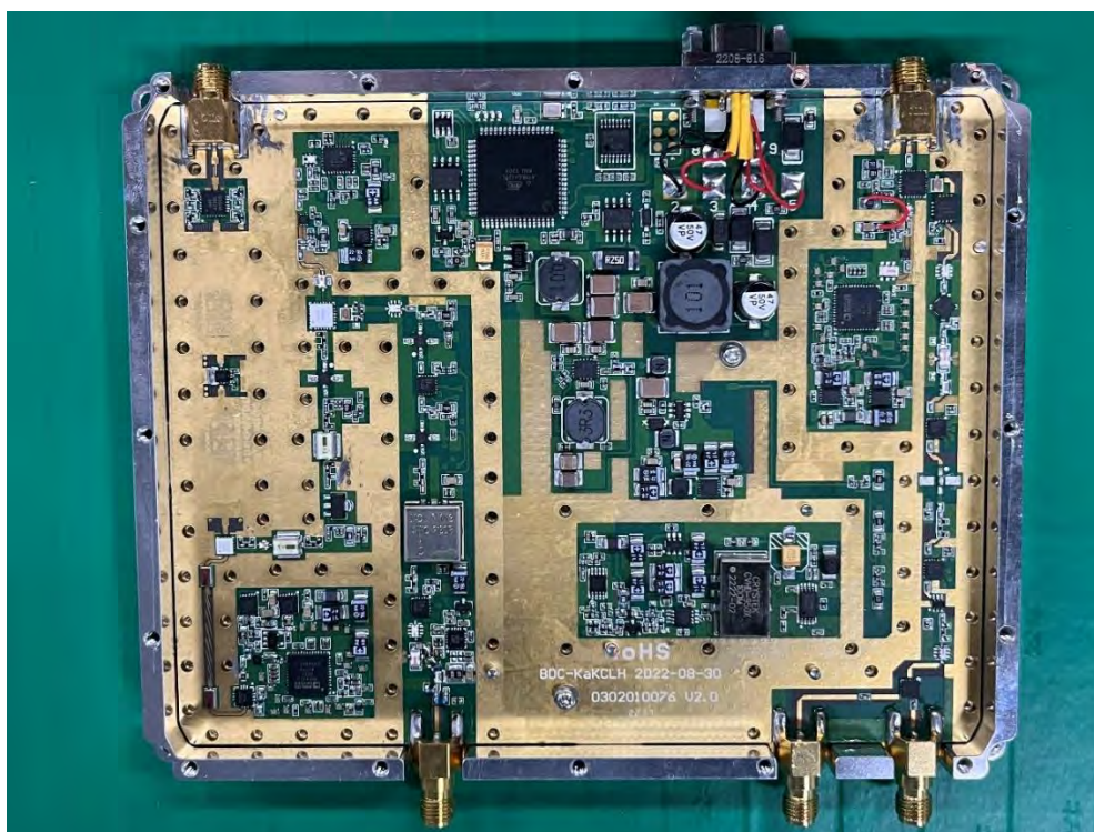
(28) EUT Photo
